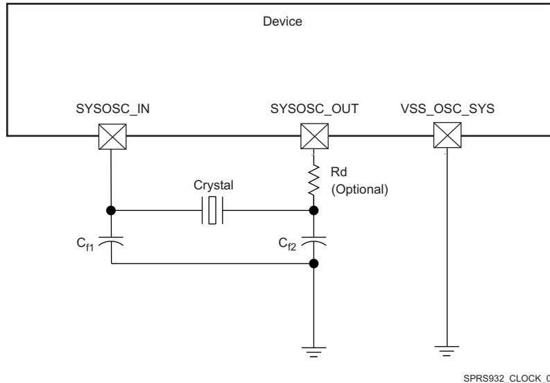
Figure 5-9. Crystal Implementation (1)
