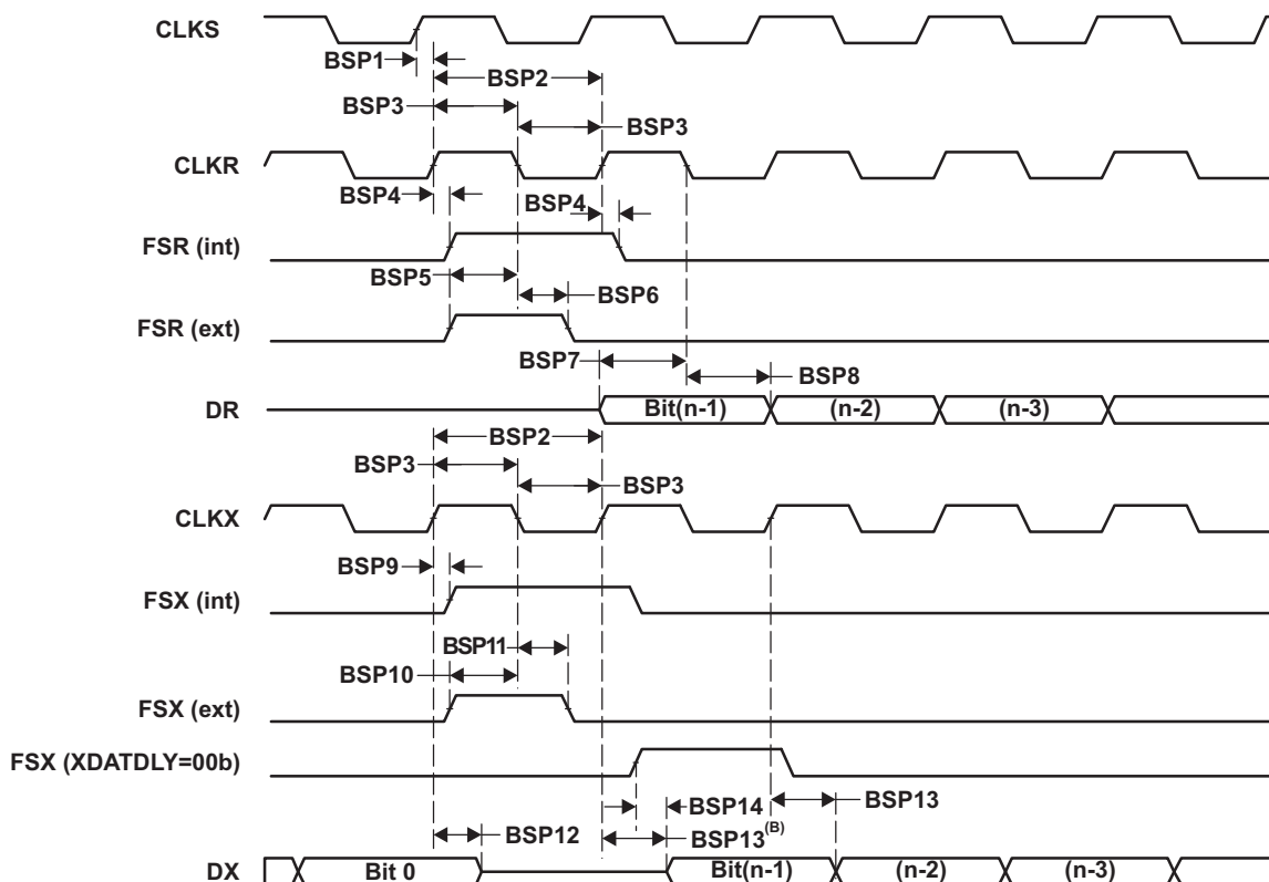
图 5-51. McBSP Timing
