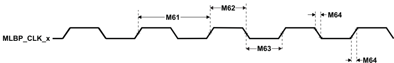
图 5-55. MLB_CLKP/N Timing (1)
