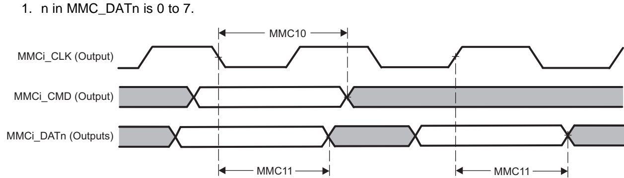
图 5-61. MMC1_CMD and MMC1_DATn Output Timing—HSPE=0 – DDR Mode (1)
