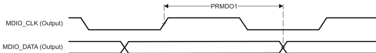
图 5-73. PRU-ICSS MDIO_DATA Timing – Output Mode
