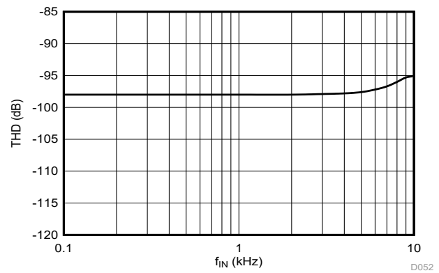
图 6-27. Total Harmonic Distortion vs Input Signal Frequency
