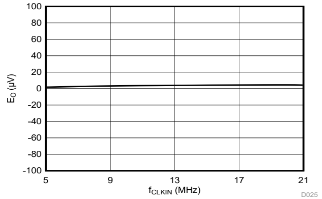
图 6-13. Offset Error vs Clock Frequency
