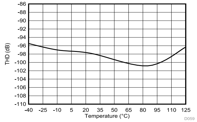
图 6-25. Total Harmonic Distortion vs Temperature
