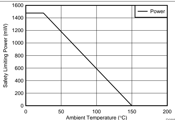
Figure 6. Thermal Derating Curve for Limiting Power for DWW Package
