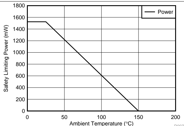
Figure 5. Thermal Derating Curve for Limiting Power for DW Package
