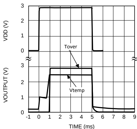
Figure 9. Start-Up Response
