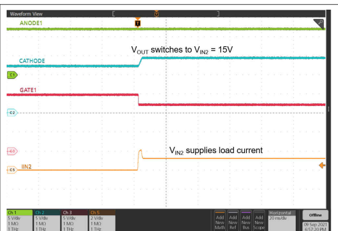
图 9-14. ORing V_{IN1} to V_{IN2} Switch Over
