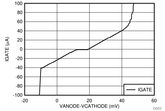
图 6-16. Gate Current vs Forward Voltage Drop
