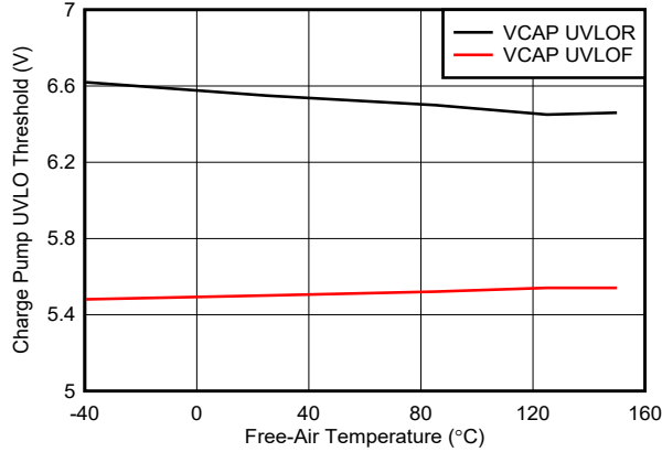
图 6-13. Charge Pump UVLO Threshold vs Temperature
