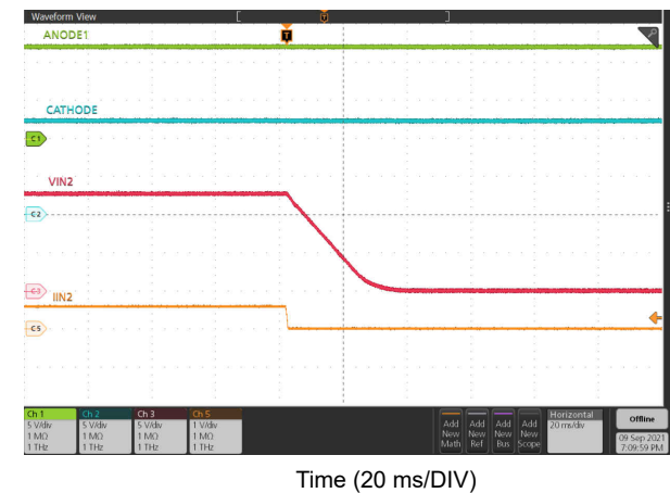
图 9-18. ORing - V_{IN2} Failure and Switch Over to V_{IN1}
