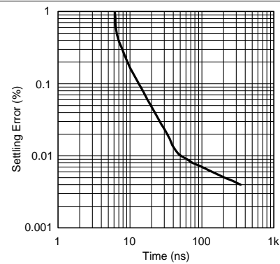
R_L = 100\ \Omega
