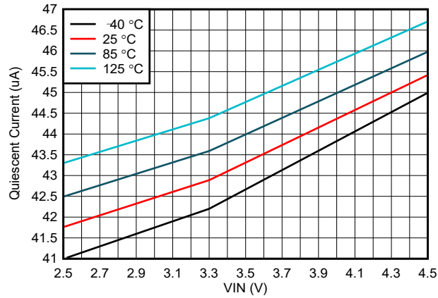
图 6-1. Quiescent Current vs Input Voltage
