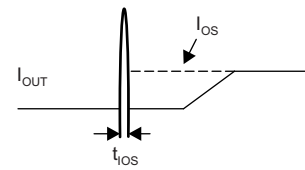
Figure 12. Output Short Circuit Parameters
