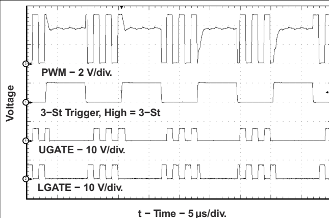
图 6-19. Normal and Three-State Operation ENTER/EXIT Conditions
