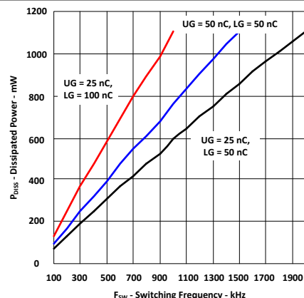
图 6-15. Driver Dissipated Power vs Switching Frequency
