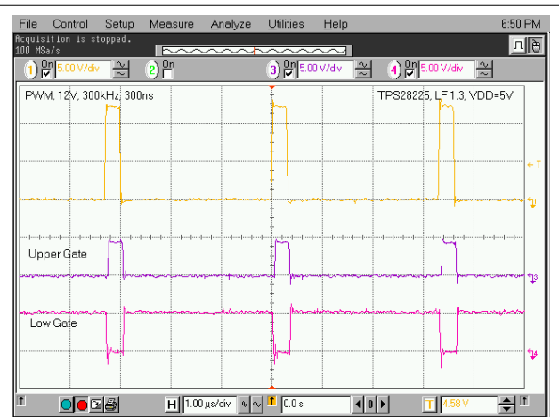
图 7-5. 12-V PWM Pulse at V_{DD} = 5 V
