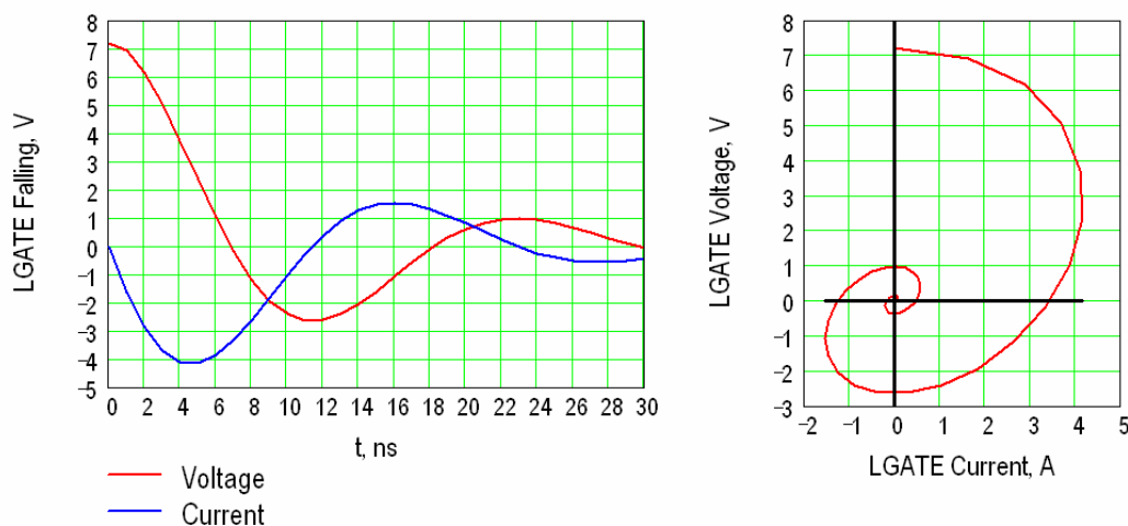
图 8-6. LGATE Turning Off Voltage and Sink Current vs Time (Related Switching Diagram [Right])
