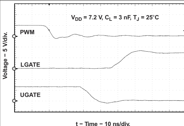
图 6-17. PWM Input Falling Switching Waveforms
