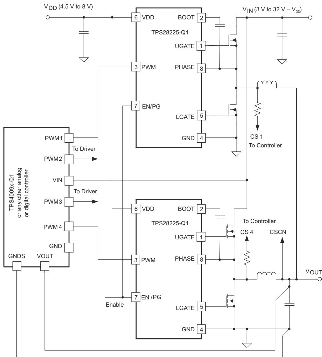
图 8-2. Multi-Phase Synchronous Buck Converter
