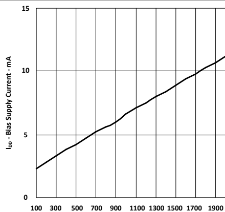
图 6-14. Bias Supply Current vs Switching Frequency
