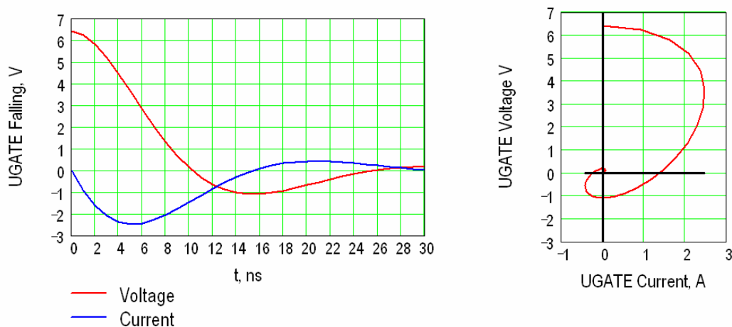
图 8-7. UGATE Turning Off Voltage and Sink Current vs Time (Related Switching Diagram [Right])
