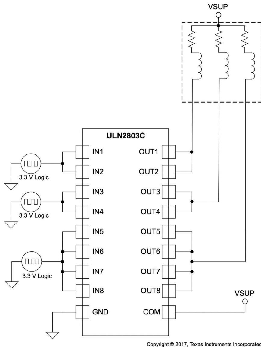
图 8-1. ULN2803C as Inductive Load Driver
