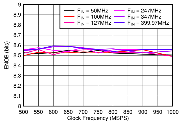
图 5-28. ENOB vs Sample Rate
