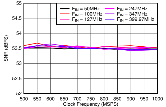
图 5-26. SNR vs Sample Rate
