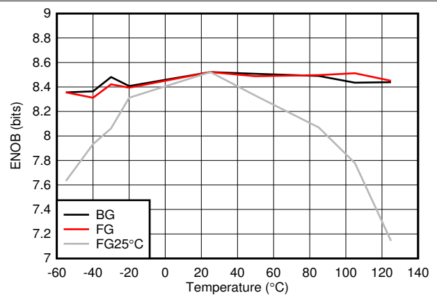
图 5-42. ENOB vs Temperature and Calibration Mode
