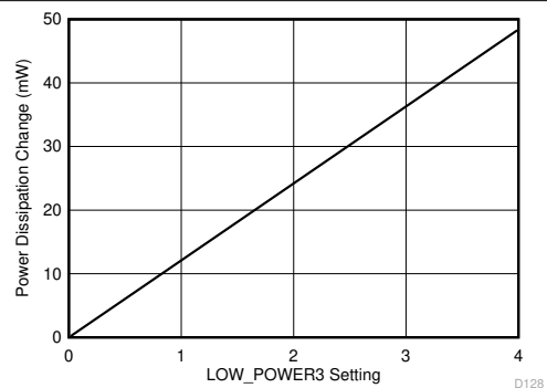
图 6-13. Power Dissipation Change vs LOW_POWER3 register setting
