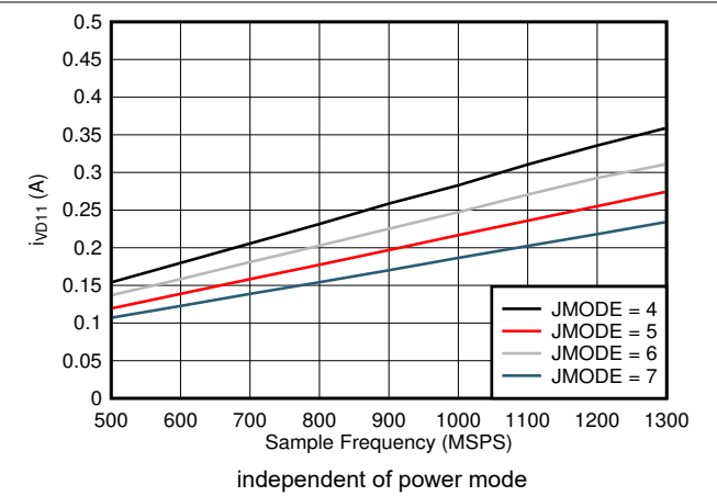
图 5-98. Dual Channel, I_{VD11} vs FS and JMODE 4 - 7
