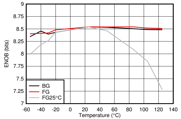
图 5-38. ENOB vs Temperature and Calibration Mode
