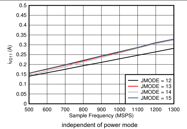
图 5-100. Dual Channel, I_{VD11} vs FS and JMODE 12 - 15
