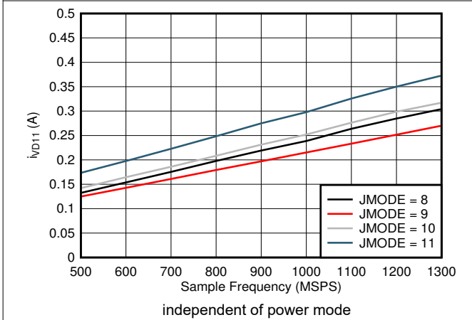
图 5-99. Dual Channel, I_{VD11} vs FS and JMODE 8 - 11
