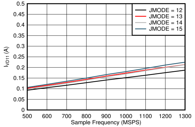
图 5-110. Single Channel, I_{VD11} vs FS and JMODE 12 - 15
