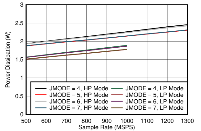
图 5-82. Quad Channel, Power Dissipation vs FS for JMODES 4 - 7
