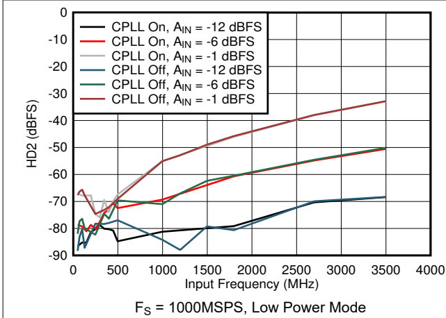
图 5-79. HD2 vs Input Frequency, CPLL and Input Amplitude
