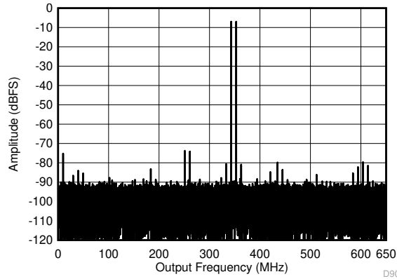
图 5-49. Two Tone FFT at 348 MHz Center
