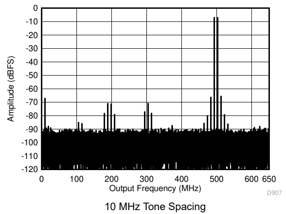
图 5-52. Two Tone FFT at 1798 MHz Center
