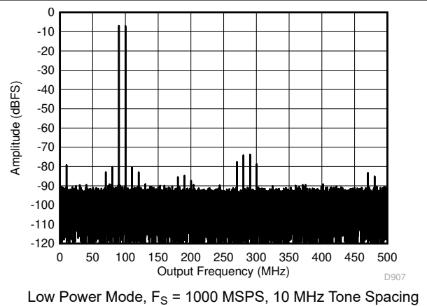
图 5-54. Two Tone FFT at 95.07 MHz Center
