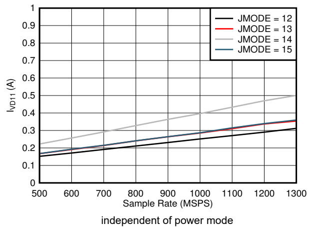
图 5-90. Quad Channel, I_{VD11} vs FS and JMODE 12 - 15
