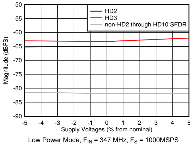
图 5-47. HD2, HD3 and Worst non-HD Spur vs Supply Voltage
