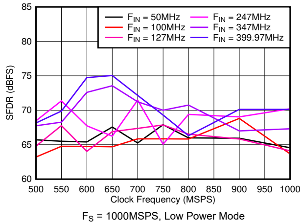
图 5-25. SFDR vs Sample Rate
