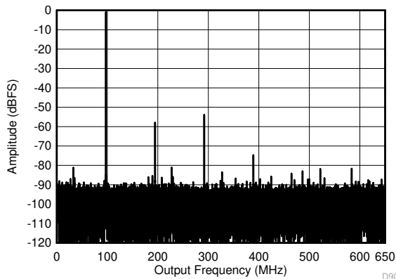
图 5-7. Single Tone FFT at 1497 MHz and -1 dBFS
