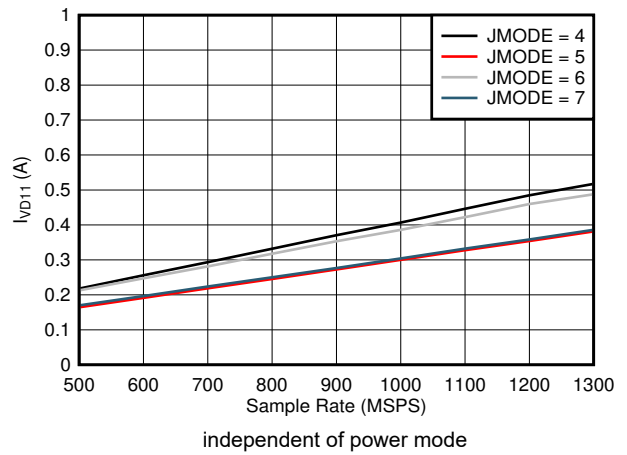
图 5-88. Quad Channel, I_{VD11} vs FS and JMODE 4 - 7
