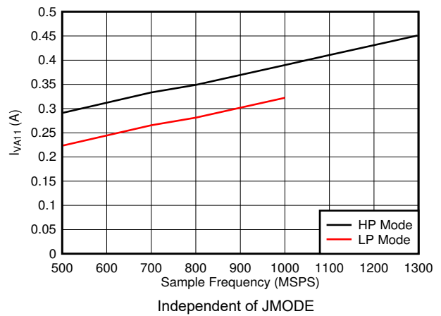
图 5-96. Dual Channel, I_{VA11} vs FS
