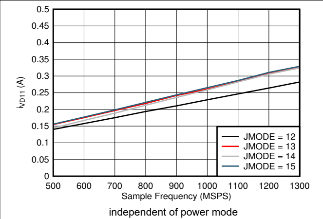
图 5-100. Dual Channel, I_{VD11} vs FS and JMODE 12 - 15
