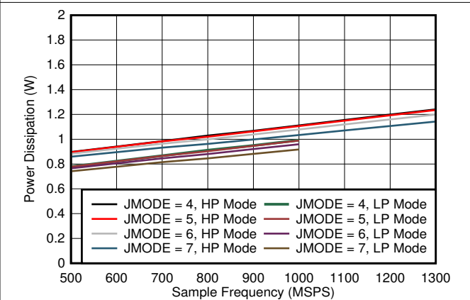
图 5-102. Single Channel, Power Dissipation vs FS for JMODES 4 - 7
