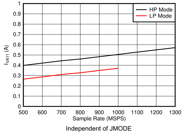
图 5-86. Quad Channel, I_{VA11} vs FS
