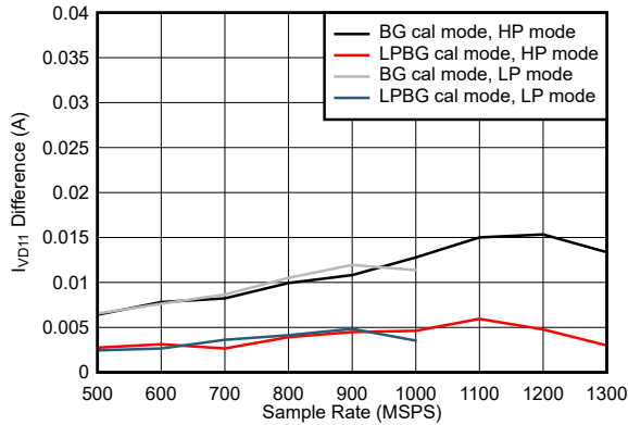
图 5-121. Dual Channel, I_{VD11} Change with Calibration Mode
