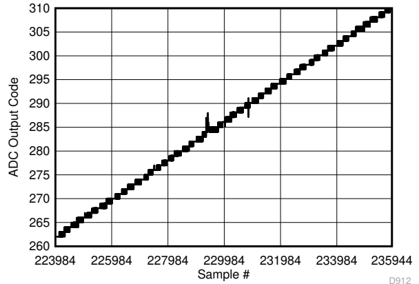
图 5-128. Background Calibration Core Transition (AC Signal Zoomed)
