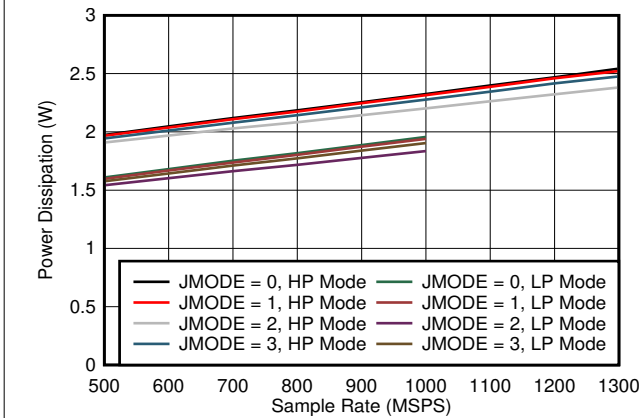
图 5-81. Quad Channel, Power Dissipation vs FS for JMODES 0 - 3
