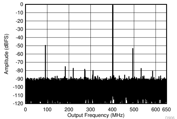
图 5-8. Single Tone FFT at 1797 MHz and -1 dBFS
