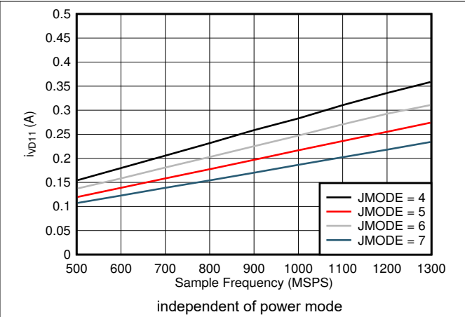
图 5-98. Dual Channel, I_{VD11} vs FS and JMODE 4 - 7
