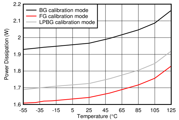
图 5-124. Dual Channel, Power Dissipation vs Temperature
