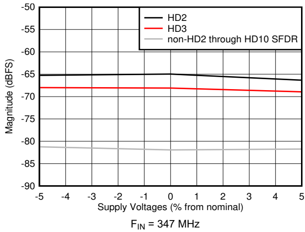
图 5-45. HD2, HD3 and Worst non-HD Spur vs Supply Voltage
