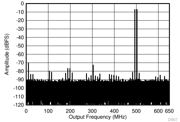
图 5-50. Two Tone FFT at 498 MHz Center
