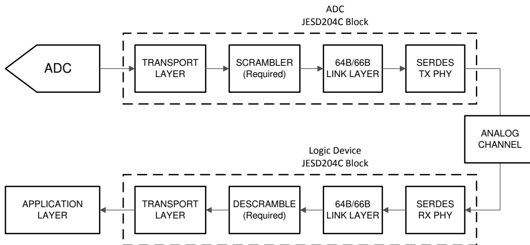
图 6-8. Simplified 64B/66B Encoded JESD204C Interface Diagram
