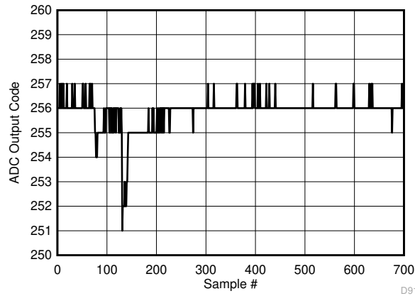
图 5-129. Background Calibration Core Transition (DC Signal)
