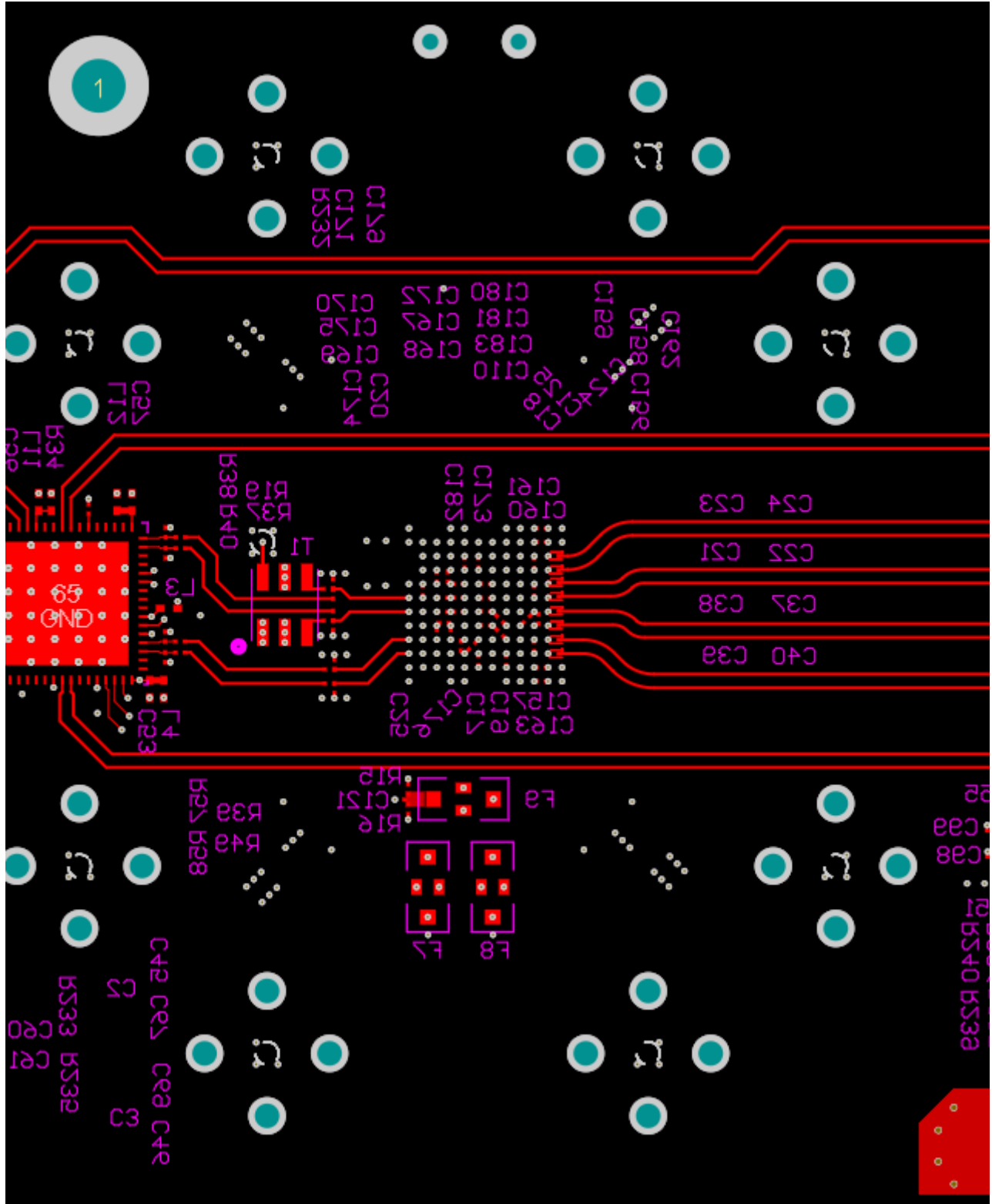
图 7-8. Bottom Layer Routing: CLK±, SYSREF and D[7:4]± Routing
