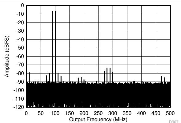
图 5-52. Two Tone FFT at 1798 MHz Center
