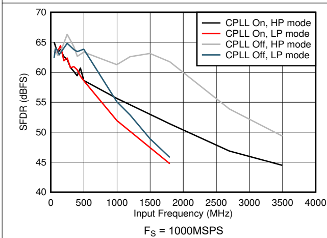
图 5-65. SFDR vs Input Frequency and CPLL
