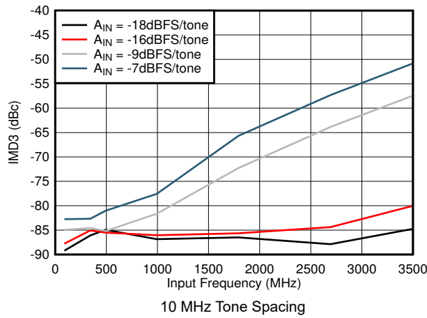
10 MHz Tone Spacing 图 5-57. IMD3 vs Input Frequency
