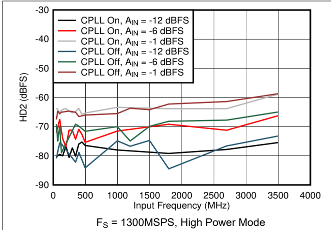
图 5-73. HD2 vs Input Frequency, CPLL and Input Amplitude
