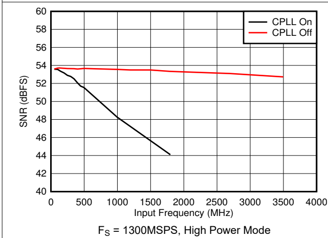
图 5-63. SNR vs Input Frequency and CPLL
