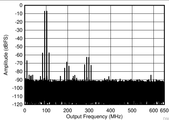
图 5-51. Two Tone FFT at 998 MHz Center
