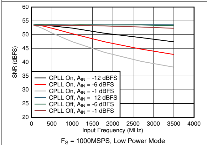
图 5-75. SNR vs Input Frequency, CPLL and Input Amplitude
