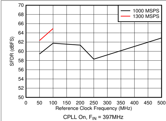
图 5-61. SFDR vs Reference Clock Frequency
