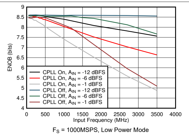
图 5-78. ENOB vs Input Frequency, CPLL and Input Amplitude
