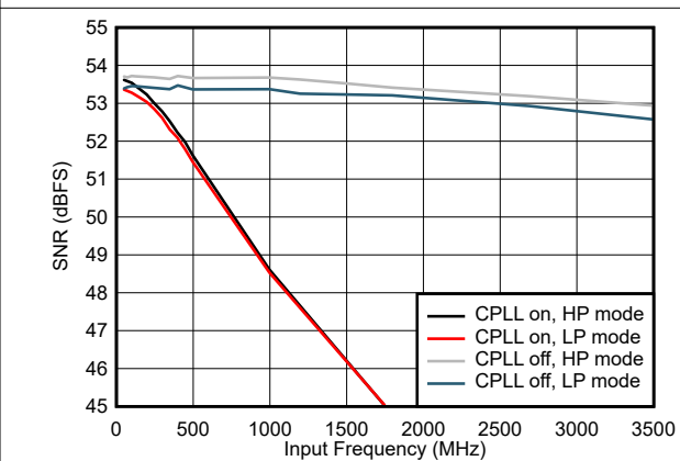
图 5-66. SNR vs Input Frequency and CPLL and Power Mode
