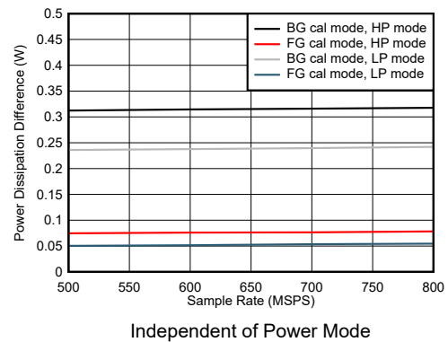
图 5-102. Dual Channel, Power Dissipation Change with Calibration Mode
