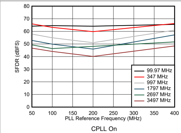
图 5-64. SFDR vs Reference Clock Frequency
