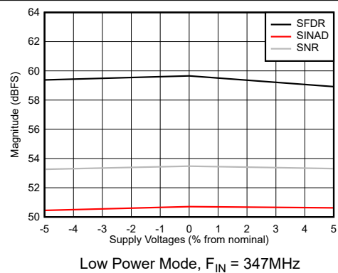
图 5-48. SNR, SFDR and SINAD vs Supply Voltage
