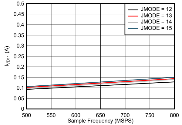
图 5-100. Single Channel, I_{VD11} vs F_S for JMODES 12 - 15
