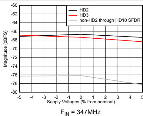
图 5-47. HD2, HD3 and Worst non-HD2/3 Spur vs Supply Voltage
