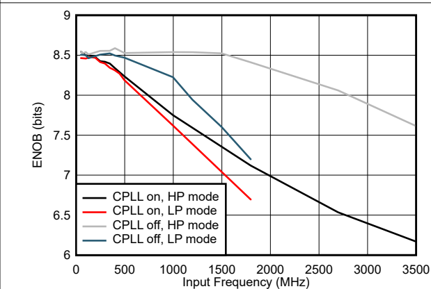
图 5-68. ENOB vs Input Frequency and CPLL and Power Mode
