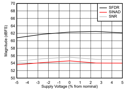
图 6-100. DES Mode: SNR, SINAD and SFDR vs Supply Voltage
