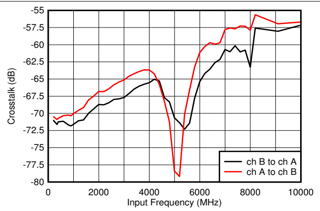
图 6-2. Crosstalk vs Input Frequency
