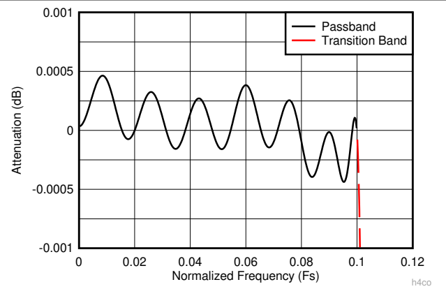
图 7-12. Decimate-by-4 Composite Zoomed Pass-Band Response
