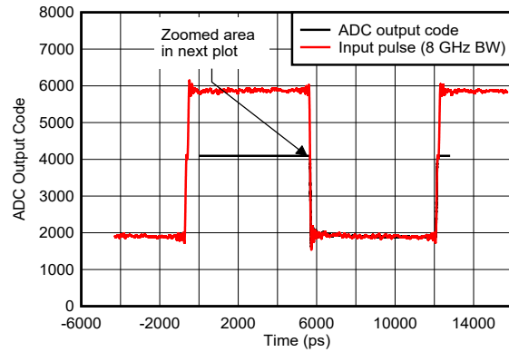
图 6-148. Pulse Overdrive Recovery
