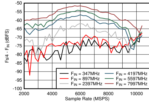
图 6-44. DES Mode: F_s/4 - F_{IN} vs Sample Rate and Input Frequency
