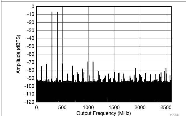
图 6-21. Dual Channel Mode: Single Tone FFT at 5597 MHz
