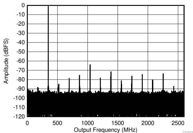
图 6-17. Dual Channel Mode: Single Tone FFT at 347 MHz
