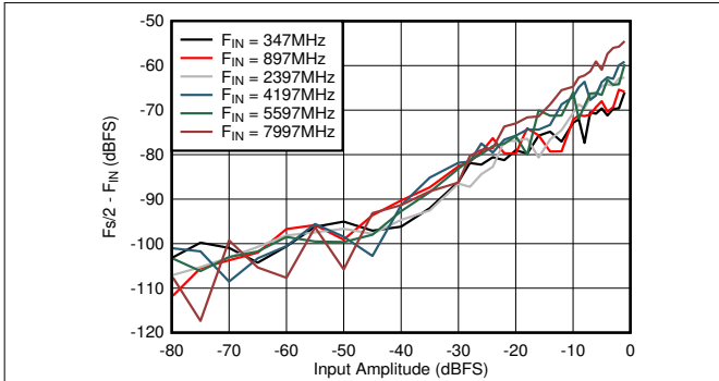
图 6-67. DES Mode: F_s/2 - F_{IN} vs Input Amplitude and Frequency
