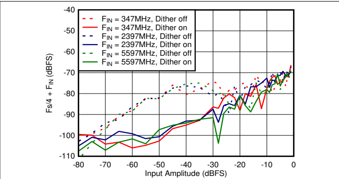
图 6-68. DES Mode: F_s/2 - F_{IN} vs Input Amplitude and Dither
