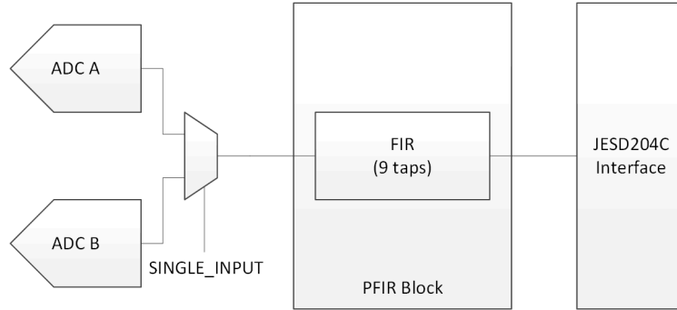
图 7-5. Single Channel Equalization PFIR Block Diagram
