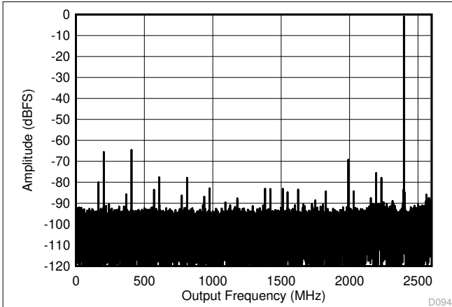
图 6-19. Dual Channel Mode: Single Tone FFT at 2397 MHz
