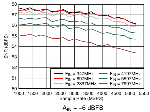
图 6-46. Dual Channel Mode: SNR vs Sample Rate and Input Frequency A_{IN} = -6\text{ dBFS}
