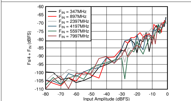
图 6-69. DES Mode: F_s/4 + F_{IN} vs Input Amplitude and Frequency
