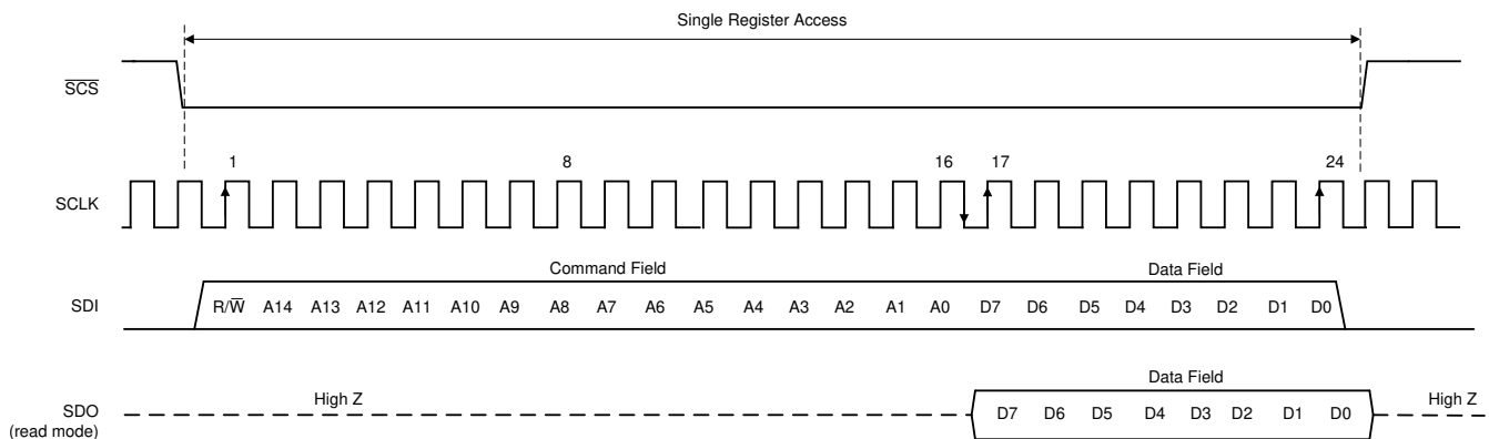
图 7-26. Serial Interface Protocol: Single Read/Write
