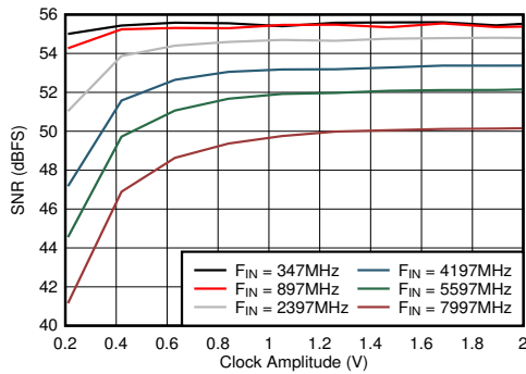
图 6-85. Dual Channel Mode: SNR vs Clock Amplitude
