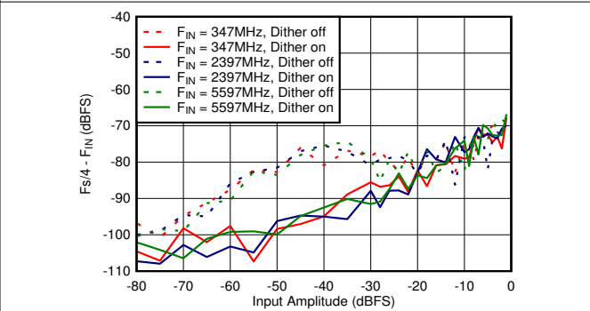
图 6-72. DES Mode: F_s/4 - F_{IN} vs Input Amplitude and Dither
