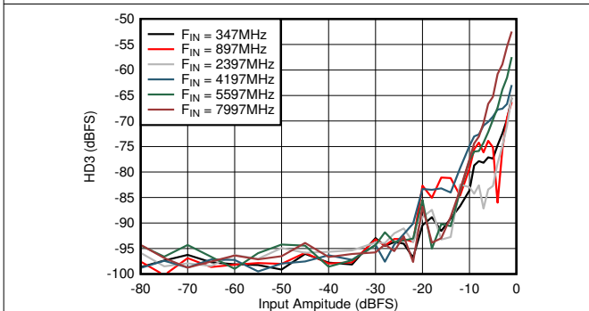
图 6-65. DES Mode: HD3 vs Input Amplitude and Frequency
