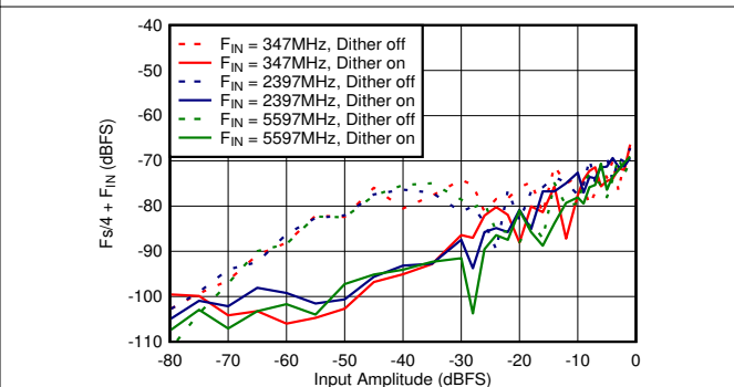
图 6-70. DES Mode: F_s/4 + F_{IN} vs Input Amplitude and Dither
