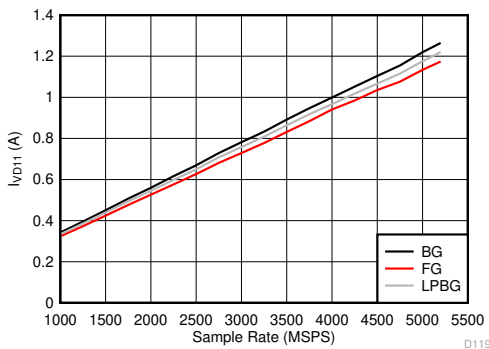
图 6-135. Dual Channel Mode: I_{VD11} vs Sample Rate
