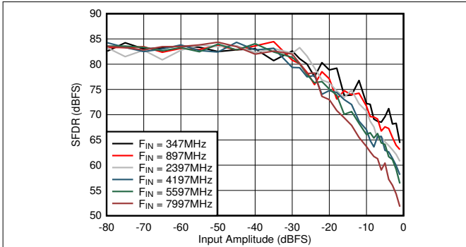
图 6-61. DES Mode: SFDR vs Input Amplitude and Frequency
