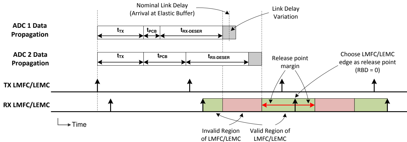
图 7-23. LMFC/LEMV Valid Region Definition for Elastic Buffer Release Point Selection
