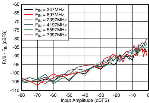
图 6-81. Dual Channel Mode: F_s/2 - F_{IN} vs Input Amplitude and Frequency
