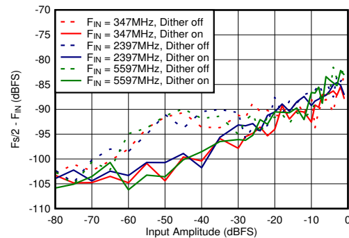
图 6-82. Dual Channel Mode: F_s/2 - F_{IN} vs Input Amplitude and Dither
