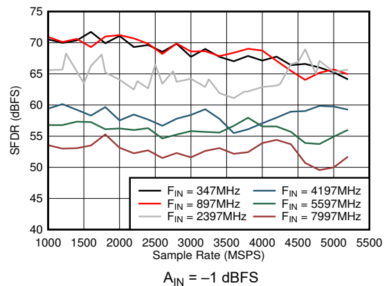
图 6-48. Dual Channel Mode: SFDR vs Sample Rate and Input Frequency A_{IN} = -1\text{ dBFS}
