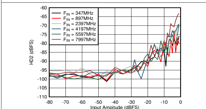
图 6-63. DES Mode: HD2 vs Input Amplitude and Frequency
