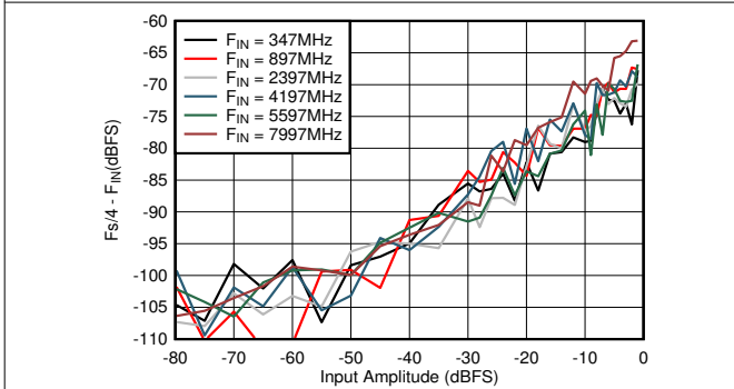
图 6-71. DES Mode: F_s/4 - F_{IN} vs Input Amplitude and Frequency
