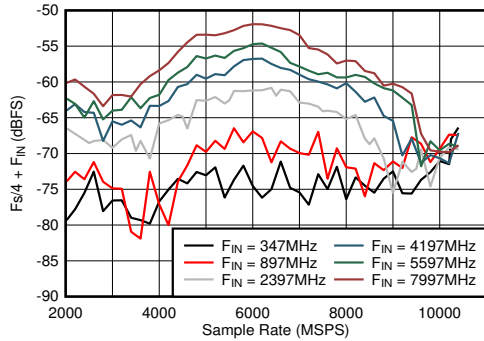
图 6-43. DES Mode: F_s/4 + F_{IN} vs Sample Rate and Input Frequency
