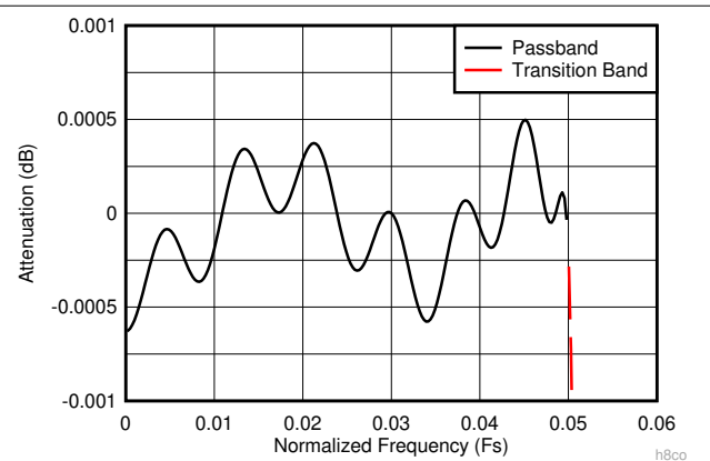
图 7-14. Decimate-by-8 Composite Zoomed Pass-Band Response
