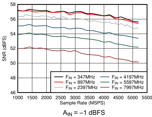
图 6-45. Dual Channel Mode: SNR vs Sample Rate and Input Frequency A_{IN} = -1\text{ dBFS}
