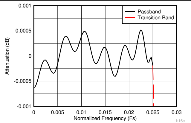
图 7-16. Decimate-by-16 Composite Zoomed Pass-Band Response
