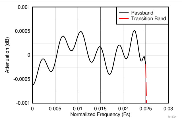
图 6-16. Decimate-by-16 Composite Zoomed Pass-Band Response
