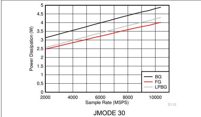
图 5-129. DES Mode: Power Dissipation vs Sample Rate
