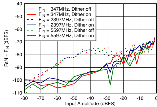
图 5-66. DES Mode: F_s/4 - F_{\text{IN}} vs Input Amplitude and Dither
