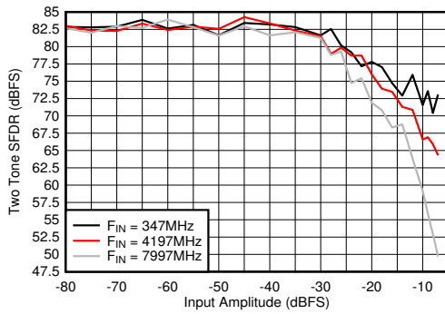
图 5-103. DES Mode: Two Tone SFDR vs Input Amplitude
