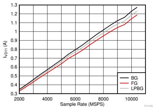
图 5-123. DES Mode: I_{VD11} vs Sample Rate
