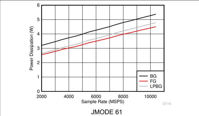
图 5-130. DES Mode: Power Dissipation vs Sample Rate
