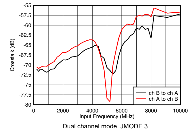
图 5-2. Crosstalk vs Input Frequency
