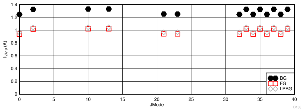
图 5-116. Dual Channel Mode: Power Dissipation vs JMODE at 5.2GSPS
