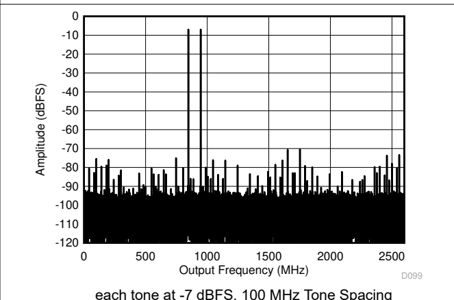
图 5-24. Dual Channel Mode: Two Tone FFT at 897 MHz
