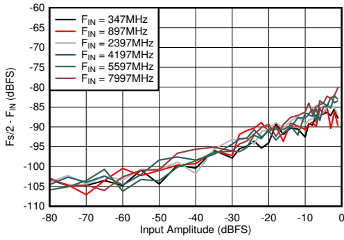
图 5-79. Dual Channel Mode: F_s/2 - F_{IN} vs Input Amplitude and Frequency
