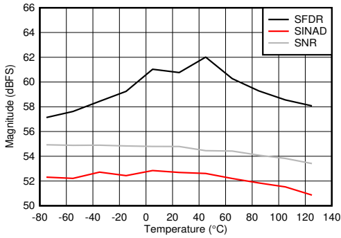
FG calibration at each temperature 图 5-85. DES Mode: SNR, SINAD and SFDR vs Temperature
