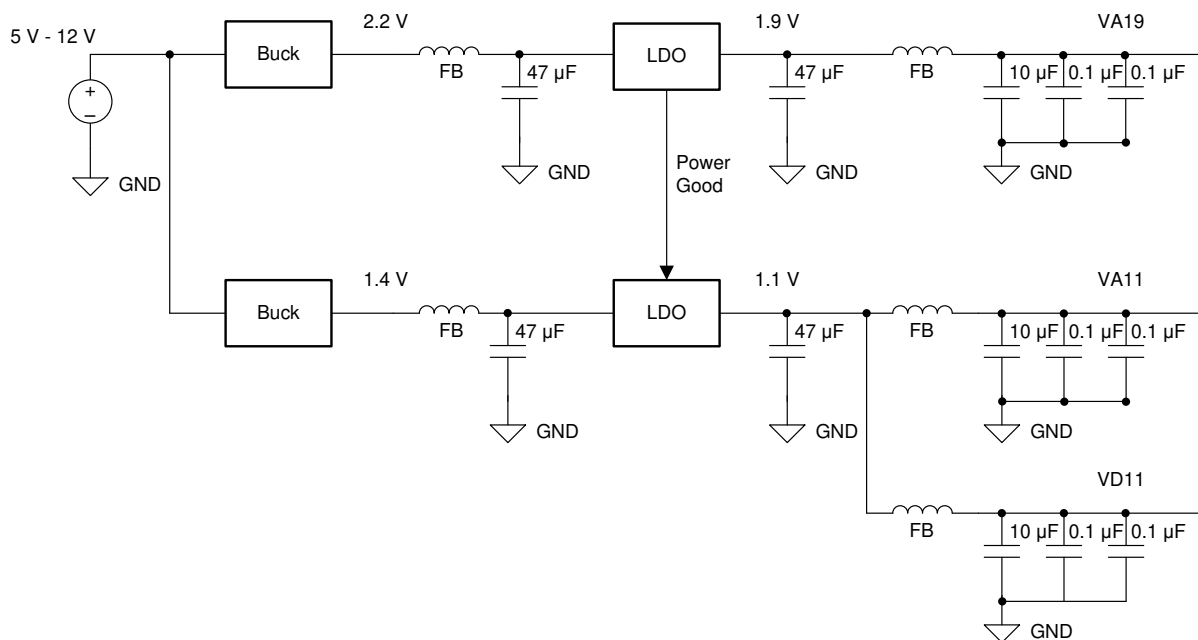
图 7-13. LDO Linear Regulator Approach Example
