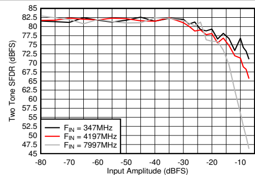
图 5-108. Dual Channel Mode: Two Tone SFDR vs Input Amplitude
