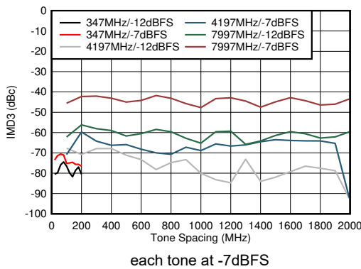
图 5-101. DES Mode: IMD3 vs Tone Spacing
