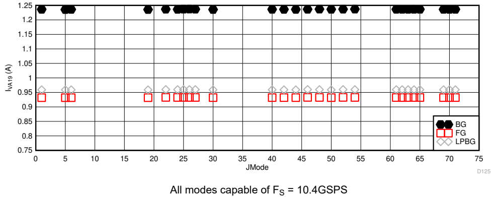
图 5-109. DES Mode: I_{VA19} vs JMODE at 10.4GSPS
