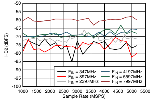
图 5-50. Dual Channel Mode: HD2 vs Sample Rate and Input Frequency
