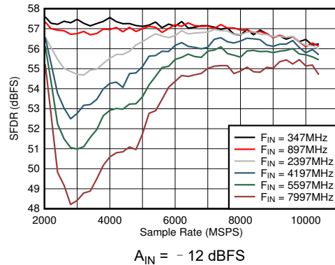
图 5-34. DES Mode: SFDR vs Sample Rate and Input Frequency
