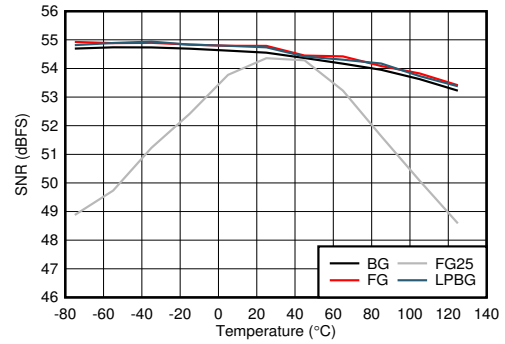
FG25 is calibrated at 25^\circ\text{C} and held at other temperatures, other modes recalibrated at each temperature 图 5-86. DES Mode: SNR vs Temperature and Calibration Mode
