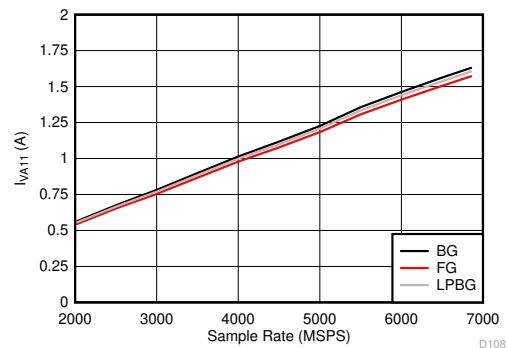
图 5-122. DES Mode: I_{VA11} vs Sample Rate
