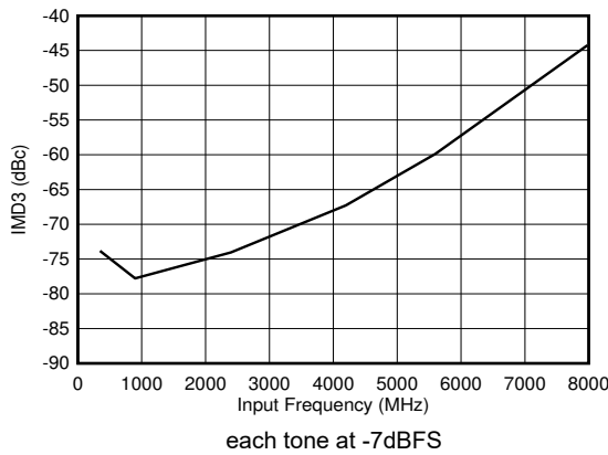
图 5-99. DES Mode: IMD3 vs Input Frequency
