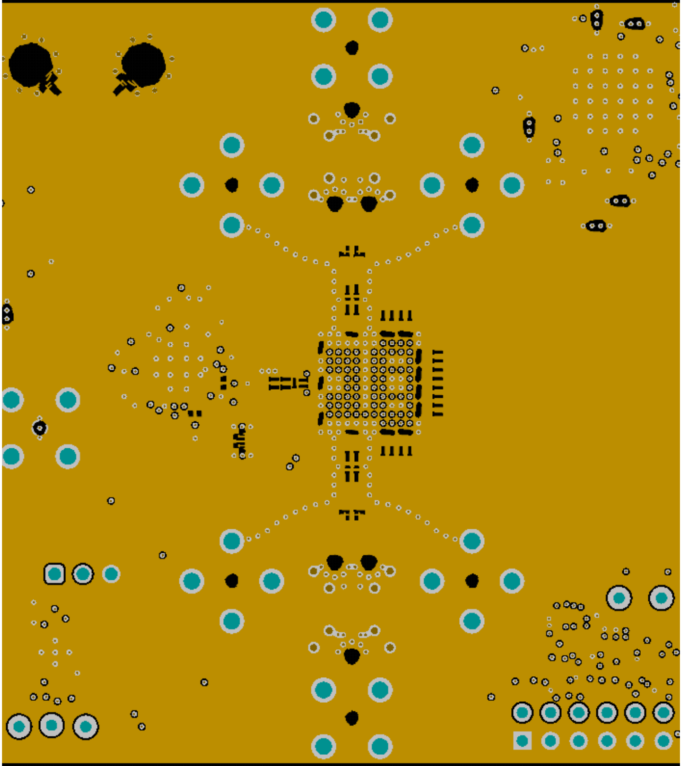
图 7-16. GND1 Cutouts to Optimize Impedance of Component Pads
