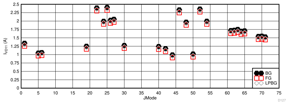
图 5-110. DES Mode: I_{VA11} vs JMODE at 10.4GSPS
