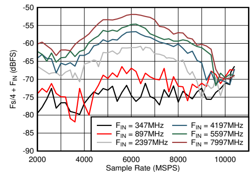
图 5-42. DES Mode: F_s/4 + F_{\text{IN}} vs Sample Rate and Input Frequency
