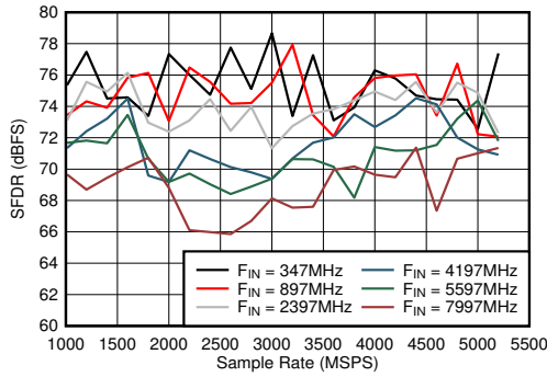
图 5-49. Dual Channel Mode: SFDR vs Sample Rate and Input Frequency
