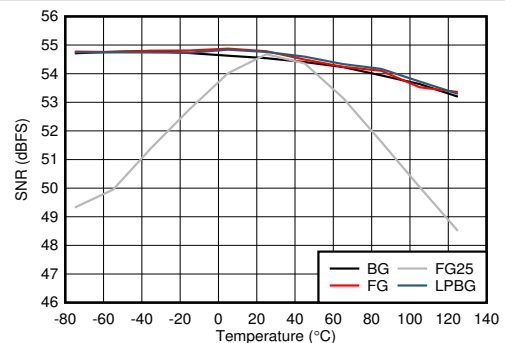
FG25 is calibrated at 25^\circ\text{C} and held at other temperatures, other modes recalibrated at each temperature 图 5-90. Dual Channel Mode: SNR vs Temperature and Calibration Mode
