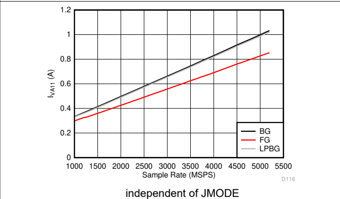
图 5-132. Dual Channel Mode: I_{VA11} vs Sample Rate
