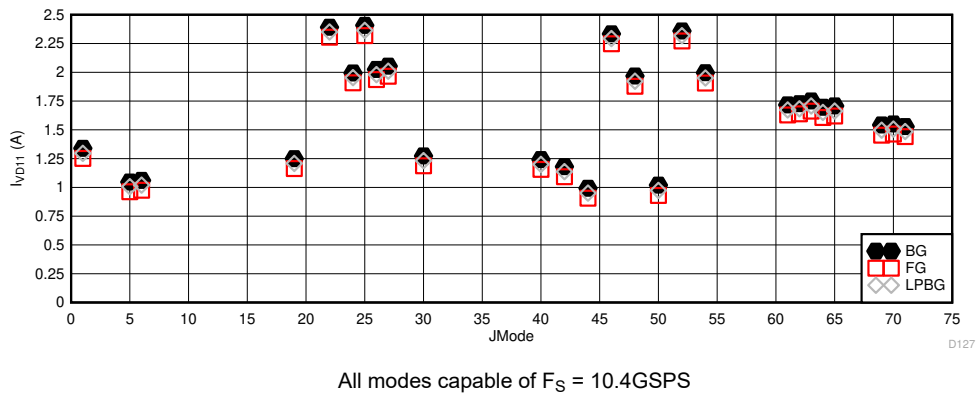
图 5-111. DES Mode: I_{VD11} vs JMODE at 10.4GSPS
