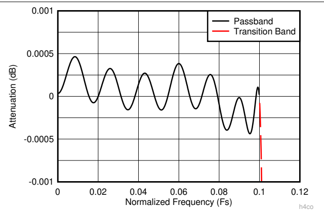
图 6-12. Decimate-by-4 Composite Zoomed Pass-Band Response
