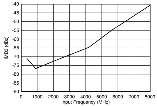
图 5-104. Dual Channel Mode: IMD3 vs Input Frequency each tone at -7dBFS
