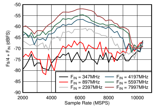
图 5-42. DES Mode: F_s/4 + F_{\text{IN}} vs Sample Rate and Input Frequency
