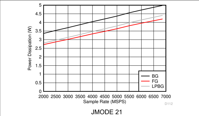
图 5-128. DES Mode: Power Dissipation vs Sample Rate
