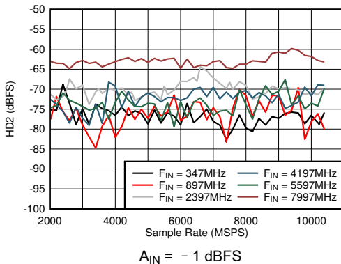
图 5-35. DES Mode: HD2 vs Sample Rate and Input Frequency
