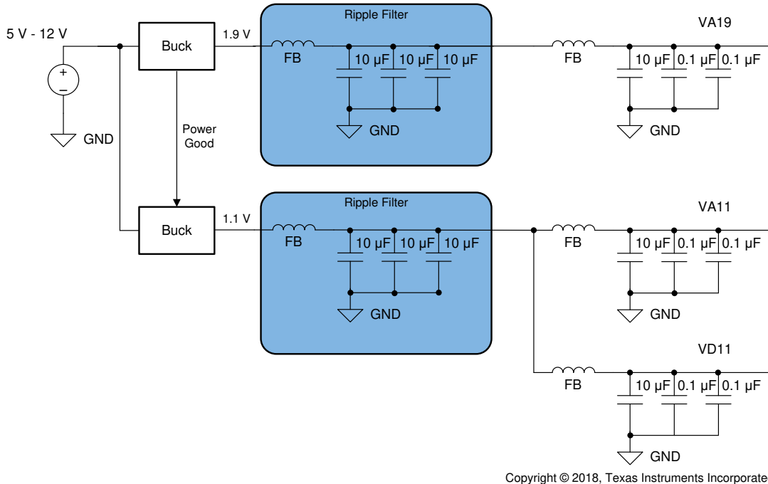
图 7-14. Switcher-Only Approach Example
