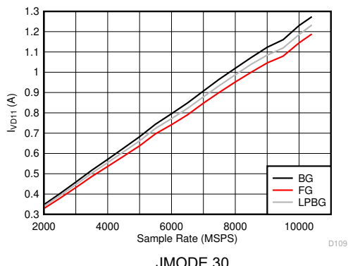
图 5-125. DES Mode: I_{VD11} vs Sample Rate
