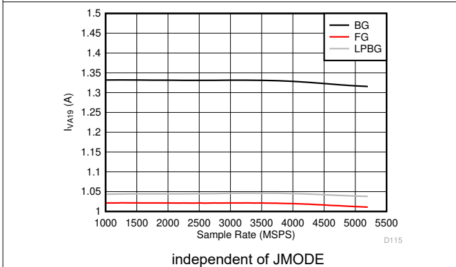
图 5-131. Dual Channel Mode: I_{VA19} vs Sample Rate
