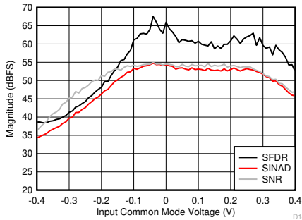
图 5-97. SNR, SFDR and SINAD vs Input Common Mode Voltage
