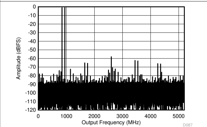
图 5-12. DES Mode: Two Tone FFT at 897 MHz
