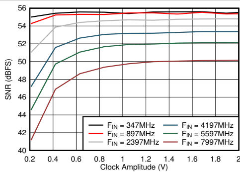
图 5-83. Dual Channel Mode: SNR vs Clock Amplitude
