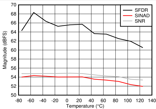
FG calibration at each temperature 图 5-89. Dual Channel Mode: SNR, SINAD and SFDR vs Temperature
