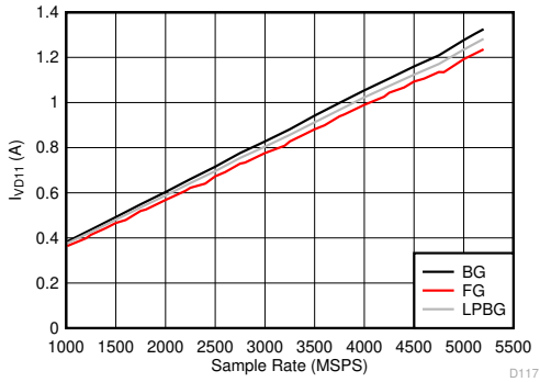
图 5-133. Dual Channel Mode: I_{VD11} vs Sample Rate
