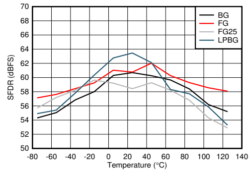
FG25 is calibrated at 25^\circ\text{C} and held at other temperatures, other modes recalibrated at each temperature 图 5-88. DES Mode: SFDR vs Temperature and Calibration Mode
