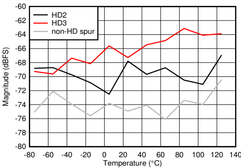
FG calibration at each temperature 图 5-87. DES Mode: HD2, HD3 and Worst non-HD Spur vs Temperature
