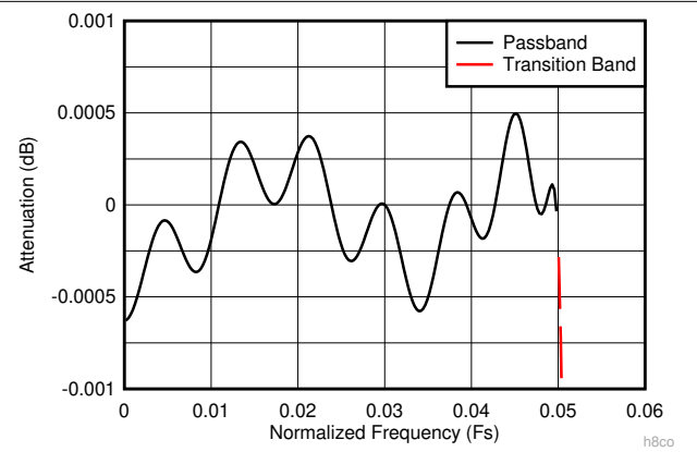
图 6-14. Decimate-by-8 Composite Zoomed Pass-Band Response
