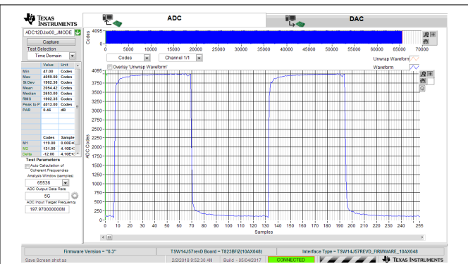
图 7-7. 40-MHz, Square-Wave Time Domain for 5-GSPS, Single-Channel Oscilloscope
