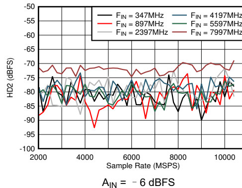
图 5-36. DES Mode: HD2 vs Sample Rate and Input Frequency
