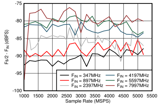
图 5-56. Dual Channel Mode: F_s/2 - F_{IN} vs Sample Rate and Input Frequency
