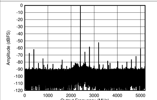
图 5-10. DES Mode: Single Tone FFT at 7997 MHz
