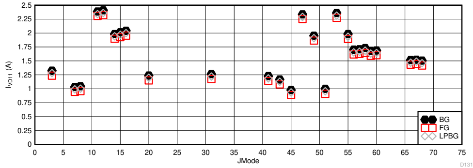
图 5-115. Dual Channel Mode: I_{VD11} vs JMODE at 5.2GSPS
