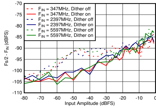
图 5-80. Dual Channel Mode: F_s/2 - F_{IN} vs Input Amplitude and Dither
