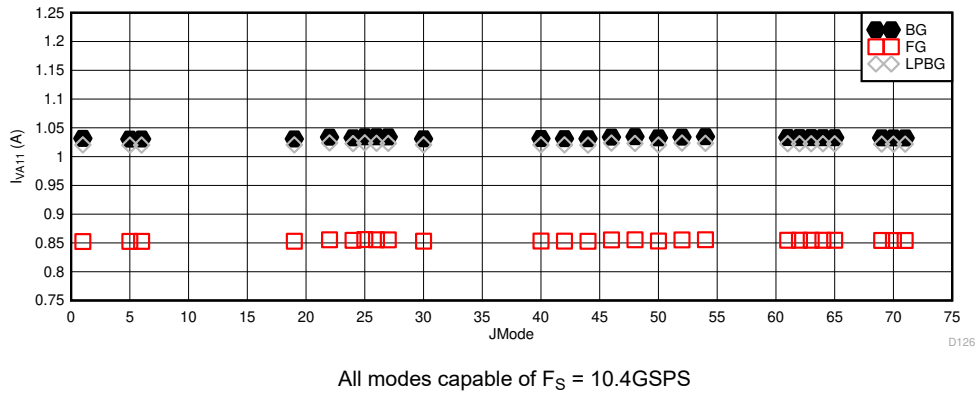
图 5-110. DES Mode: I_{VA11} vs JMODE at 10.4GSPS
