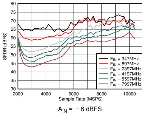
图 5-33. DES Mode: SFDR vs Sample Rate and Input Frequency
