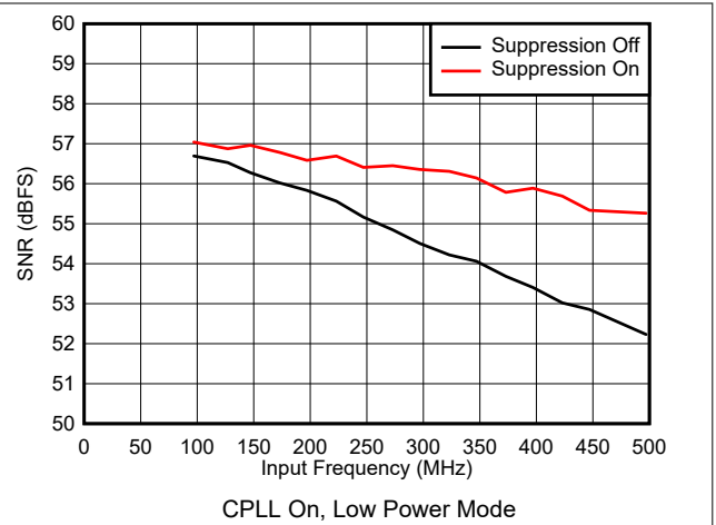
图 5-60. SNR vs Input Frequency
