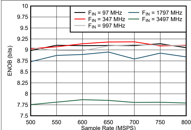
图 5-31. ENOB vs Sample Rate
