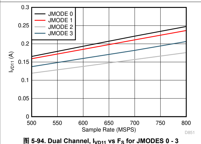
图 5-94. Dual Channel, I_{VD11} vs F_S for JMODES 0 - 3
