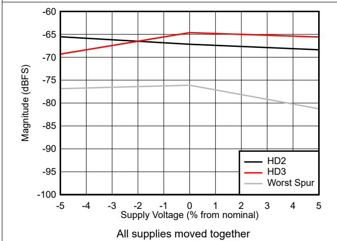
图 5-39. HD2, HD3 and worst non-HD vs Supply Voltage
