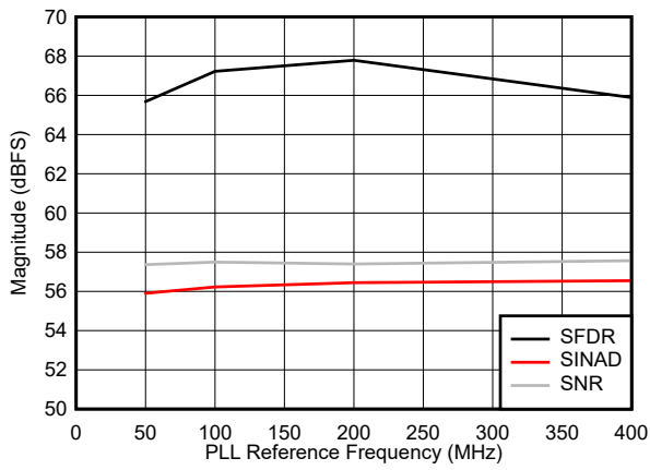
图 5-42. SNR, SFDR and SINAD vs Reference Frequency with PLL on
