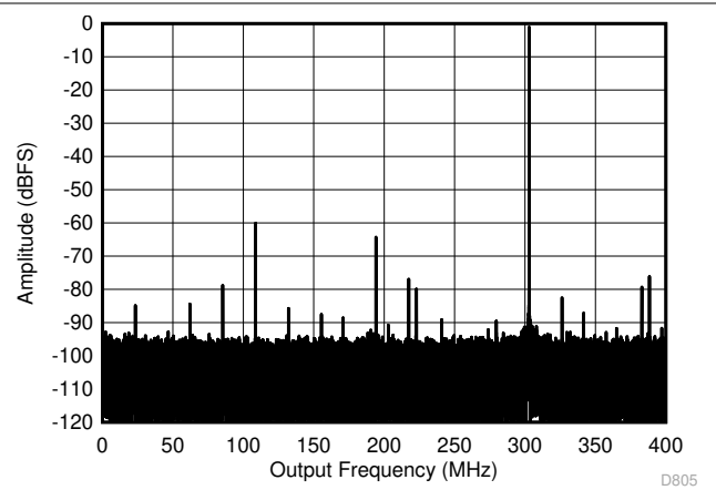
图 5-8. Single Tone FFT at 2097 MHz and -1dBFS
