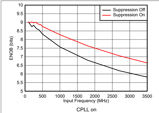
图 5-37. ENOB vs Input Frequency and Suppression
