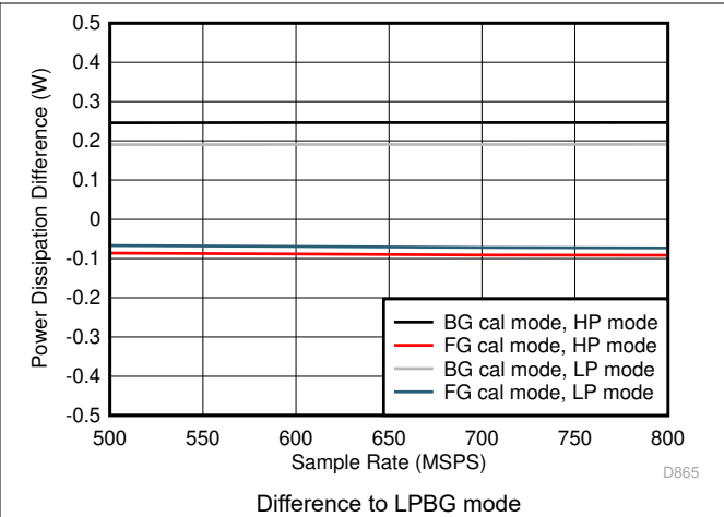
图 5-84. Quad Channel, Power Dissipation vs F_S over Modes
