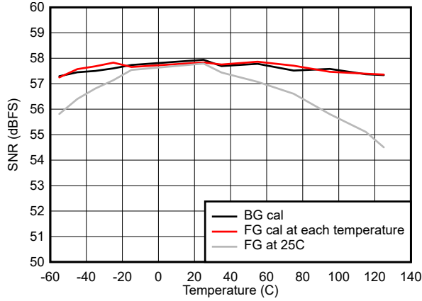
图 5-43. SNR vs Temperature
