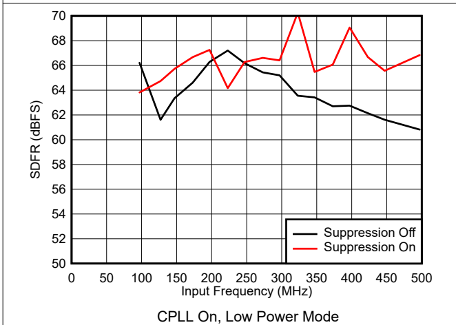
图 5-61. SFDR vs Input Frequency
