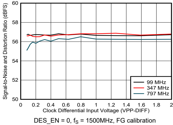
图 5-128. SINAD vs Clock Amplitude
