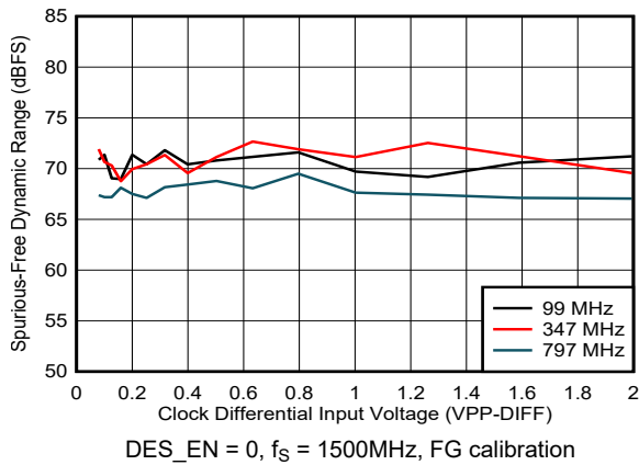
图 5-132. SFDR vs Clock Amplitude
