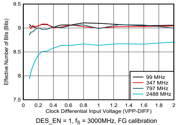
图 5-131. ENOB vs Clock Amplitude
