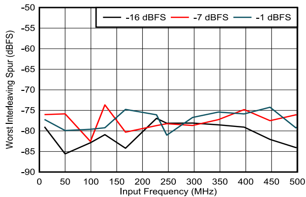
DES_EN = 0, f_S = 500\text{MHz} , FG calibration, includes f_S / 2 - f_{IN} spur only
