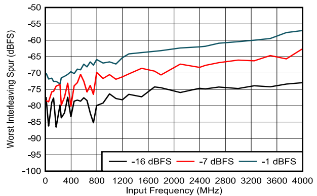
DES_EN = 1, f_S = 4000\text{MHz} , FG calibration, includes f_{IN} and f_S / 4 \pm f_{IN} spurs only
