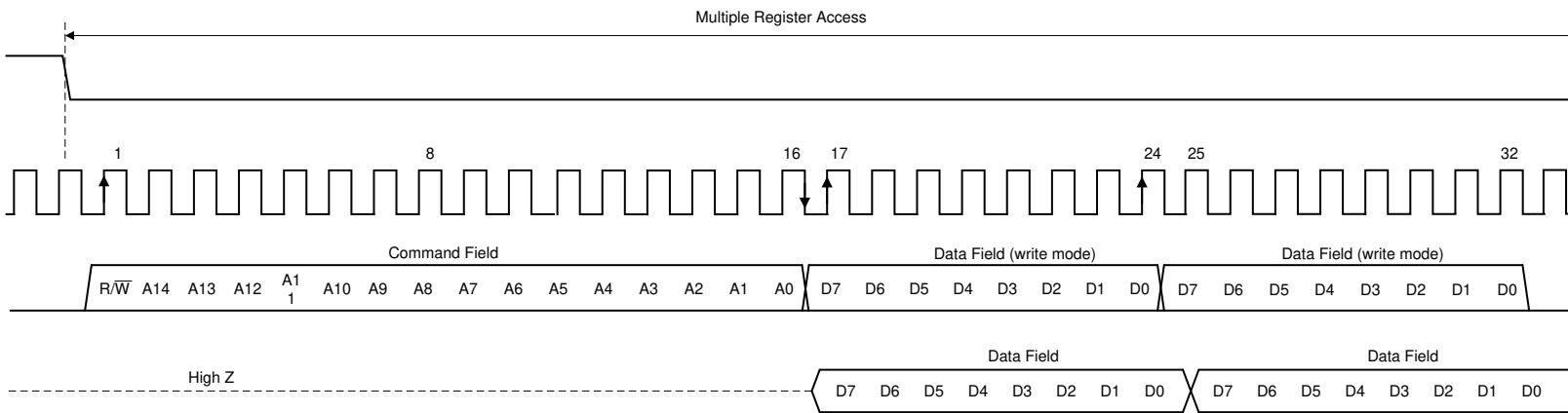
图 6-6. Serial Interface Protocol: Streaming Read/Write Operation
