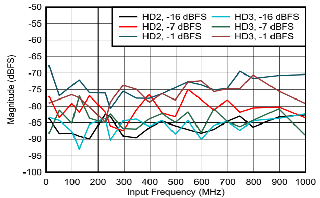
DES_EN = 1, f_S = 1000\text{MHz} , FG calibration
