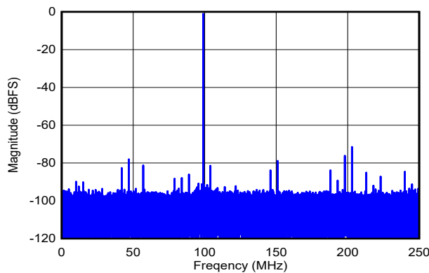
DES_EN = 0, f_S = 500\text{MHz} , FG calibration, SNR = 57.5dBFS, SFDR = 71.4dBFS, ENOB = 9.2 bits
