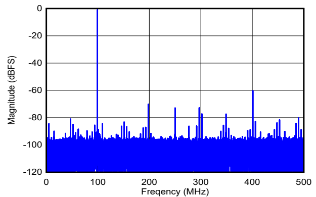
DES_EN = 1, f_S = 1000\text{MHz} , FG calibration, SNR = 57.1dBFS, SFDR = 60.5dBFS, ENOB = 8.8 bits
