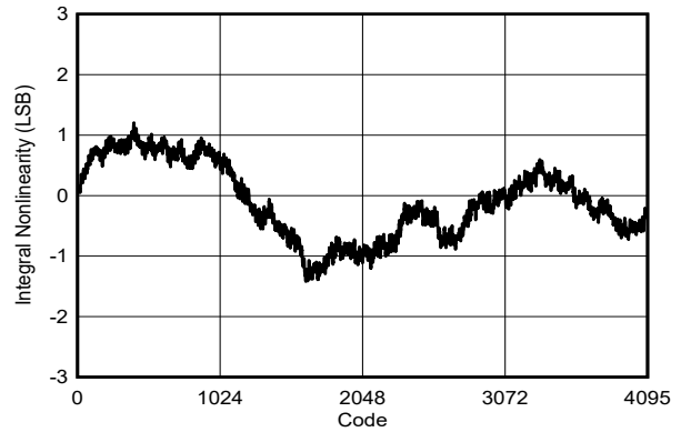
DES_EN = 1, f_S = 4000\text{MHz} , FG calibration, F_{IN} = 99\text{MHz}
