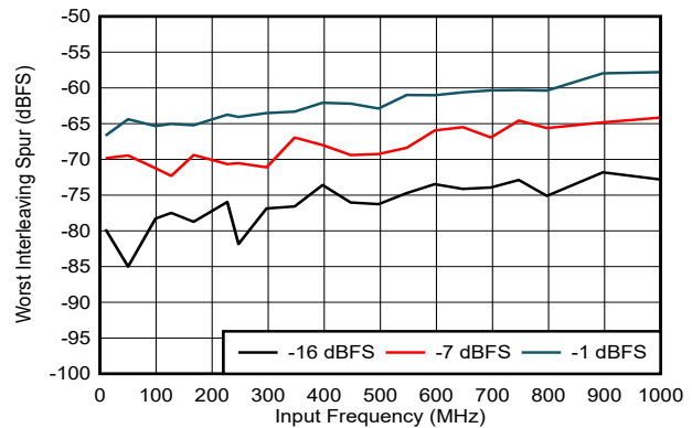
DES_EN = 1, f_S = 1000\text{MHz} , FG calibration, includes f_S / 2 - f_{IN} and f_S / 4 \pm f_{IN} spurs only
