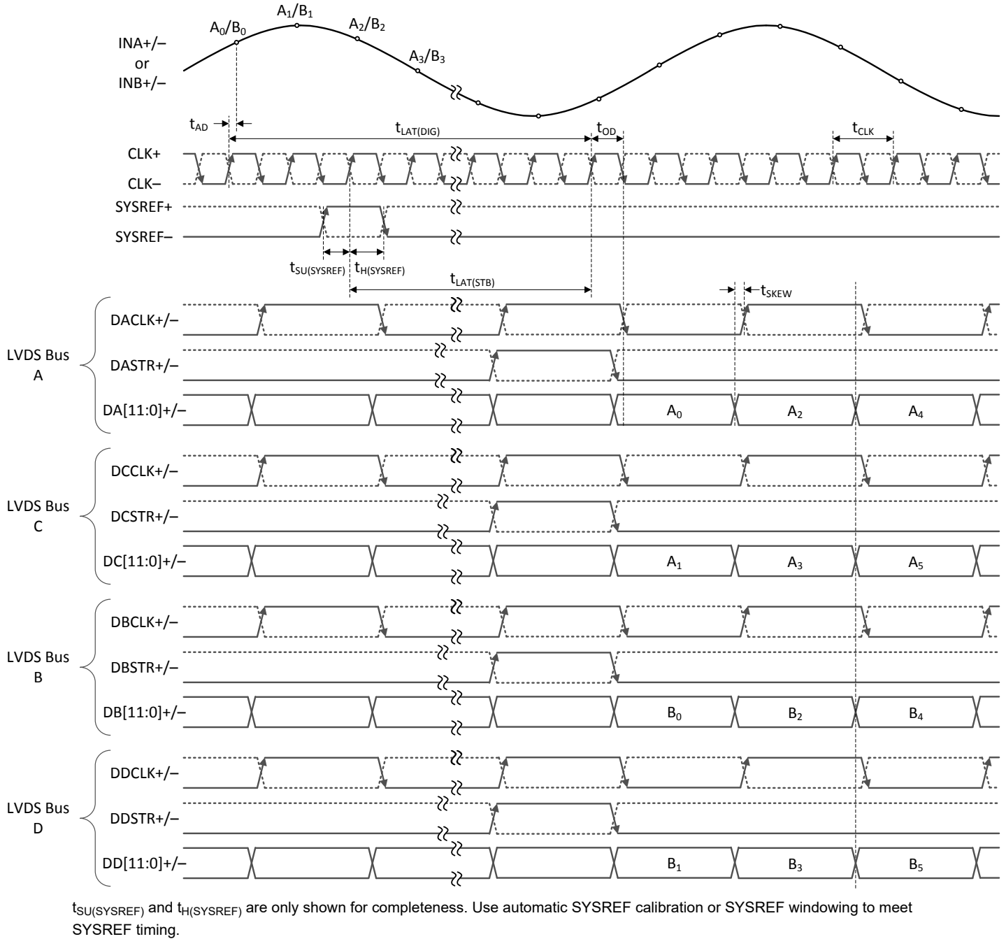
图 5-3. Dual-Channel, 4-Bus, Aligned-Mode Timing (LDEMUX = 1, DES_EN = 0, LALIGNED = 1)
