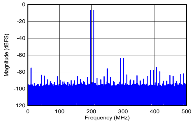
DES_EN = 1, f_S = 1000\text{MHz} , FG calibration, f_1 = 792\text{MHz} , f_2 = 802\text{MHz} , A_{IN} = -7\text{dBFS} per tone, SFDR = -64dBFS, IMD3 = -87dBFS, IMD2 = -75dBFS
