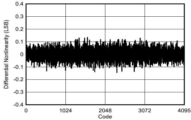
DES_EN = 1, f_S = 4000\text{MHz} , FG calibration, F_{IN} = 99\text{MHz}
