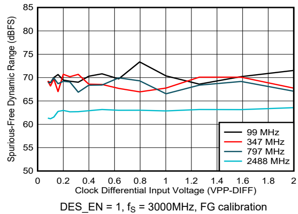
图 5-133. SFDR vs Clock Amplitude
