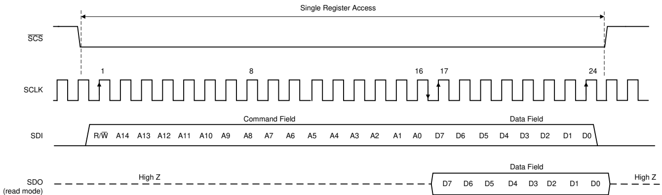
图 6-5. Serial Interface Protocol: Single Read/Write Operation
