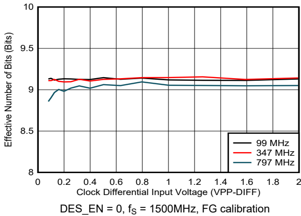
图 5-130. ENOB vs Clock Amplitude
