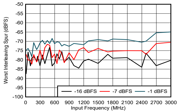
DES_EN = 1, f_S = 3000\text{MHz} , FG calibration, includes f_{IN} and f_S / 4 \pm f_{IN} spurs only
