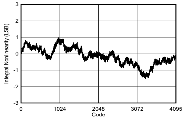
DES_EN = 0, f_S = 2000\text{MHz} , FG calibration, F_{IN} = 99\text{MHz}
