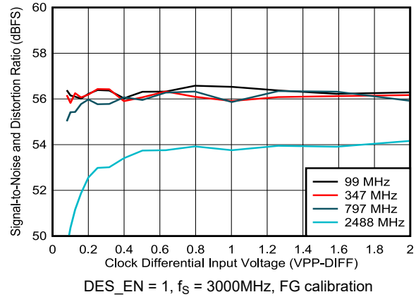
图 5-129. SINAD vs Clock Amplitude
