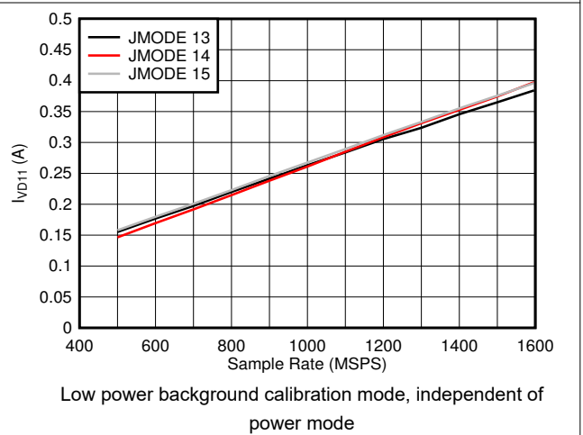
图 6-98. Dual Channel, Power Dissipation vs F_S and JMODE 13 - 15
