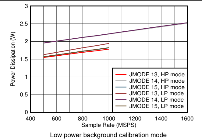
图 6-82. Quad Channel, Power Dissipation vs F_S and JMODE 13 - 15
