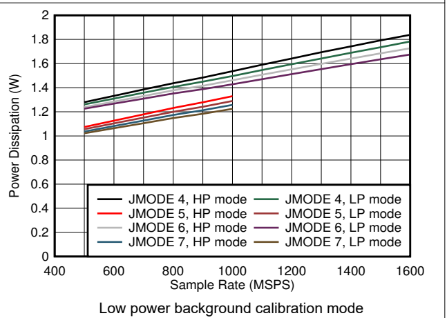
图 6-90. Dual Channel, Power Dissipation vs F_S and JMODE 4 - 7
