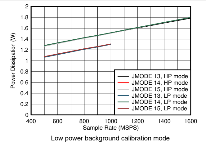
图 6-92. Dual Channel, Power Dissipation vs F_S and JMODE 13 - 15
