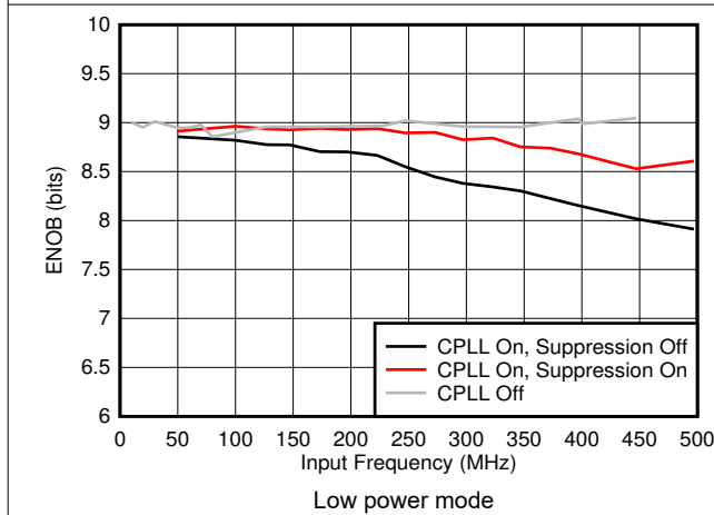
图 6-47. ENOB vs F_{IN} and C-PLL modes
