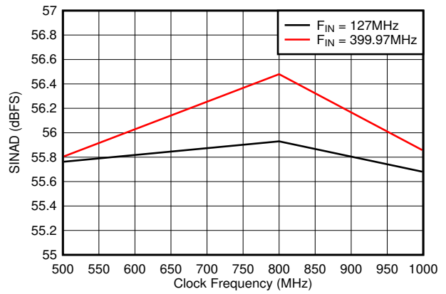
图 6-30. SINAD vs Sample Rate
