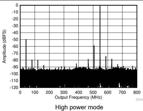
图 6-11. Single Tone FFT at 3797 MHz and -1 dBFS
