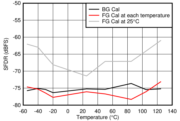
图 6-68. Worst Spur vs Temperature
