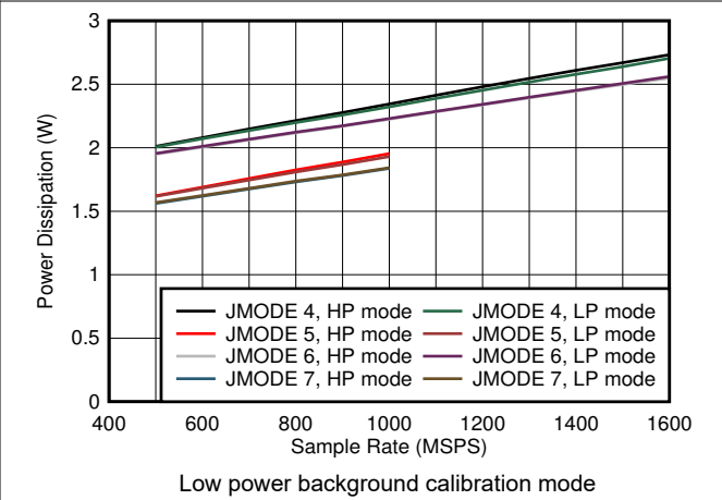
图 6-80. Quad Channel, Power Dissipation vs F_S and JMODE 4 - 7
