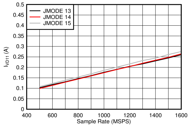
图 6-108. Single Channel, I_{VD11} vs F_S and JMODE 13 - 15
