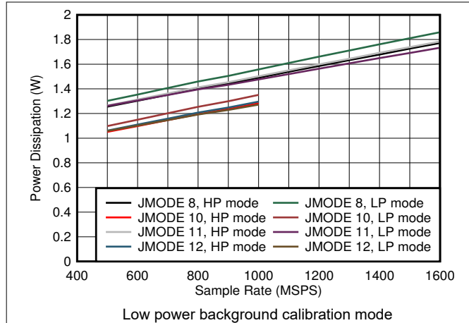
图 6-91. Dual Channel, Power Dissipation vs F_S and JMODE 8 - 12
