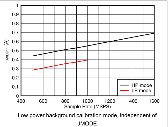
图 6-84. Quad Channel, I_{VDD11} vs F_S
