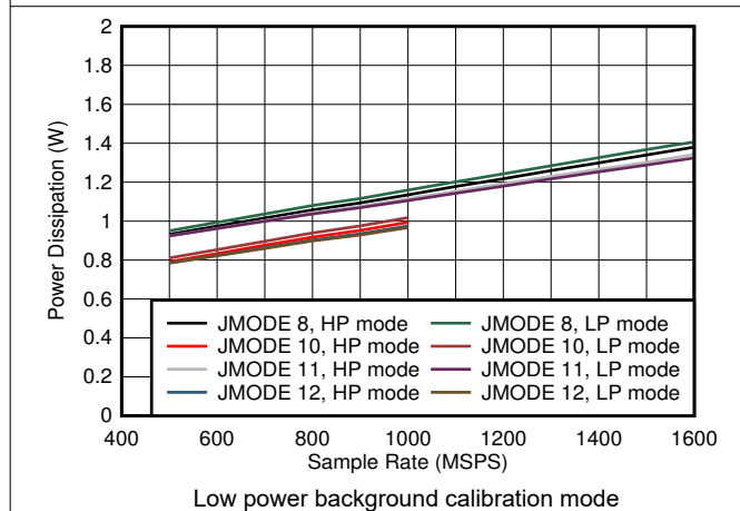
图 6-101. Single Channel, Power Dissipation vs F_S and JMODE 8 - 12
