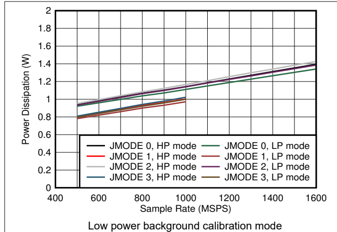
图 6-99. Single Channel, Power Dissipation vs F_S and JMODE 0 - 3
