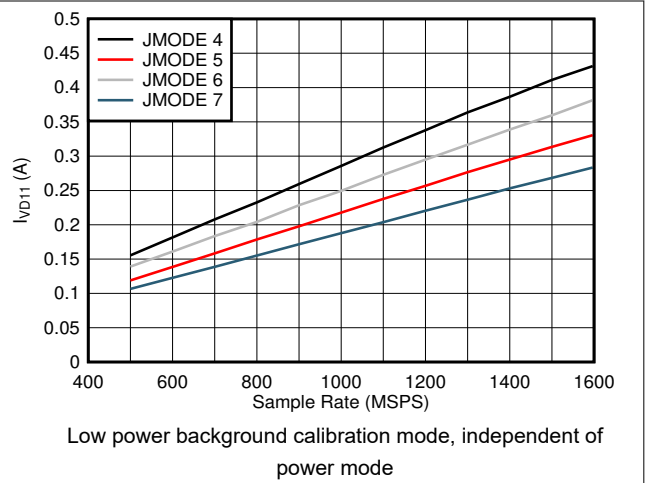
图 6-96. Dual Channel, Power Dissipation vs F_S and JMODE 4 - 7
