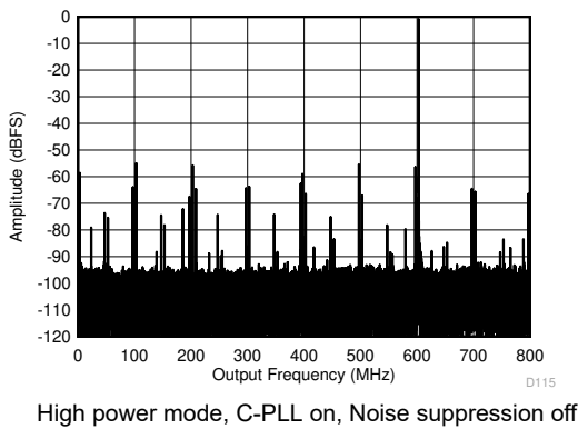
图 6-9. Single Tone FFT at 997 MHz and -1 dBFS
