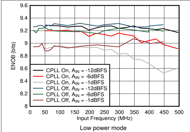
图 6-57. ENOB vs A_{IN} and C-PLL
