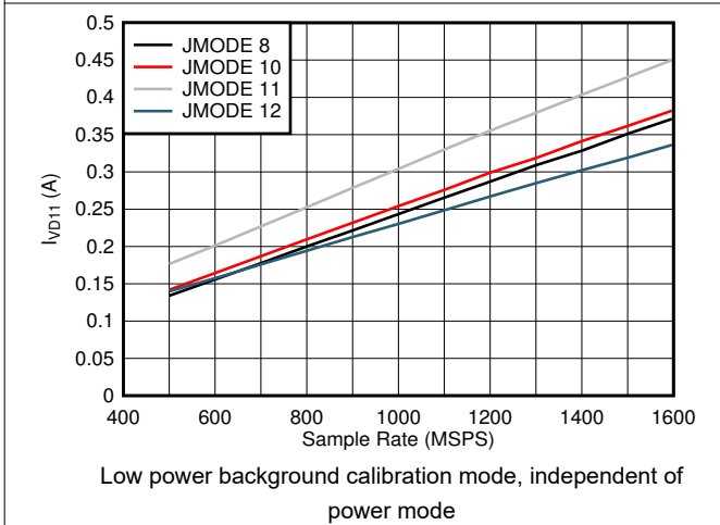
图 6-97. Dual Channel, Power Dissipation vs F_S and JMODE 8 - 12
