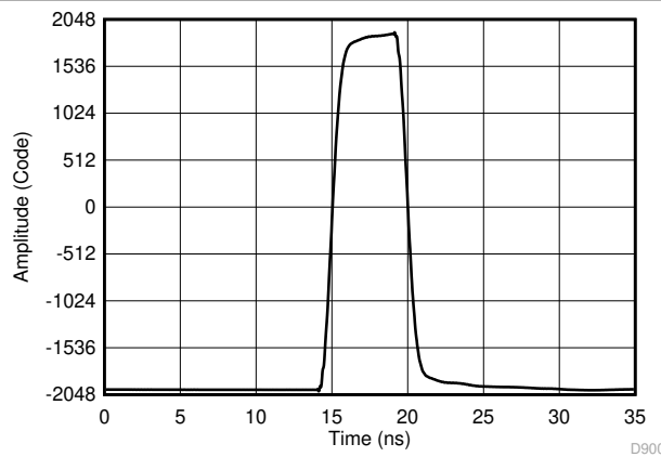
图 8-2. Measured Pulse using Sub-Sampling Technique for Equivalent 32 GSPS Measurement
