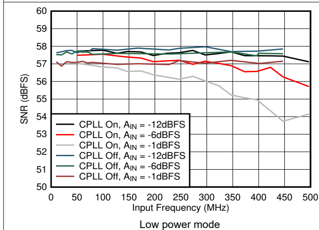
图 6-55. SNR vs A_{IN} and C-PLL
