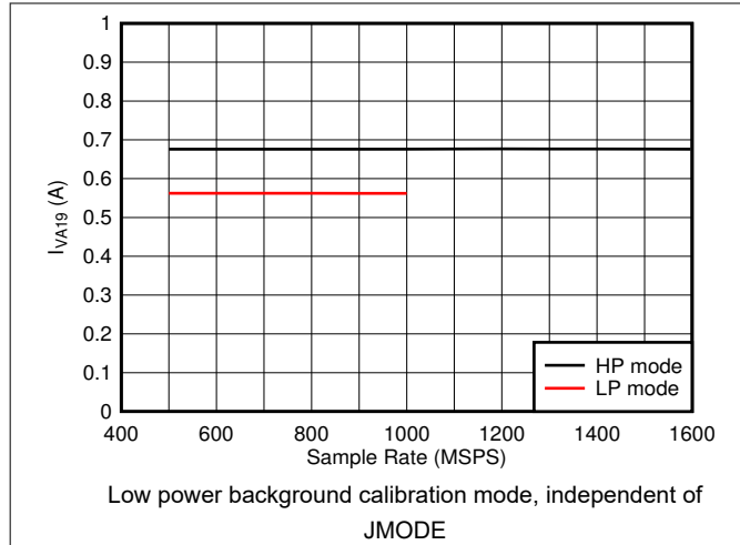
图 6-83. Quad Channel, I_{VA19} vs F_S
