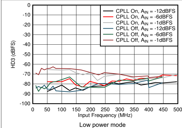
图 6-59. HD3 vs A_{IN} and C-PLL
