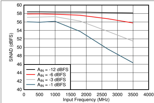
图 6-19. SINAD vs Input Frequency
