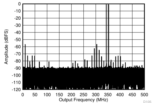
图 6-70. Two Tone FFT at 1798MHz
