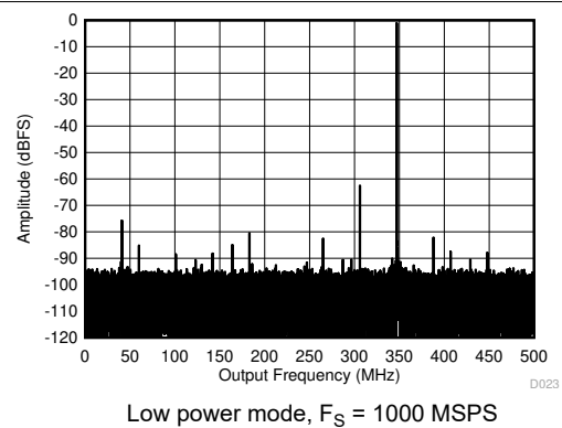
图 6-12. Single Tone FFT at 347 MHz and -1 dBFS
