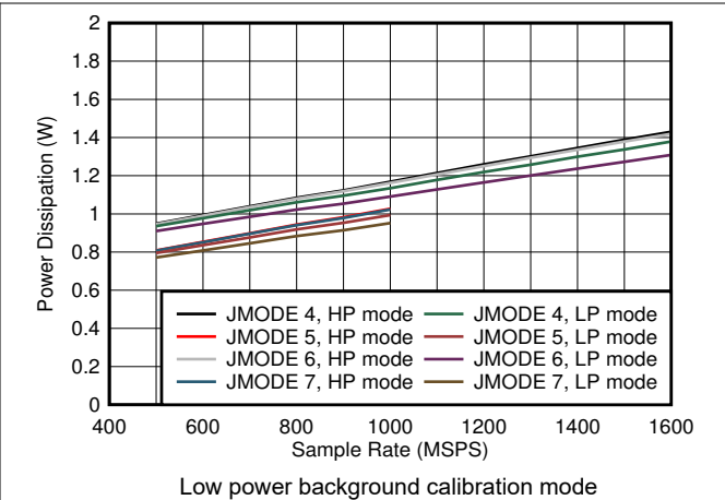
图 6-100. Single Channel, Power Dissipation vs F_S and JMODE 4 - 7
