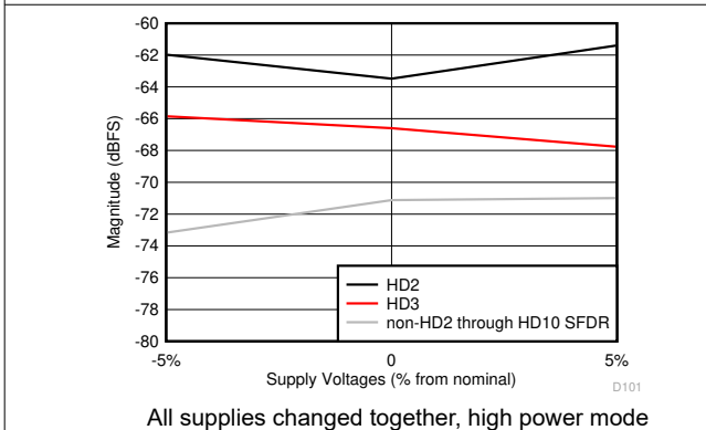
图 6-61. HD2, HD3 and Worst non-HD Spur vs Supply Voltage
