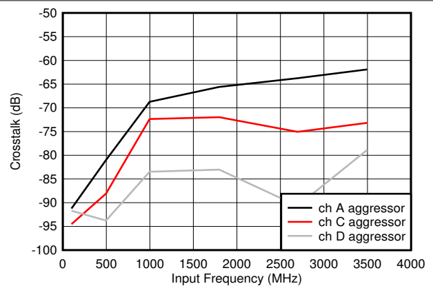
图 6-78. Crosstalk to Channel B vs F_{IN}
