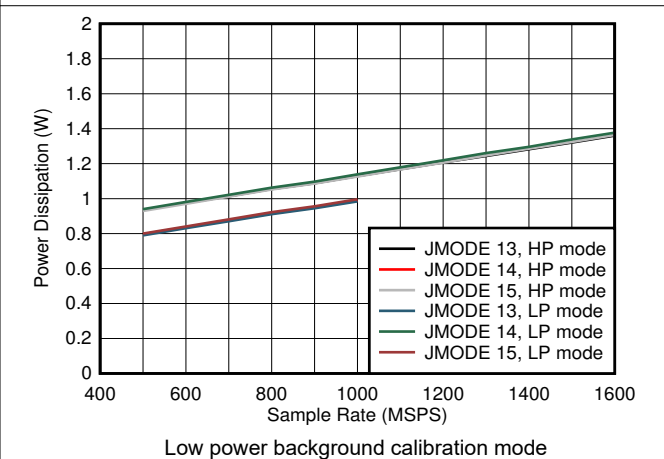
图 6-102. Single Channel, Power Dissipation vs F_S and JMODE 13 - 15
