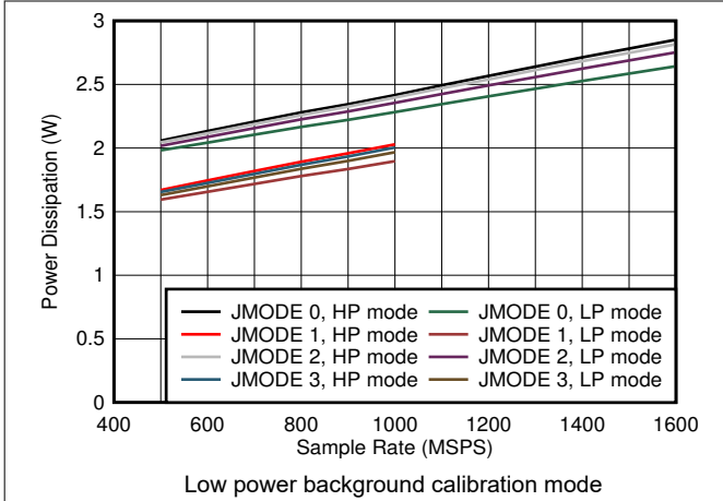
图 6-79. Quad Channel, Power Dissipation vs F_S and JMODES 0 - 3
