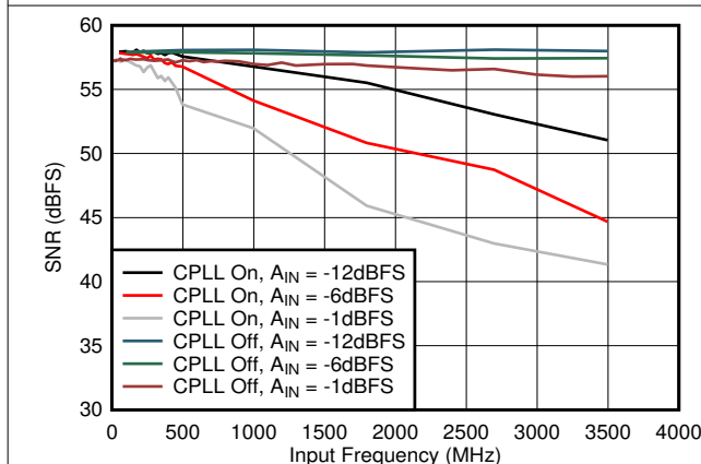
图 6-49. SNR vs A_{IN} and C-PLL
