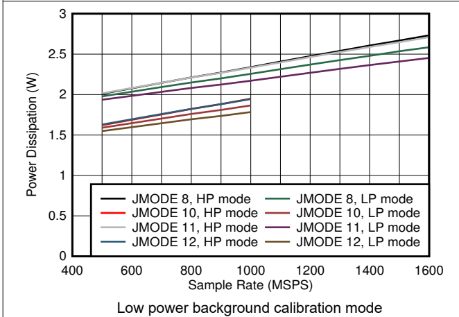
图 6-81. Quad Channel, Power Dissipation vs F_S and JMODE 8 - 12
