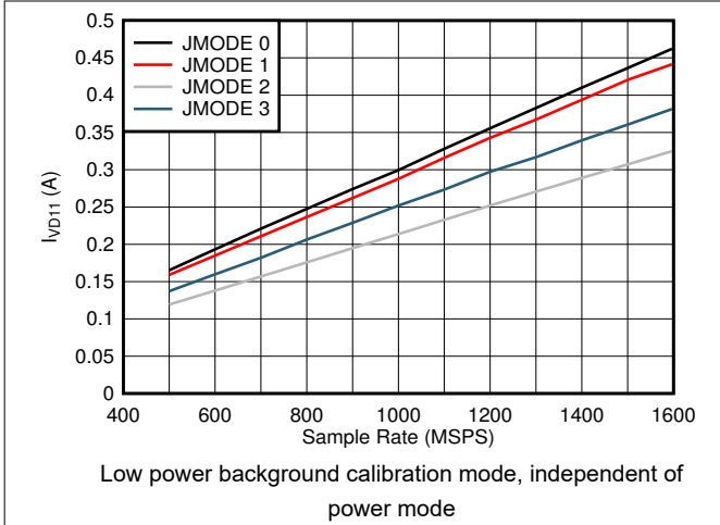
图 6-95. Dual Channel, Power Dissipation vs F_S and JMODE 0 - 3
