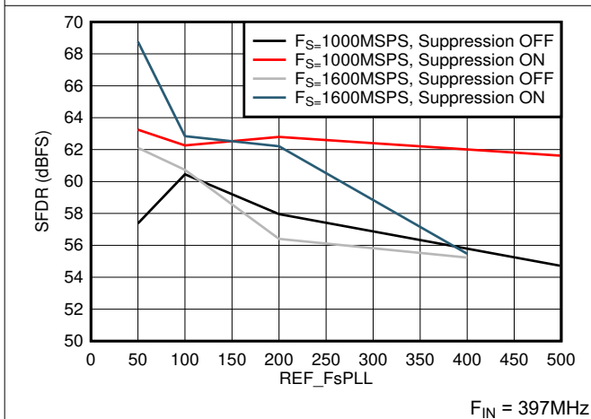
图 6-39. SFDR vs F_{REF} and Suppression
