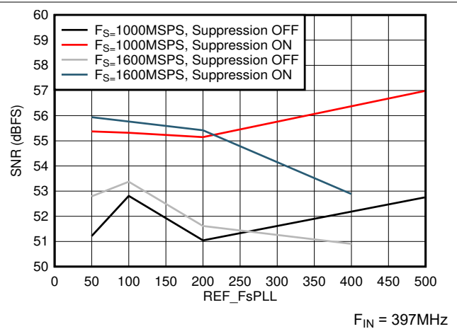
图 6-38. SNR vs F_{REF} and Suppression
