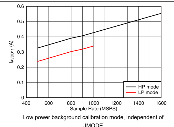
图 6-94. Dual Channel, I_{VA11} vs F_S
