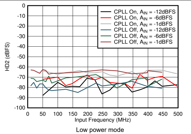
图 6-58. HD2 vs A_{IN} and C-PLL
