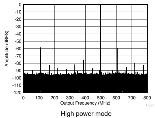
图 6-10. Single Tone FFT at 1797 MHz and -1 dBFS
