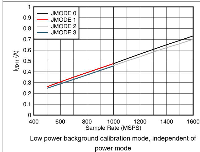
图 6-85. Quad Channel, I_{VD11} vs F_S and JMODE 0 - 3
