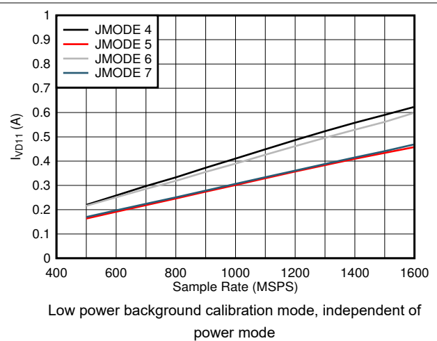
图 6-86. Quad Channel, I_{VD11} vs F_S and JMODE 4 - 7
