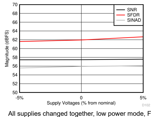
图 6-62. SNR, SFDR and SINAD vs Supply Voltages
