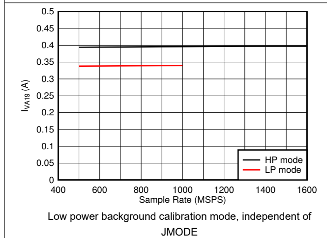
图 6-93. Dual Channel, I_{VA19} vs F_S
