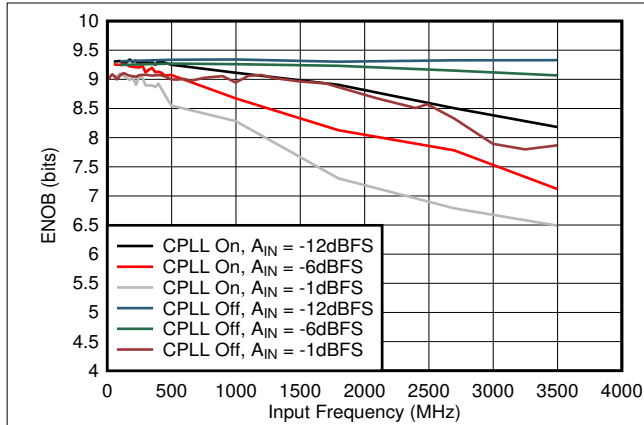
图 6-51. ENOB vs A_{IN} and C-PLL
