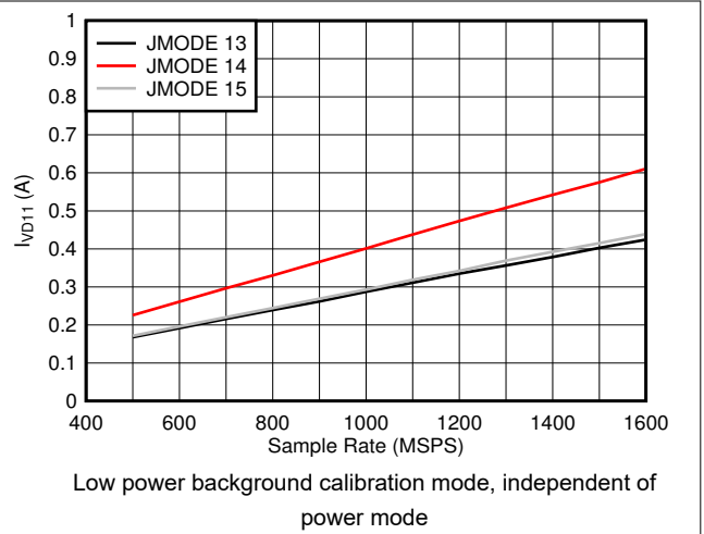
图 6-88. Quad Channel, I_{VD11} vs F_S and JMODE 13 - 15
