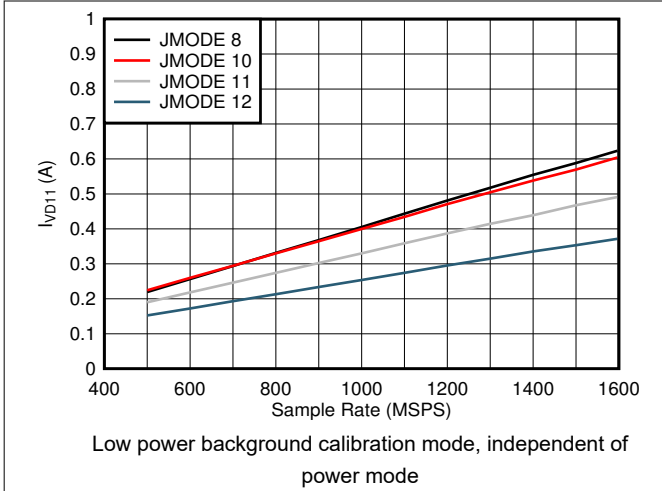
图 6-87. Quad Channel, I_{VD11} vs F_S and JMODE 8 - 12
