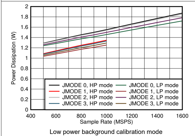
图 6-89. Dual Channel, Power Dissipation vs F_S and JMODE 0 - 3
