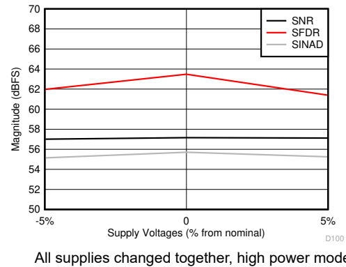
图 6-60. SNR, SFDR and SINAD vs Supply Voltage
