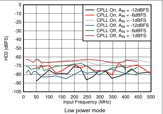
图 5-58. HD2 vs A_{IN} and C-PLL
