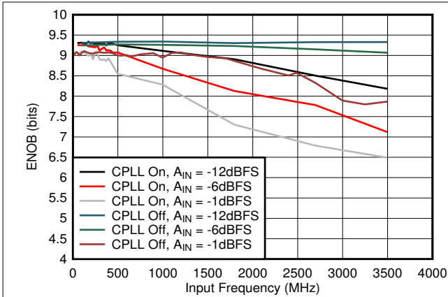
图 5-51. ENOB vs A_{IN} and C-PLL
