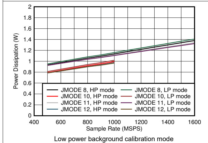
图 5-101. Single Channel, Power Dissipation vs F_S and JMODE 8 - 12
