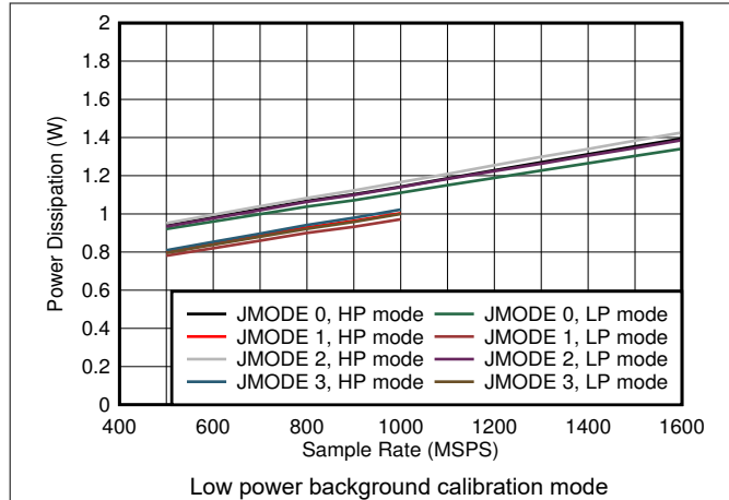
图 5-99. Single Channel, Power Dissipation vs F_S and JMODE 0 - 3
