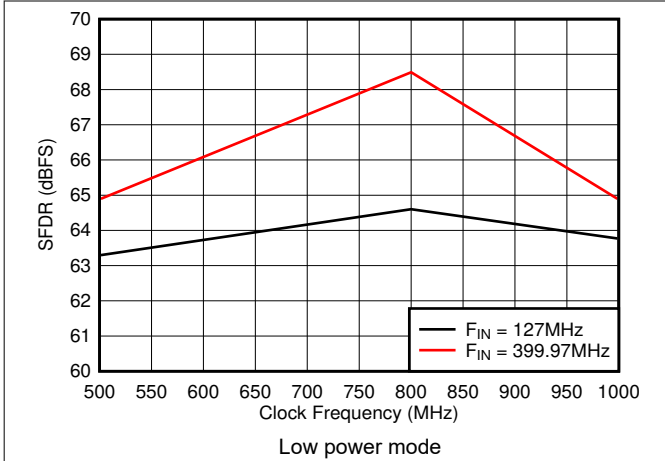
图 5-29. SFDR vs Sample Rate
