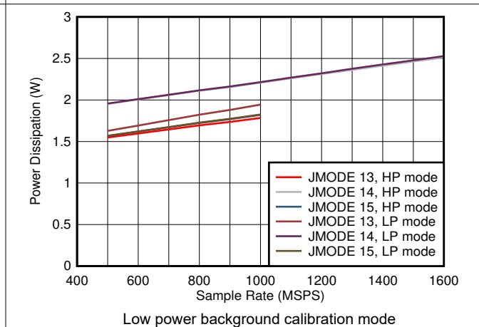
图 5-82. Quad Channel, Power Dissipation vs F_S and JMODE 13 - 15
