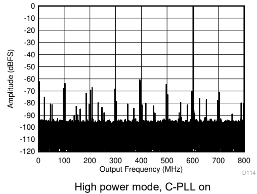
图 5-8. Single Tone FFT at 997 MHz and -1 dBFS
