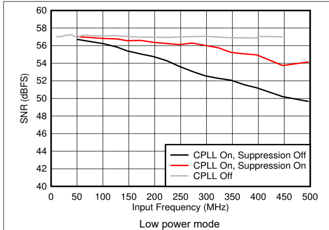
图 5-45. SNR vs F_{IN} and C-PLL modes
