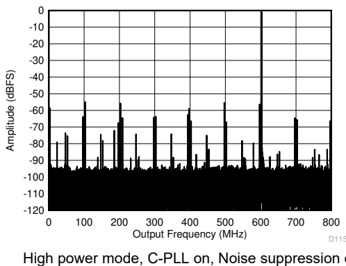
图 5-9. Single Tone FFT at 997 MHz and -1 dBFS
