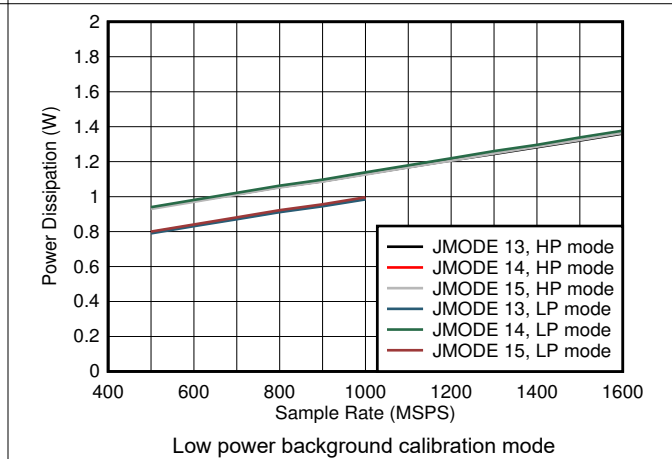
图 5-102. Single Channel, Power Dissipation vs F_S and JMODE 13 - 15
