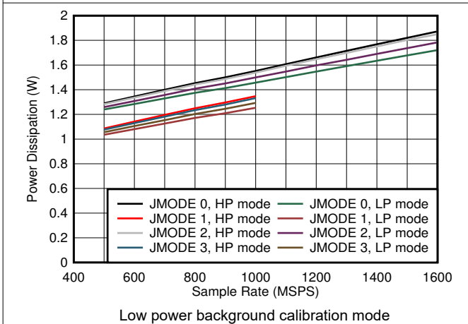
图 5-89. Dual Channel, Power Dissipation vs F_S and JMODE 0 - 3
