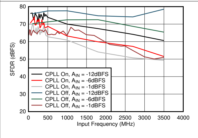
图 5-48. SFDR vs A_{IN} and C-PLL
