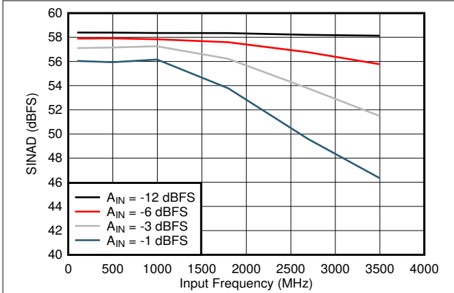
图 5-19. SINAD vs Input Frequency
