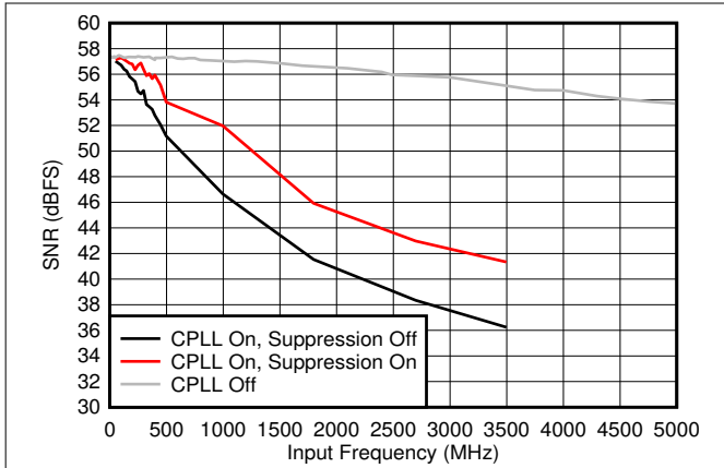
图 5-41. SNR vs F_{IN} and C-PLL modes
