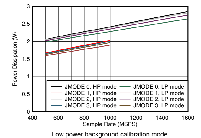
图 5-79. Quad Channel, Power Dissipation vs F_S and JMODES 0 - 3
