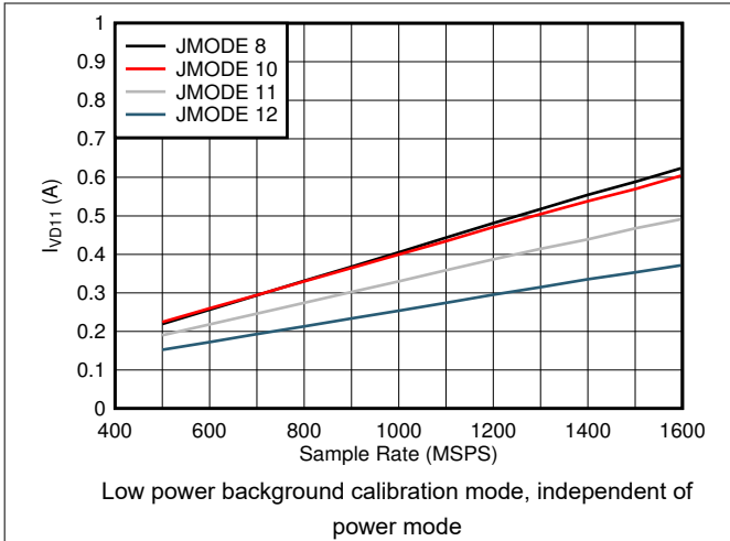
图 5-87. Quad Channel, I_{VD11} vs F_S and JMODE 8 - 12
