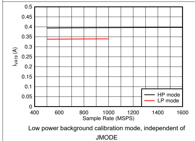
图 5-93. Dual Channel, I_{VA19} vs F_S
