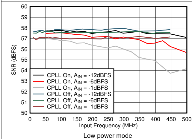
图 5-55. SNR vs A_{IN} and C-PLL
