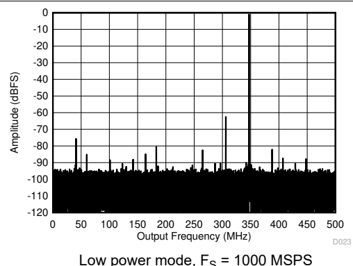
图 5-12. Single Tone FFT at 347 MHz and -1 dBFS
