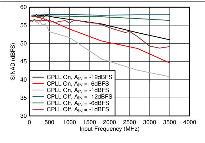
图 5-50. SINAD vs A_{IN} and C-PLL
