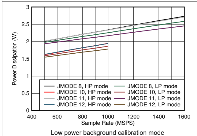
图 5-81. Quad Channel, Power Dissipation vs F_S and JMODE 8 - 12
