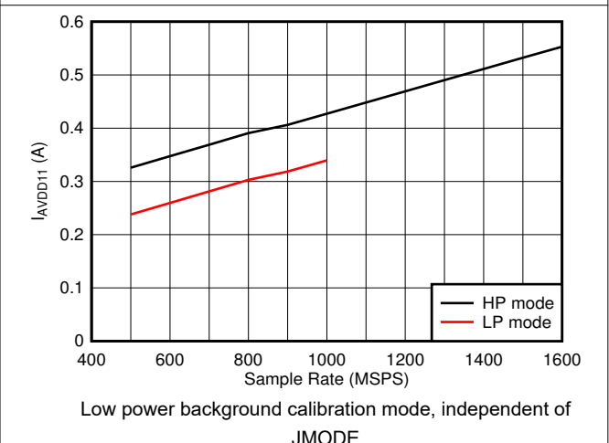
图 5-94. Dual Channel, I_{VA11} vs F_S
