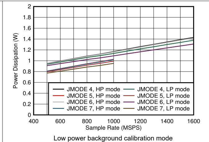
图 5-100. Single Channel, Power Dissipation vs F_S and JMODE 4 - 7
