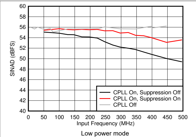
图 5-46. SINAD vs F_{IN} and C-PLL modes
