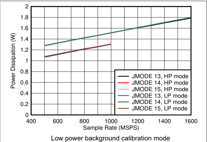
图 5-92. Dual Channel, Power Dissipation vs F_S and JMODE 13 - 15
