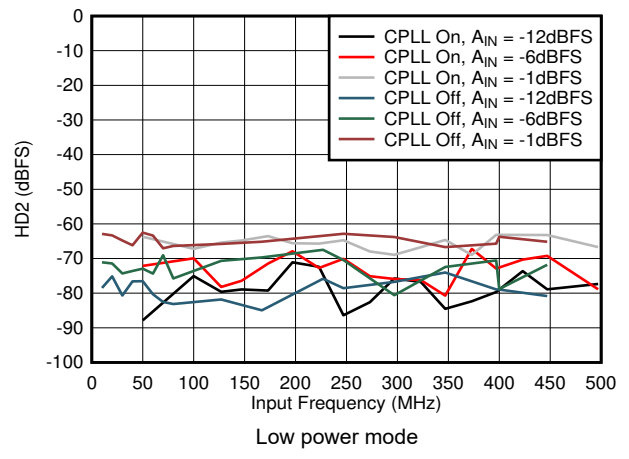
图 5-58. HD2 vs A_{IN} and C-PLL
