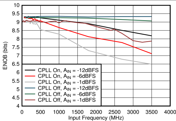
图 5-51. ENOB vs A_{IN} and C-PLL
