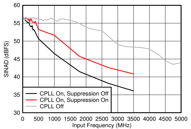
图 5-42. SINAD vs F IN and C-PLL modes
