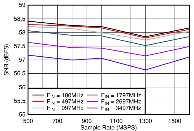
图 5-24. SNR vs Sample Rate
