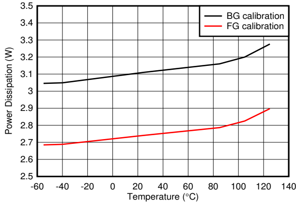
图 5-121. Quad Channel, Power Dissipation vs Temperature
