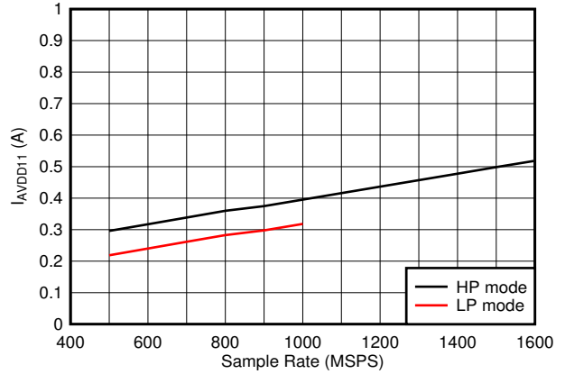
图 5-104. Single Channel, I_{VD11} vs F_S
