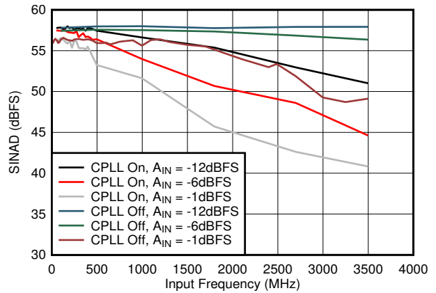
图 5-50. SINAD vs A_{IN} and C-PLL
