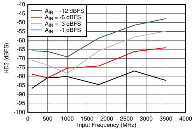
图 5-22. HD3 vs Input Frequency
