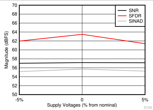
图 5-60. SNR, SFDR and SINAD vs Supply Voltage All supplies changed together, high power mode
