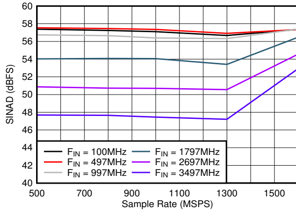
图 5-25. SINAD vs Sample Rate
