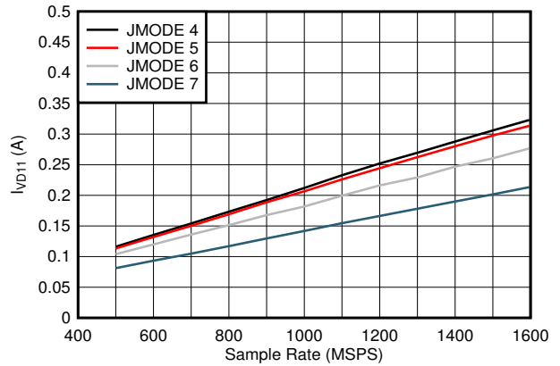
图 5-104. Single Channel, I_{VD11} vs F_S
