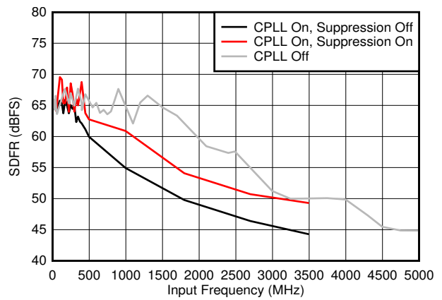
图 5-40. SFDR vs F IN and C-PLL modes
