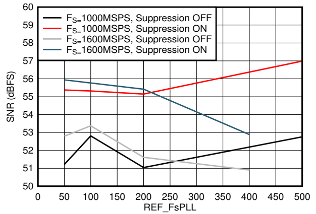
图 5-38. SNR vs F REF and Suppression
