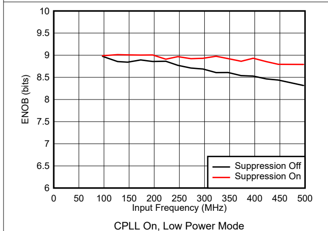
图 5-63. ENOB vs Input Frequency
