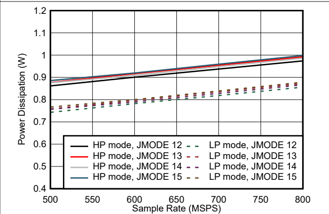
图 5-104. Single Channel, Power Dissipation vs F_S for JMODES 12 - 15
