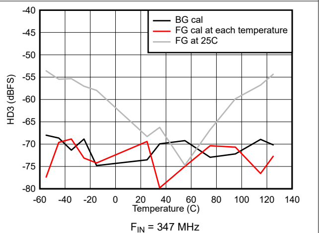
图 5-46. HD3 vs Temperature
