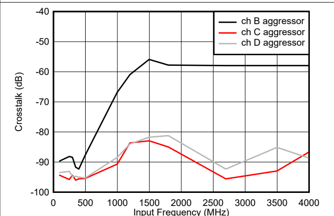
图 5-4. Crosstalk vs Input Frequency, Channel A victim
