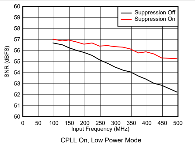
图 5-60. SNR vs Input Frequency
