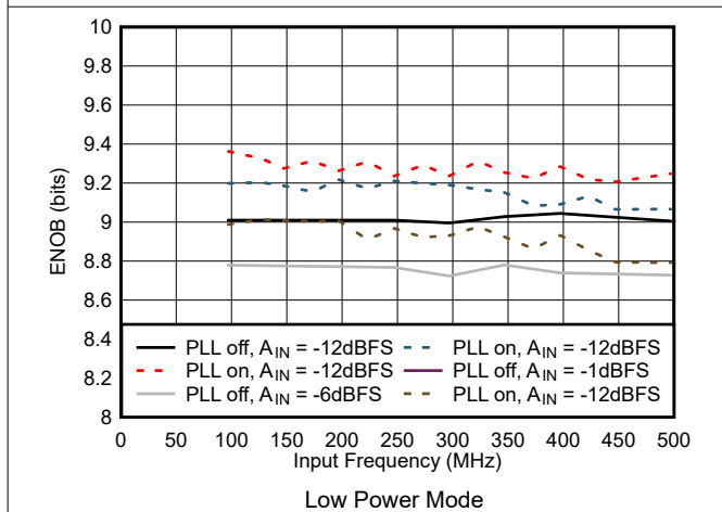
图 5-53. ENOB vs Input Frequency in Low Power Mode
