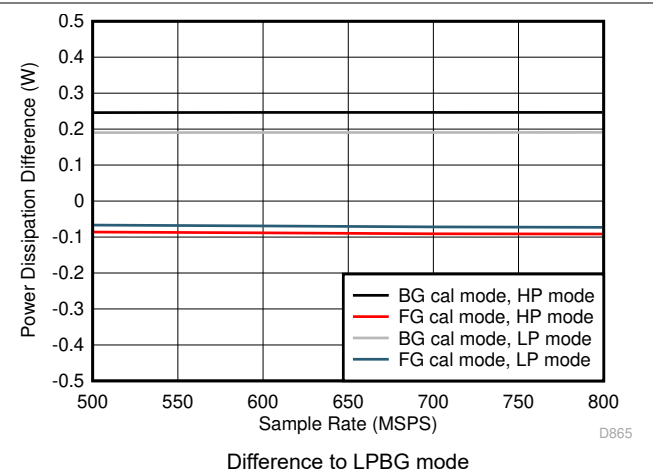
图 5-84. Quad Channel, Power Dissipation vs F_S over Modes
