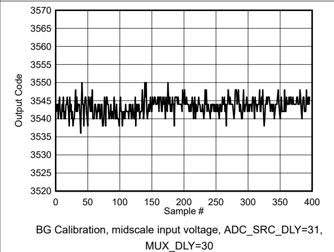
图 5-116. Background Calibration Core Transition (voltage offset)
