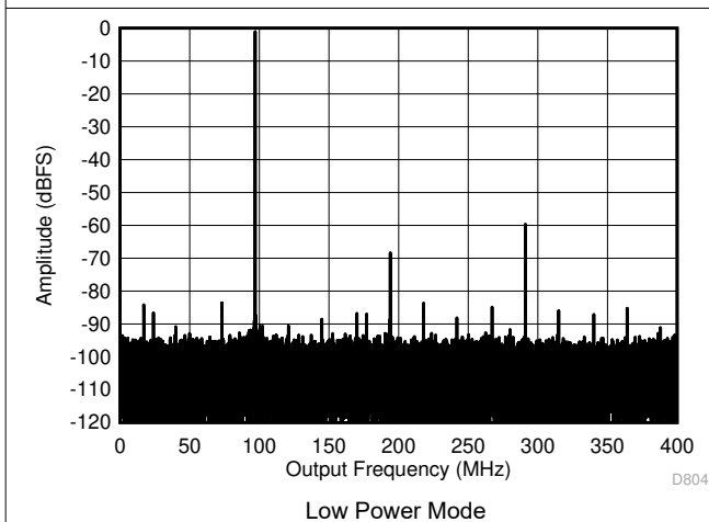
图 5-11. Single Tone FFT at 897 MHz and -1dBFS
