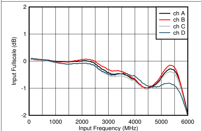
图 5-3. Input Fullscale vs Input Frequency
