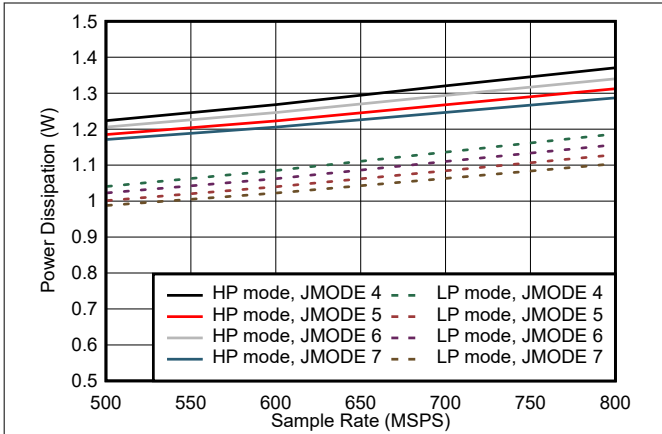
图 5-89. Dual Channel, Power Dissipation vs F_S for JMODES 4 - 7
