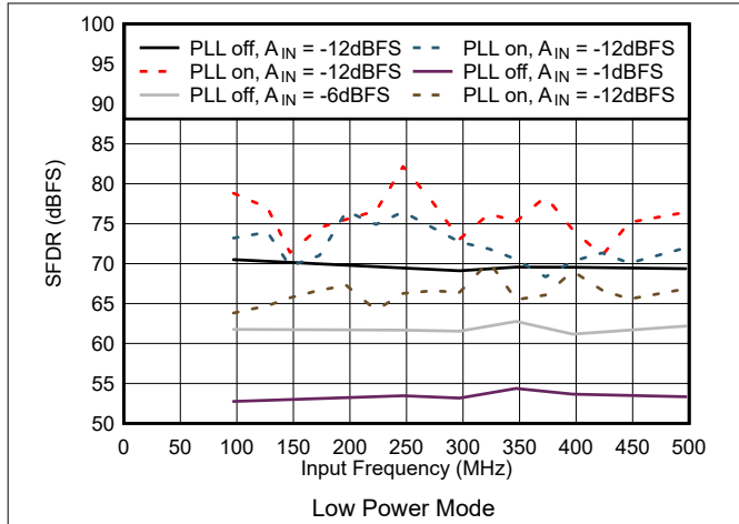
图 5-49. SFDR vs Input Frequency in Low Power Mode
