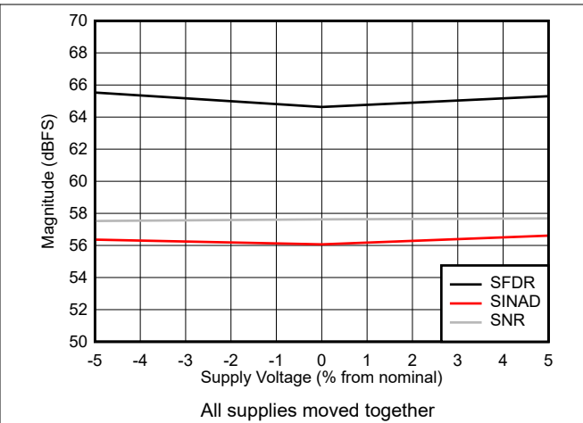
图 5-38. SNR, SFDR and SINAD vs Supply Voltage
