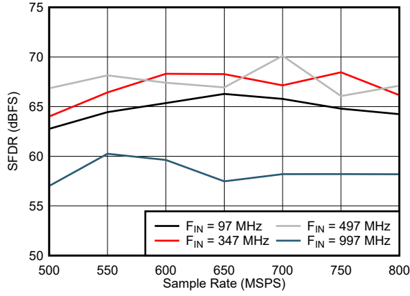
图 5-55. SFDR vs Sample Rate in Low Power Mode
