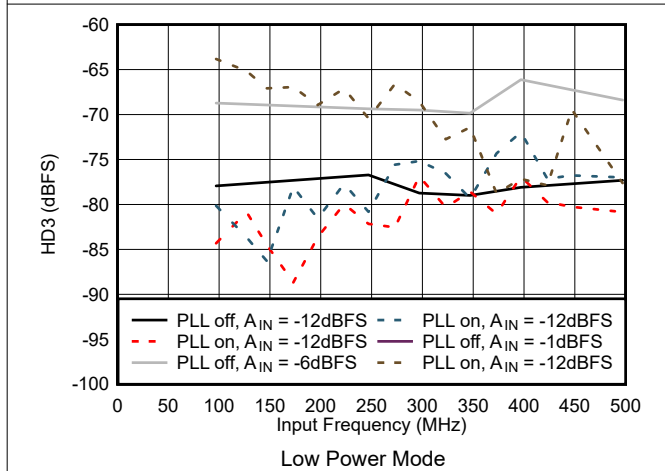
图 5-51. HD3 vs Input Frequency in Low Power Mode
