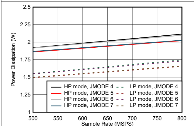
图 5-75. Quad Channel, Power Dissipation vs F_S for JMODES 4 - 7
