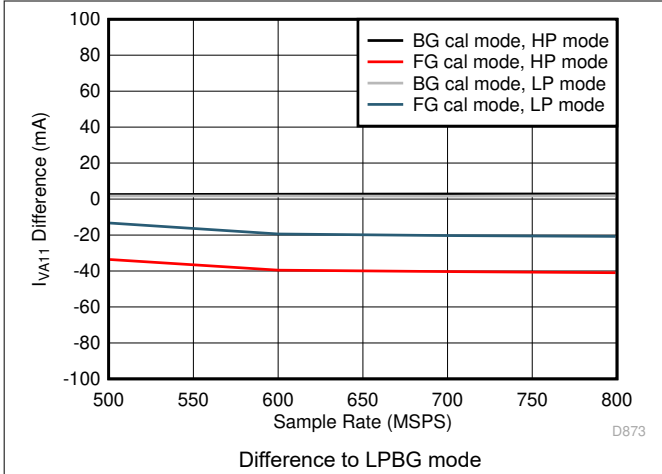
图 5-113. Single Channel, I_{VA11} vs F_S over Modes
