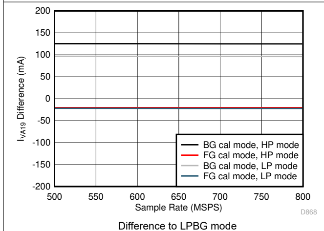
图 5-85. Quad Channel, I_{VA19} vs F_S over Modes
