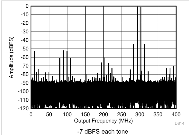
图 5-71. Two Tone FFT at 3498 MHz in Low Power Mode
