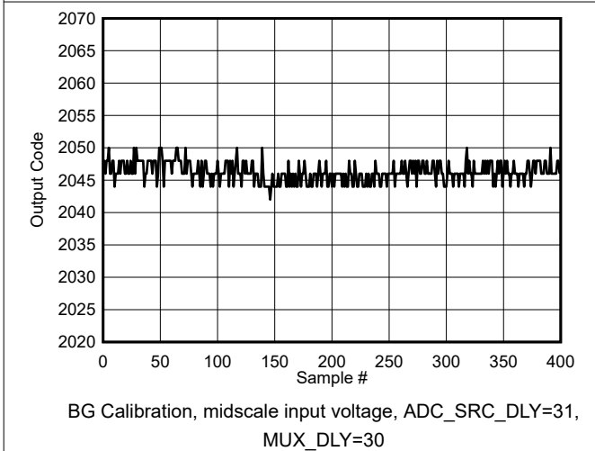
图 5-115. Background Calibration Core Transition (midscale)
