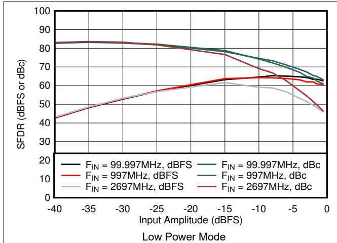
图 5-59. SFDR vs Input Amplitude in Low Power Mode
