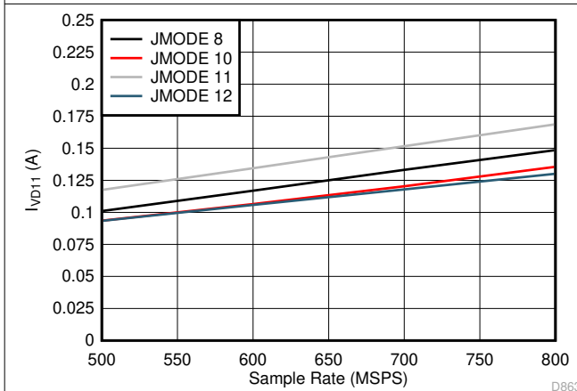
图 5-109. Single Channel, I_{VD11} vs F_S for JMODES 8 - 12
