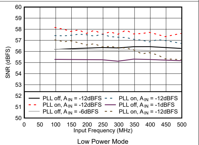
图 5-48. SNR vs Input Frequency in Low Power Mode
