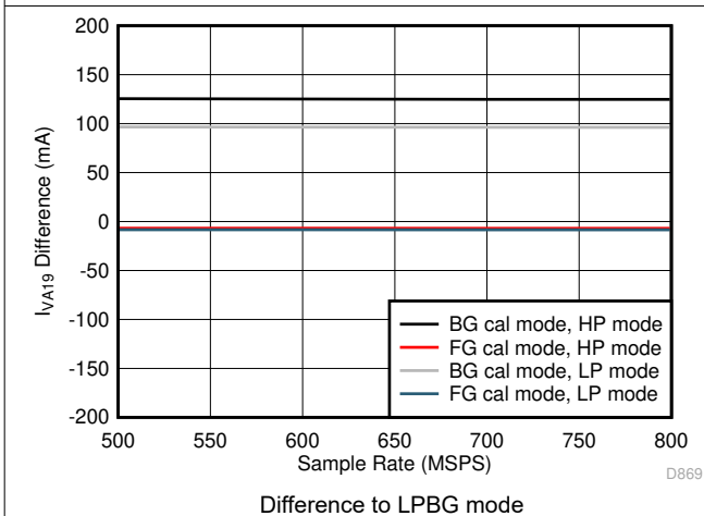
图 5-99. Dual Channel, I_{VA19} vs F_S over Modes
