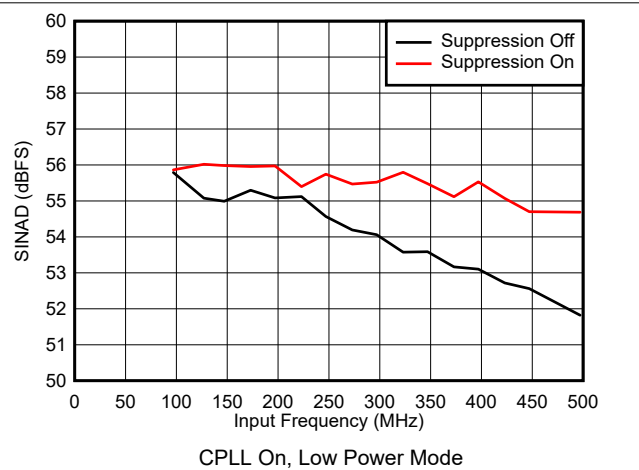
图 5-62. SINAD vs Input Frequency
