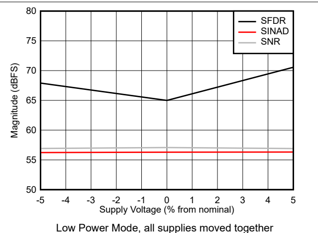
图 5-64. SNR, SFDR and SINAD vs Supply Voltage
