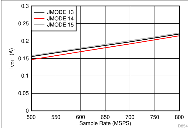
图 5-97. Dual Channel, I_{VD11} vs F_S for JMODES 13 - 15
