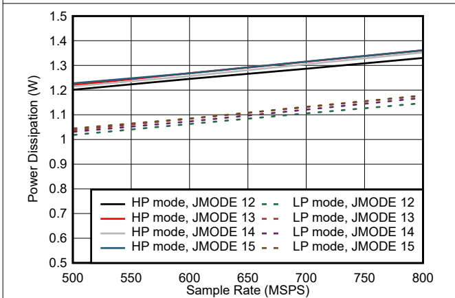
图 5-91. Dual Channel, Power Dissipation vs F_S for JMODES 12 - 15
