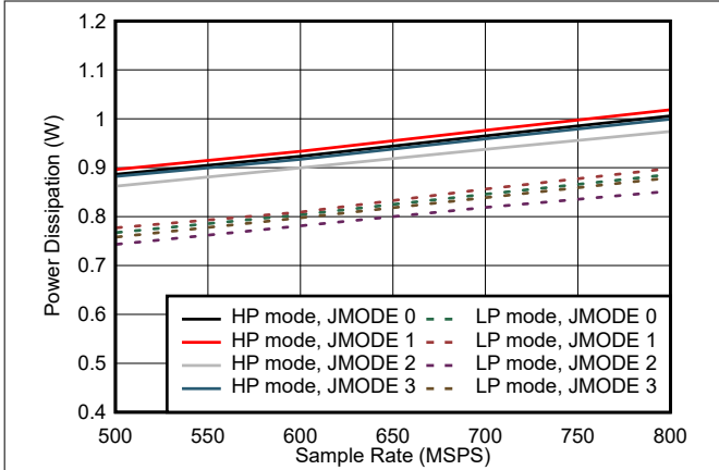
图 5-101. Dual Channel, Power Dissipation vs F_S for JMODES 0 - 3
