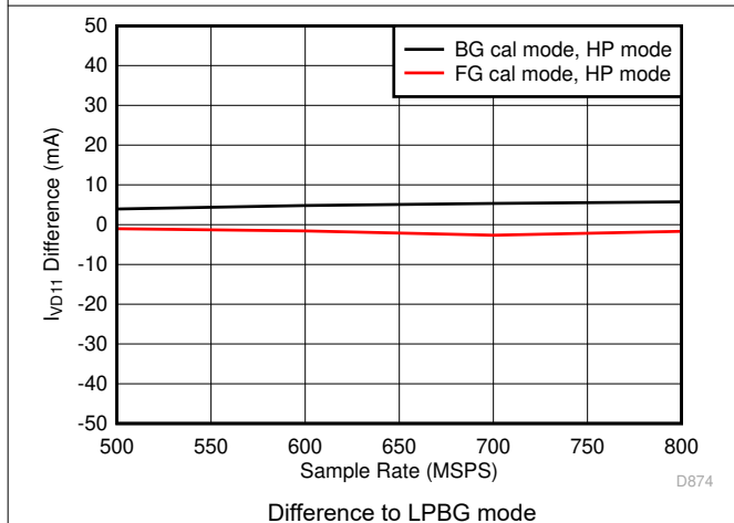
图 5-87. Quad Channel, I_{VD11} vs F_S over Modes
