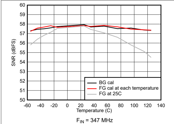
图 5-43. SNR vs Temperature
