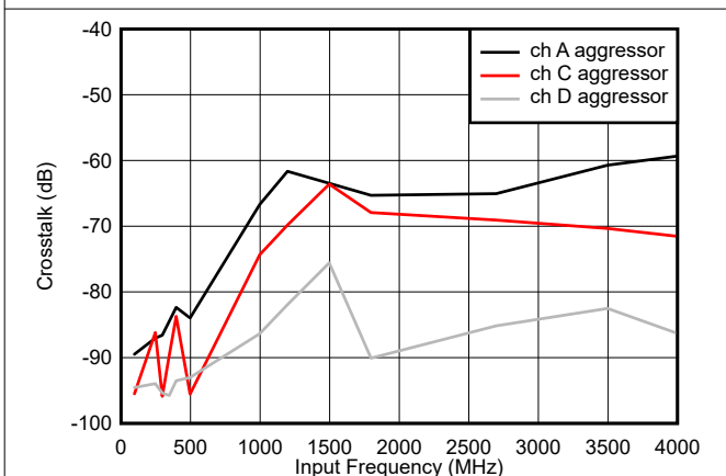
图 5-5. Crosstalk vs Input Frequency, Channel B victim
