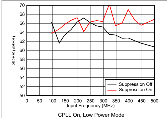
图 5-61. SFDR vs Input Frequency
