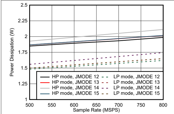
图 5-77. Quad Channel, Power Dissipation vs F_S for JMODES 12 - 15
