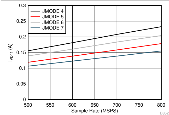
图 5-95. Dual Channel, I_{VD11} vs F_S for JMODES 4 - 7
