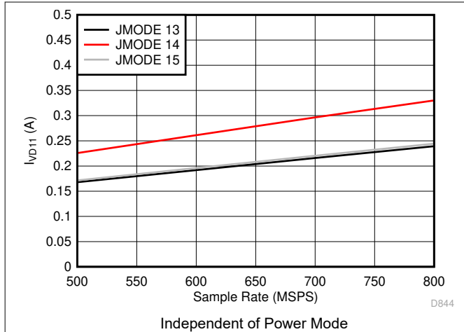
图 5-83. Quad Channel, I_{VD11} vs F_S for JMODES 13-15
