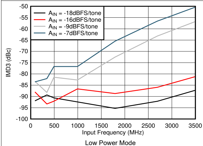
图 5-73. IMD3 vs Input Frequency in Low Power Mode
