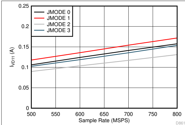
图 5-107. Single Channel, I_{VD11} vs F_S for JMODES 0 - 3
