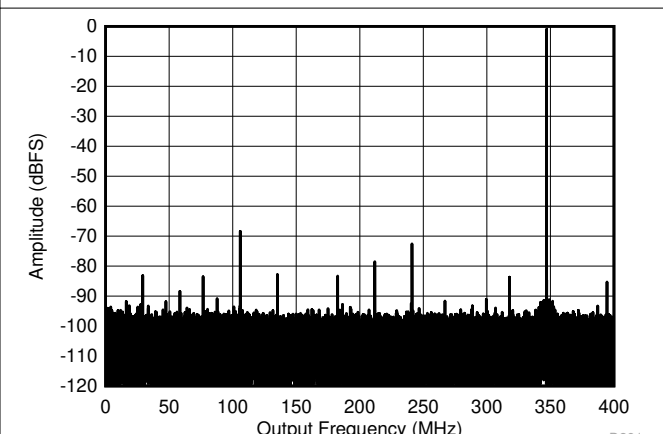
图 5-6. Single Tone FFT at 347 MHz and -1dBFS
