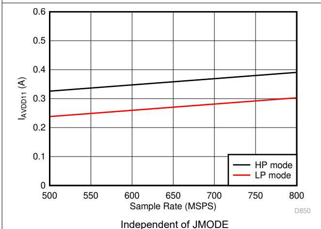
图 5-93. Dual Channel, I_{VA11} vs F_S
