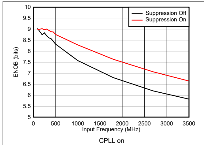
图 5-37. ENOB vs Input Frequency and Suppression
