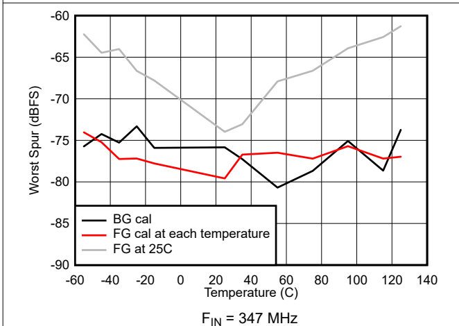
图 5-47. worst non-HD spur vs Temperature
