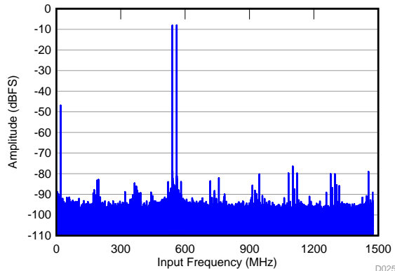
f_{IN1} = 3.49 \text{ MHz} , f_{IN2} = 3.51 \text{ GHz} , IMD = 75 dBFS, A_{IN} = -8 \text{ dBFS} with 2-dB gain
