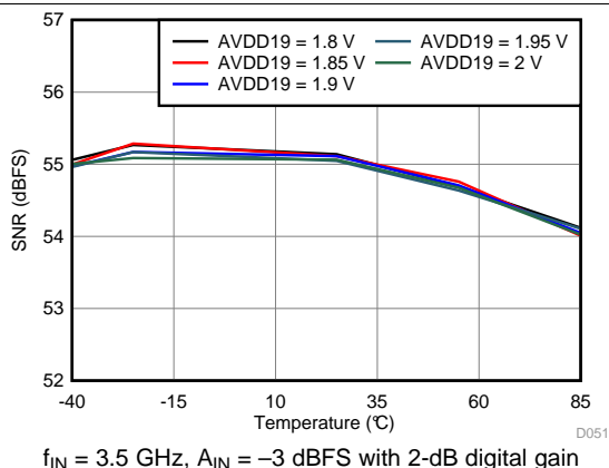
Figure 53. Signal-to-Noise Ratio vs AVDD19 Supply and Temperature
