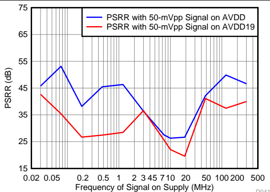
Figure 65. Power-Supply Rejection Ratio vs Tone Frequency
