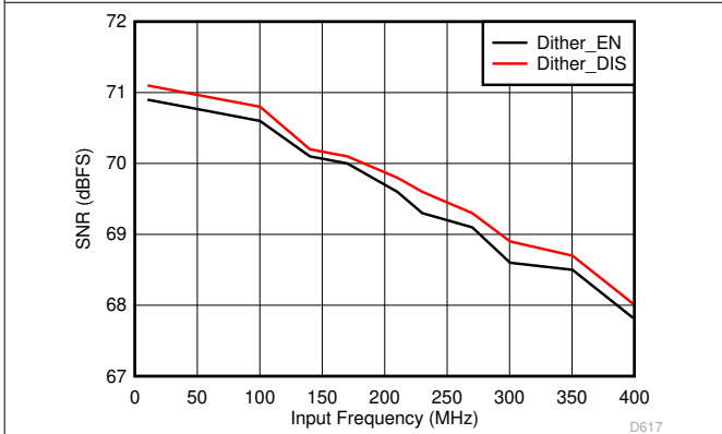
图 6-47. Signal-to-Noise Ratio vs Input Frequency
