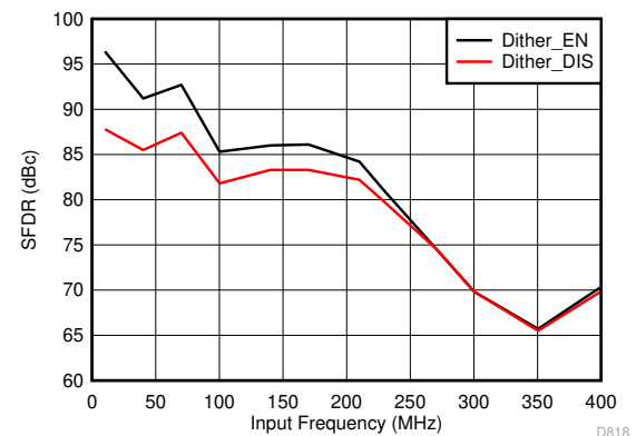
图 6-18. Spurious-Free Dynamic Range vs Input Frequency
