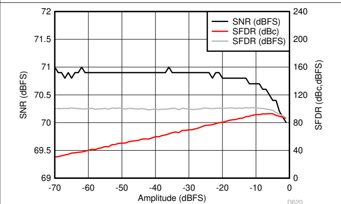
图 6-50. Performance vs Input Amplitude (170 MHz)
