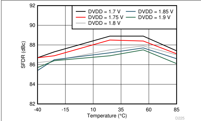
图 6-115. Spurious-Free Dynamic Range vs DVDD Supply and Temperature (170 MHz)
