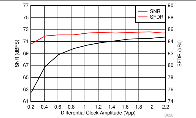
图 6-58. Performance vs Differential Clock Amplitude (150 MHz)
