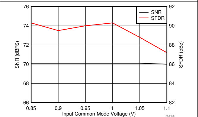
图 6-82. Performance vs Input Common-Mode Voltage (170 MHz)
