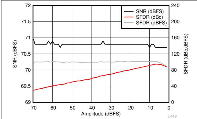
图 6-79. Performance vs Input Amplitude (30 MHz)
