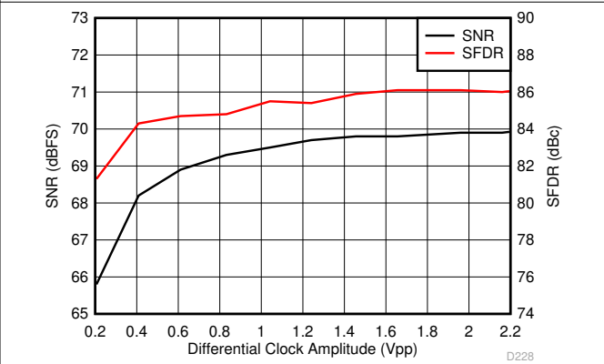
图 6-118. Performance vs Differential Clock Amplitude (150 MHz)
