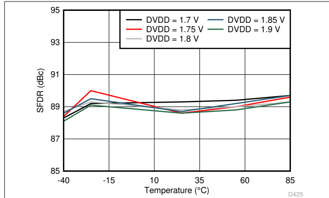
图 6-85. Spurious-Free Dynamic Range vs DVDD Supply and Temperature (170 MHz)
