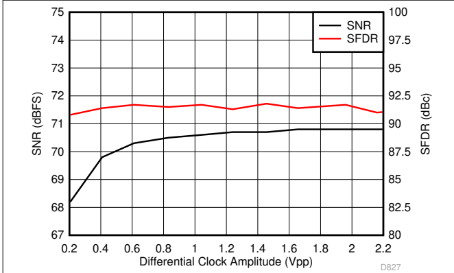
图 6-27. Performance vs Differential Clock Amplitude (40 MHz)
