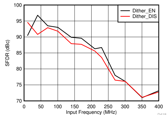
图 6-78. Spurious-Free Dynamic Range vs Input Frequency
