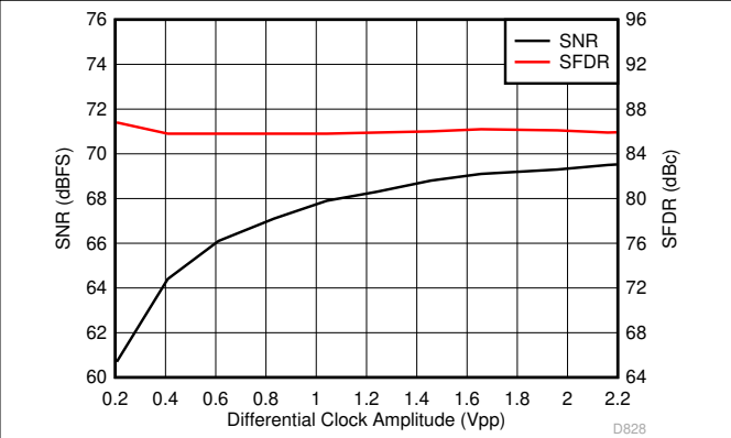
图 6-28. Performance vs Differential Clock Amplitude (150 MHz)
