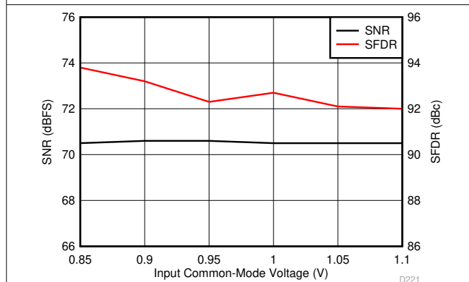
图 6-111. Performance vs Input Common-Mode Voltage (30 MHz)
