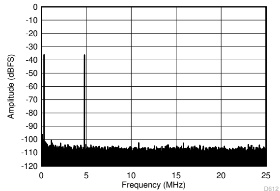
图 6-40. FFT for 450-MHz Input Signal (Dither Off)
