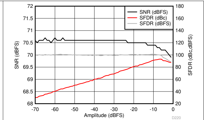
图 6-110. Performance vs Input Amplitude (170 MHz)
