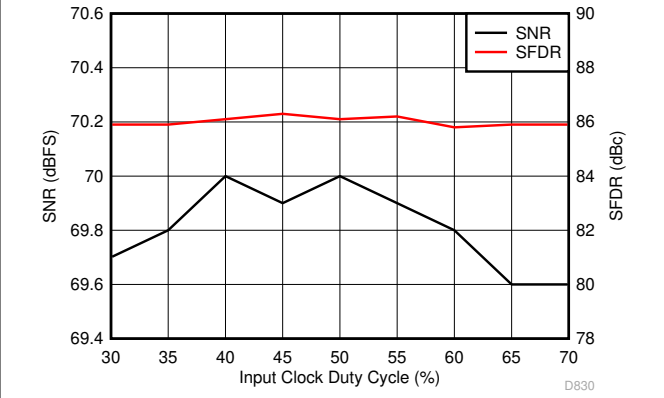
图 6-30. Performance vs Clock Duty Cycle (150 MHz)
