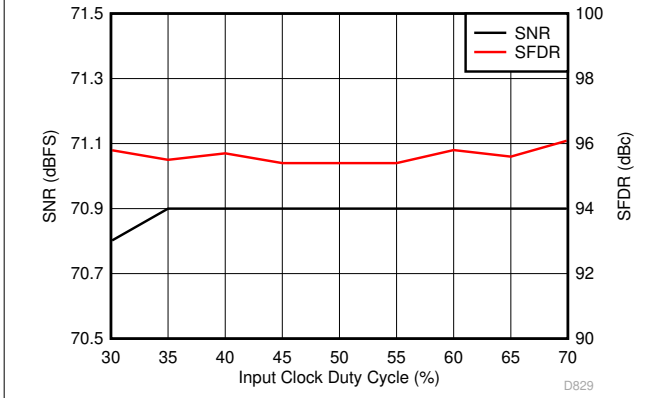
图 6-29. Performance vs Clock Duty Cycle (30 MHz)
