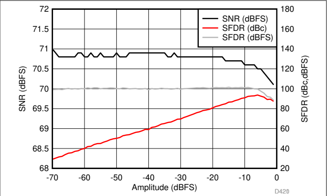
图 6-80. Performance vs Input Amplitude (170 MHz)
