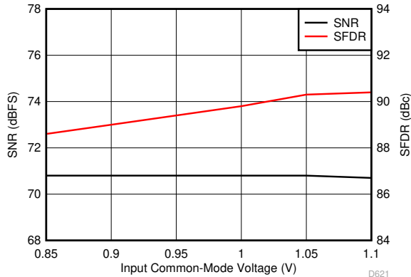
图 6-51. Performance vs Input Common-Mode Voltage (30 MHz)
