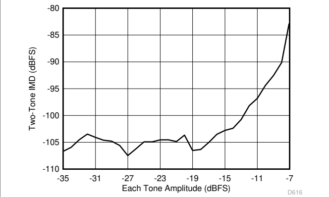
图 6-46. Intermodulation Distortion vs Input Amplitude (185 MHz and 190 MHz)
