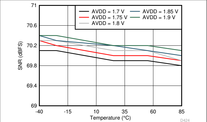
图 6-84. Signal-to-Noise Ratio vs AVDD Supply and Temperature (170 MHz)
