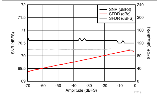
图 6-109. Performance vs Input Amplitude (30 MHz)
