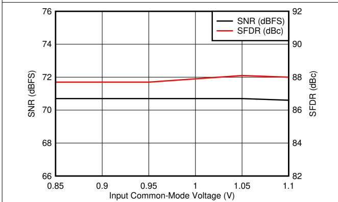
图 6-81. Performance vs Input Common-Mode Voltage (30 MHz)
