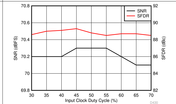
图 6-90. Performance vs Clock Duty Cycle (150 MHz)
