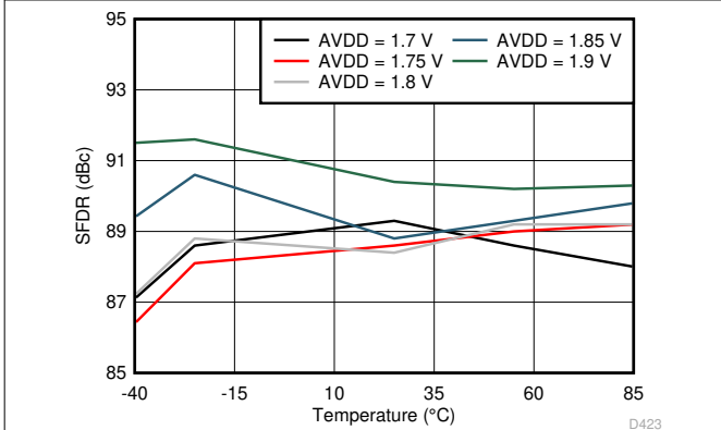
图 6-83. Spurious-Free Dynamic Range vs AVDD Supply and Temperature (170 MHz)
