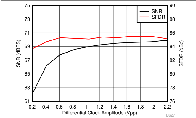
图 6-57. Performance vs Differential Clock Amplitude (40 MHz)
