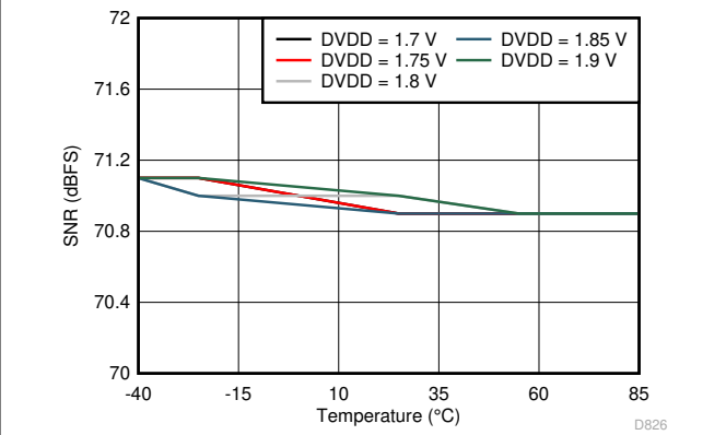
图 6-26. Signal-to-Noise Ratio vs DVDD Supply and Temperature (30 MHz)
