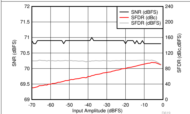
图 6-49. Performance vs Input Amplitude (30 MHz)
