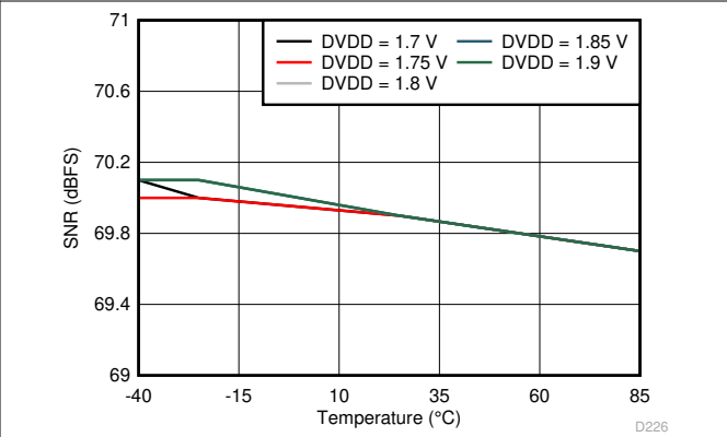
图 6-116. Signal-to-Noise Ratio vs DVDD Supply and Temperature (170 MHz)
