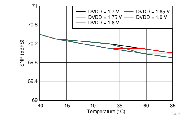
图 6-86. Signal-to-Noise Ratio vs DVDD Supply and Temperature (170 MHz)
