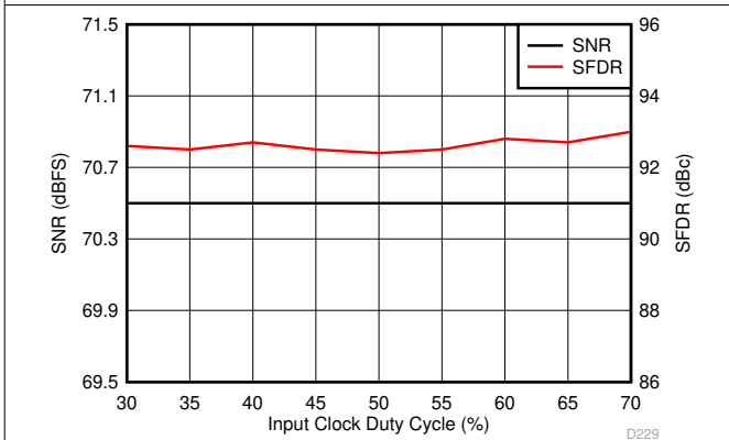
图 6-119. Performance vs Clock Duty Cycle (30 MHz)
