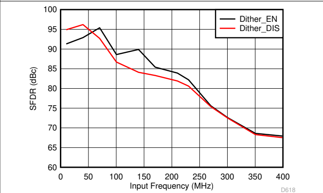
图 6-48. Spurious-Free Dynamic Range vs Input Frequency
