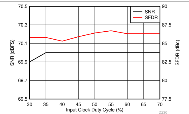
图 6-120. Performance vs Clock Duty Cycle (150 MHz)
