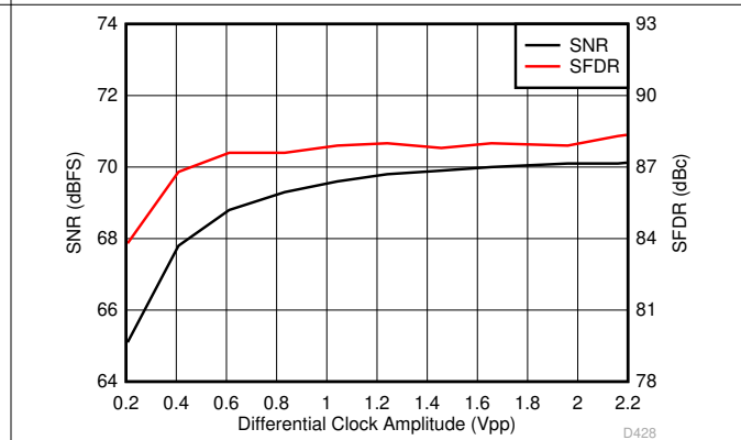
图 6-88. Performance vs Differential Clock Amplitude (150 MHz)
