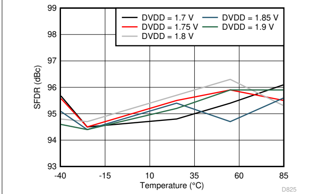
图 6-25. Spurious-Free Dynamic Range vs DVDD Supply and Temperature (30 MHz)
