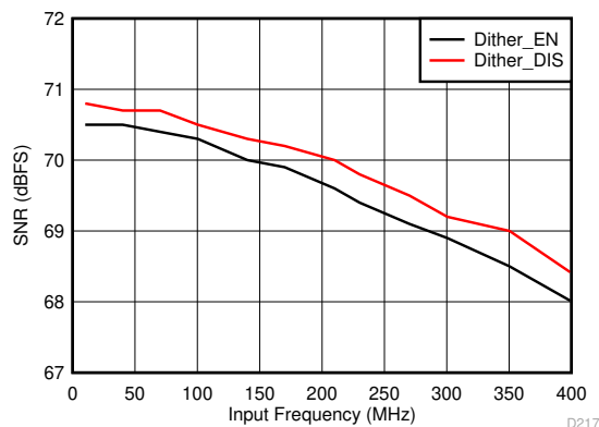
图 6-107. Signal-to-Noise Ratio vs Input Frequency
