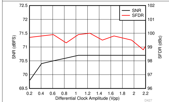
图 6-87. Performance vs Differential Clock Amplitude (40 MHz)
