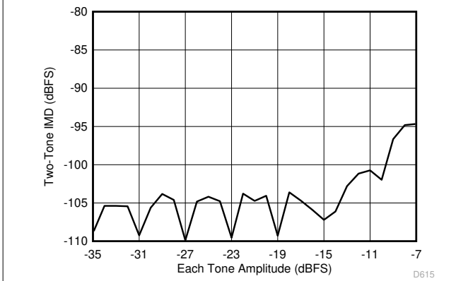
图 6-45. Intermodulation Distortion vs Input Amplitude (46 MHz and 50 MHz)
