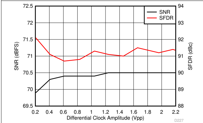
图 6-117. Performance vs Differential Clock Amplitude (40 MHz)
