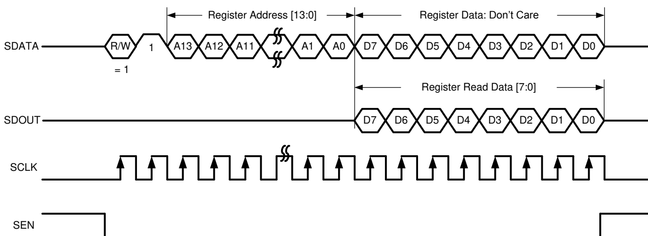
图 8-14. Serial Register Read Timing Diagram
