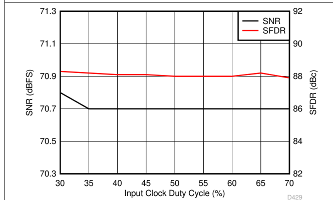
图 6-89. Performance vs Clock Duty Cycle (30 MHz)
