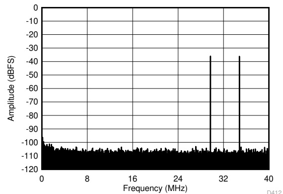
图 6-70. FFT for 450-MHz Input Signal (Dither Off)
