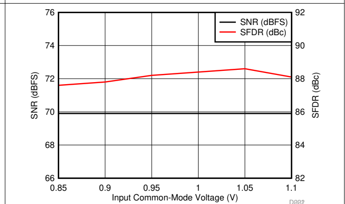
图 6-112. Performance vs Input Common-Mode Voltage (170 MHz)
