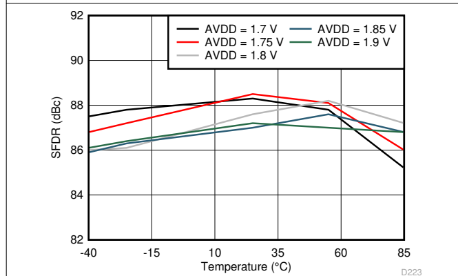
图 6-113. Spurious-Free Dynamic Range vs AVDD Supply and Temperature (170 MHz)
