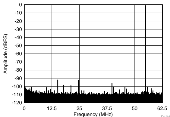
Figure 97. FFT for 70-MHz Input Signal (Dither Off) SFDR = 90.9 dBc, SNR = 73.3 dBFS, SINAD = 73.1 dBFS, THD = 87 dBc, HD2 = -90.9 dBc, HD3 = -94.9 dBc
