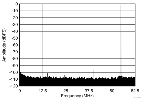
Figure 96. FFT for 70-MHz Input Signal (Dither On) SFDR = 95.9 dBc, SNR = 72.7 dBFS, SINAD = 72.7 dBFS, THD = 93.6 dBc, HD2 = -100.6 dBc, HD3 = -95.9 dBc
