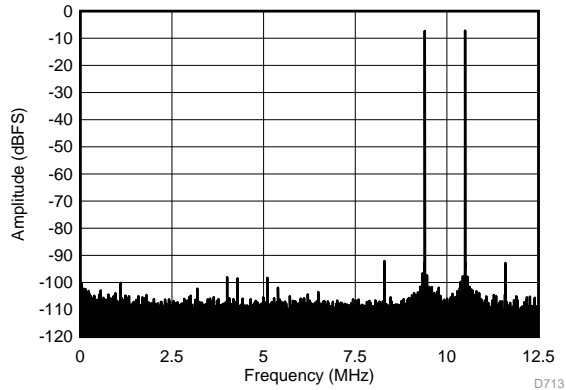
f_{IN1} = 185 \text{ MHz} , f_{IN2} = 190 \text{ MHz} , IMD3 = 78 dBFS, each tone at -7 dBFS
