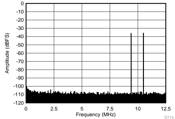
f_{IN1} = 185 \text{ MHz} , f_{IN2} = 190 \text{ MHz} , IMD3 = 89 dBFS, each tone at -36 dBFS
