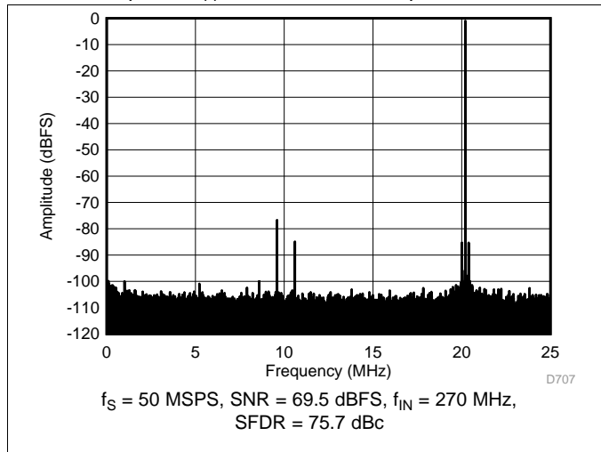
Figure 106. FFT for 270-MHz Input Signal (Dither On)
