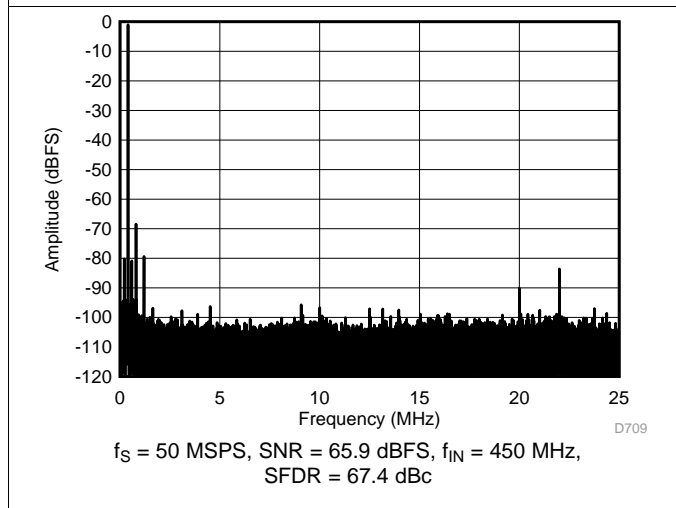
Figure 108. FFT for 450-MHz Input Signal (Dither On)
