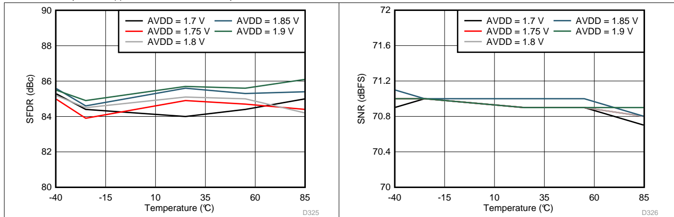
Figure 58. Spurious-Free Dynamic Range vs AVDD Supply and Temperature
