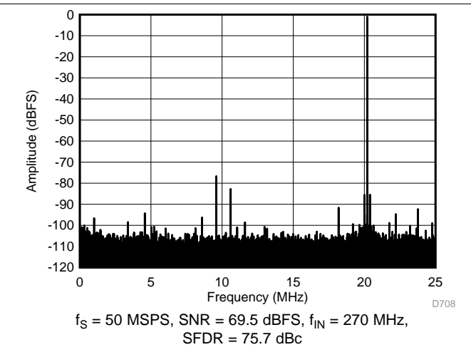
Figure 107. FFT for 270-MHz Input Signal (Dither Off)
