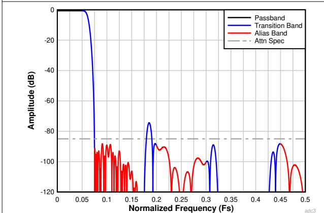
图 7-23. Complex Decimation by 8 Filter Response
