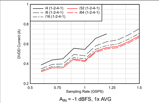
图 6-50. Current vs Sampling Rate vs Real Decimation
