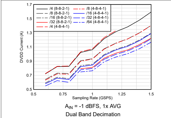
图 6-53. Current vs Sampling Rate vs Complex Decimation
