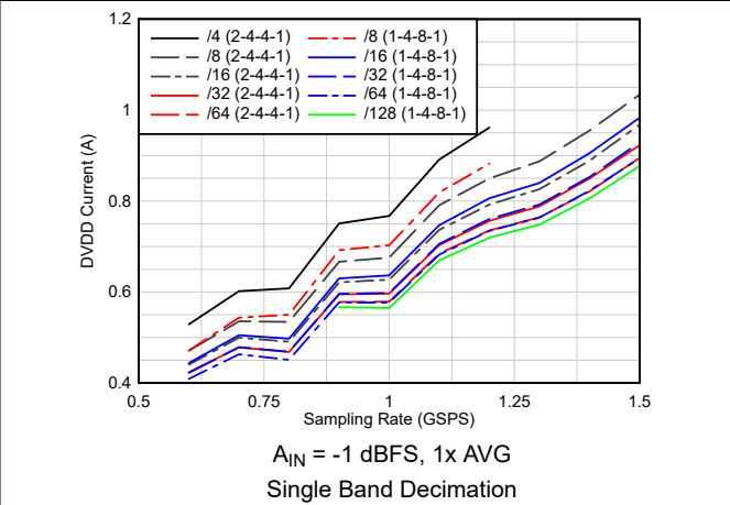
图 6-52. Current vs Sampling Rate vs Complex Decimation
