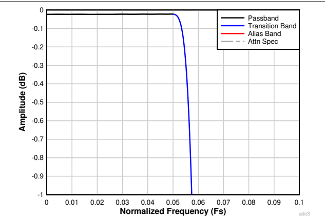
图 7-24. Decimation by 8 Passband Ripple Response
