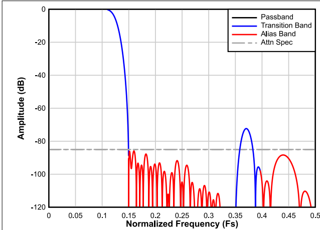
图 7-21. Complex Decimation by 4 Filter Response
