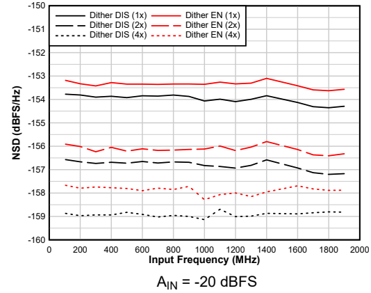
图 6-32. NSD Performance vs F_{IN}
