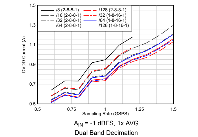
图 6-54. Current vs Sampling Rate vs Complex Decimation
