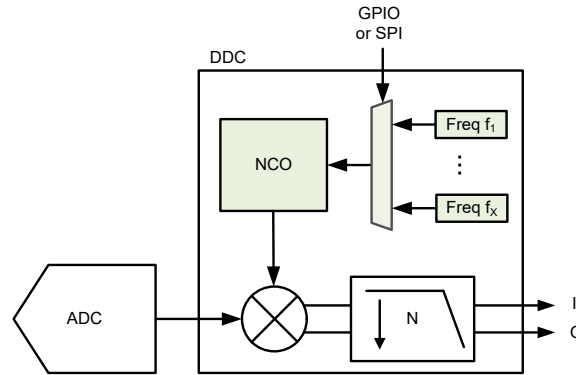
图 7-35. NCO Block Diagram
