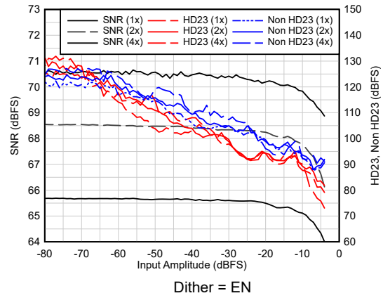
图 6-34. AC Performance vs A_{IN}
