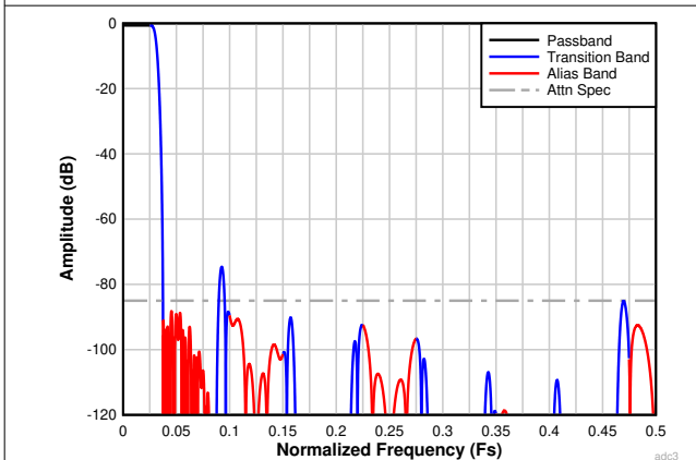
图 7-25. Complex Decimation by 16 Filter Response
