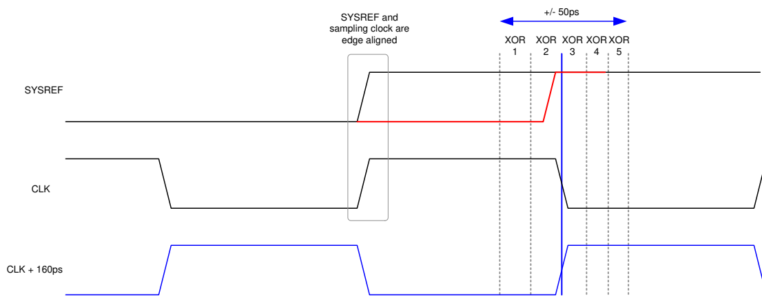
图 7-14. Detection of SYSREF Transition within Capture Window
