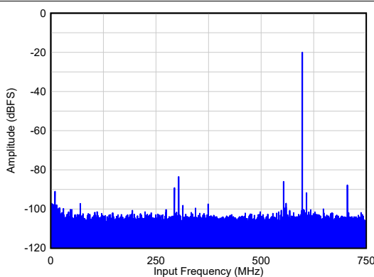
图 6-15. Single Tone FFT at F_{IN} = 900 MHz
