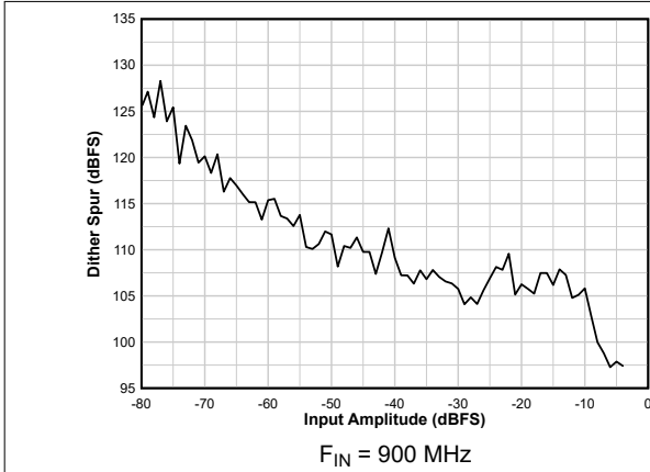
图 6-31. Dither Spur vs A_{IN}
