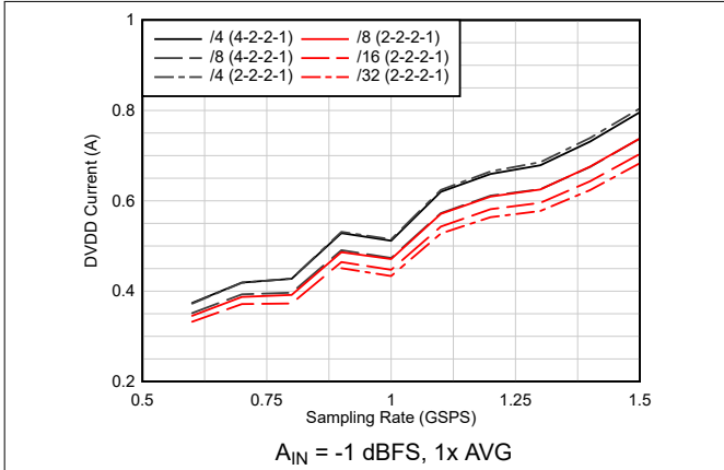
图 6-49. Current vs Sampling Rate vs Real Decimation
