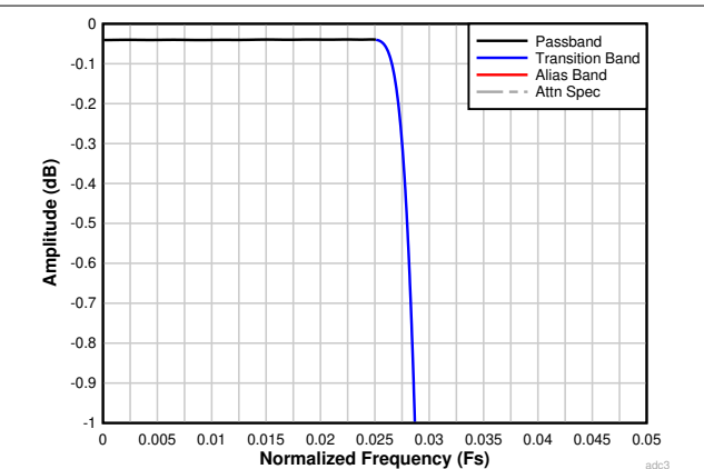
图 7-26. Decimation by 16 Passband Ripple Response
