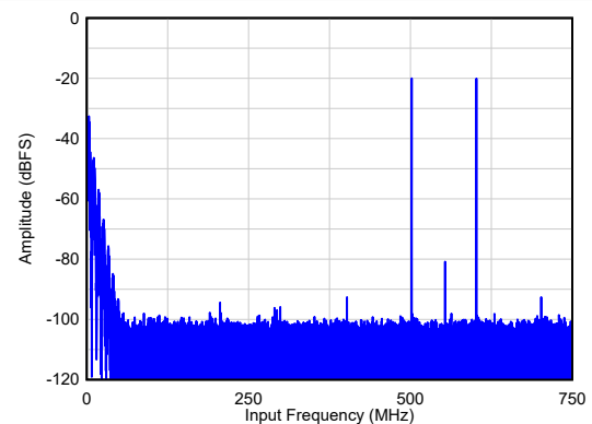
图 6-22. Two Tone FFT at F_{IN} = 900, 1000 MHz
