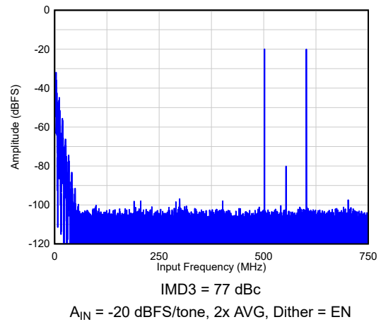
图 6-28. Two Tone FFT at F_{IN} = 900, 1000 MHz
