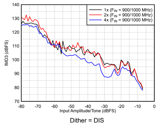
图 6-36. IMD3 Performance vs A_{IN}
