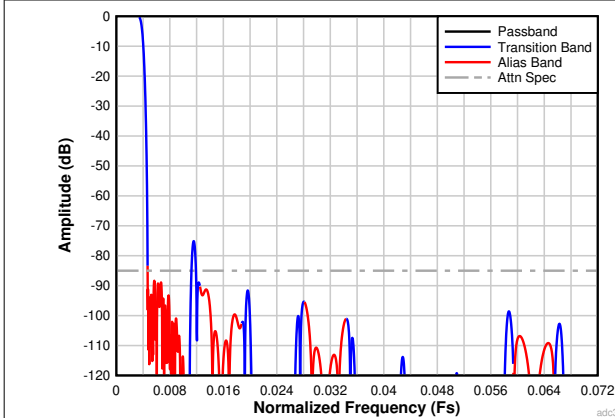
图 7-33. Complex Decimation by 128 Filter Response
