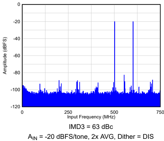
图 6-27. Two Tone FFT at F_{IN} = 900, 1000 MHz
