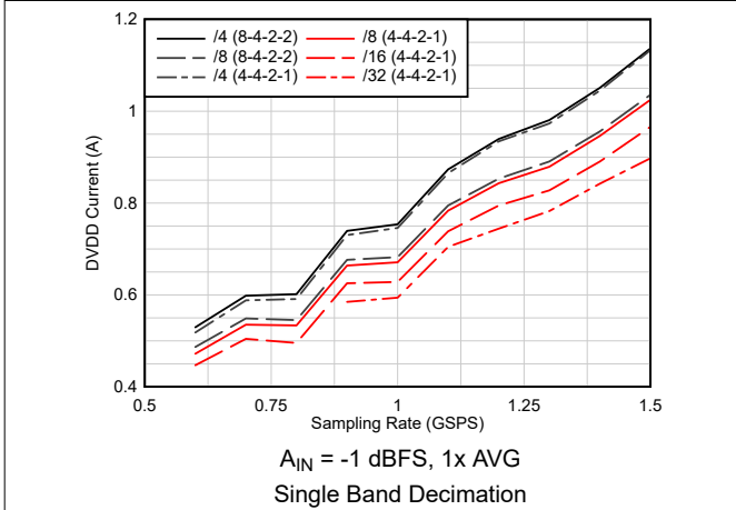
图 6-51. Current vs Sampling Rate vs Complex Decimation
