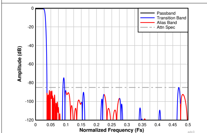
图 7-28. Complex Decimation by 16 Filter Response
