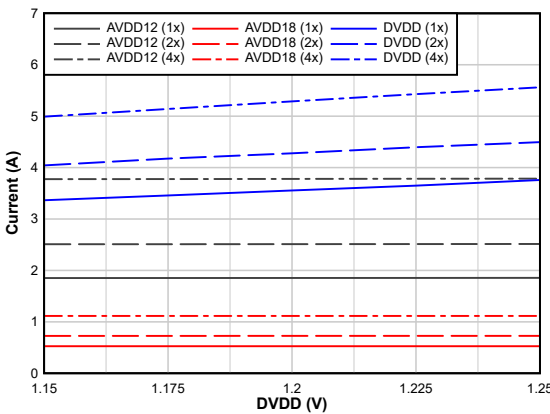
图 6-112. I_{DVDD} vs Supply A_{IN} = -1 dBFS, DDC Bypass
