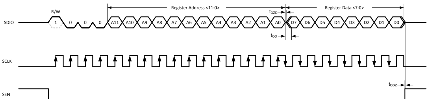
图 7-47. Serial Register Read Timing Diagram
