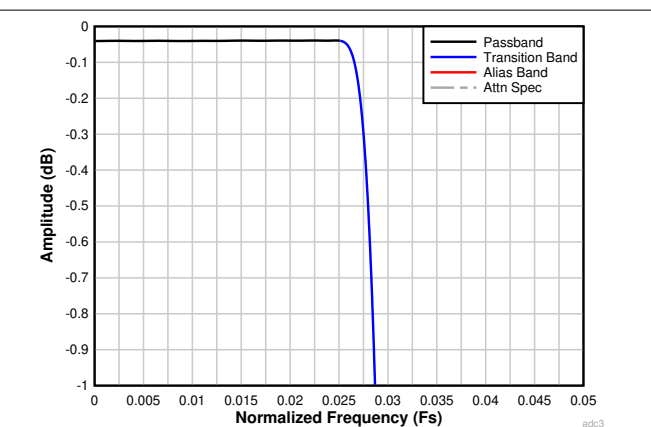
图 7-29. Decimation by 16 Passband Ripple Response
