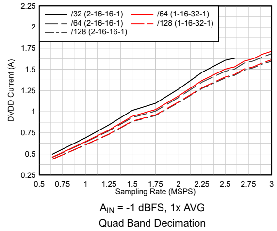
图 6-109. Current vs Sampling Rate vs Complex Decimation
