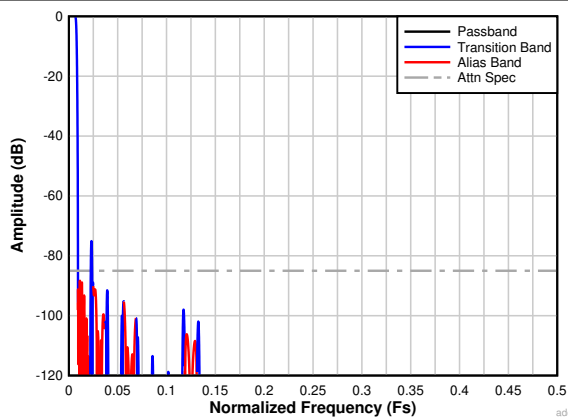
图 7-32. Complex Decimation by 64 Filter Response
