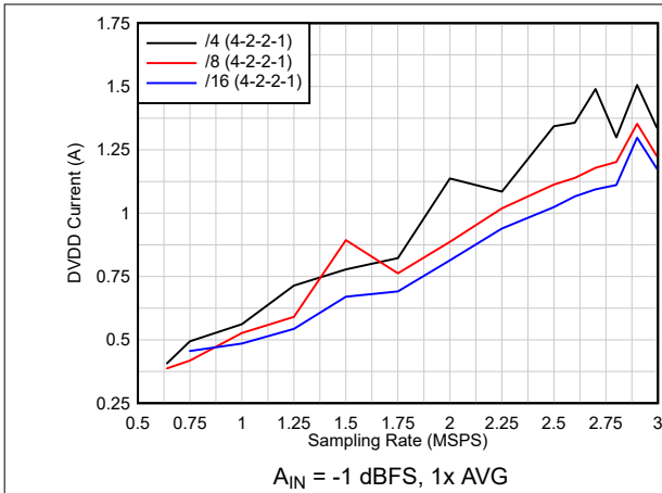
图 6-102. Current vs Sampling Rate vs Real Decimation
