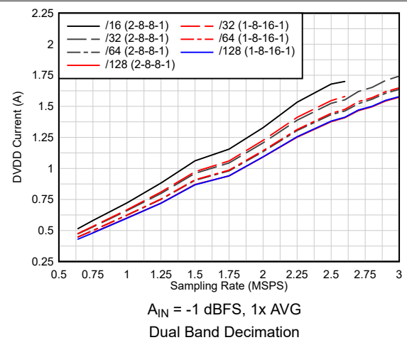
图 6-107. Current vs Sampling Rate vs Complex Decimation
