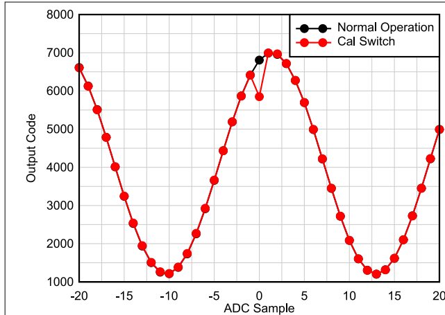
图 7-21. Output Code vs ADC Sample
