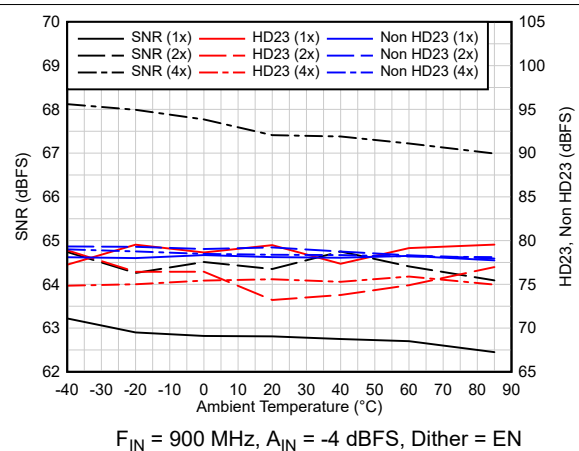
图 6-40. AC Performance vs Temperature
