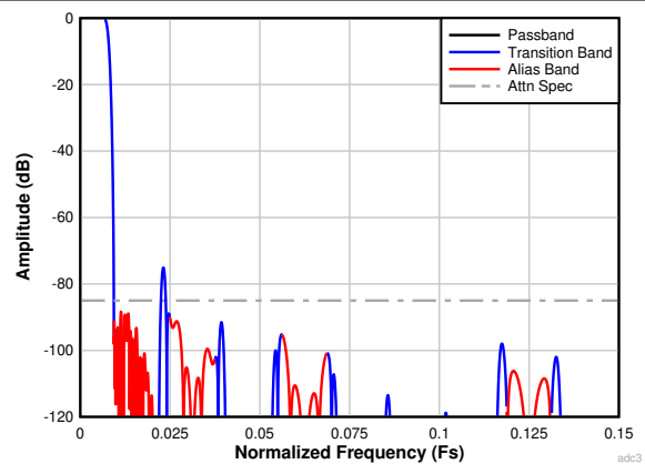
图 7-33. Complex Decimation by 64 Filter Response
