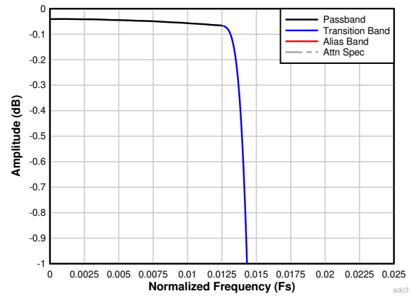
图 7-31. Decimation by 32 Passband Ripple Response
