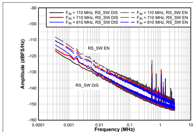
图 7-10. Amplitude Noise vs Input Frequency
