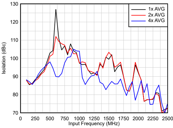
图 6-96. Isolation vs Input Frequency
