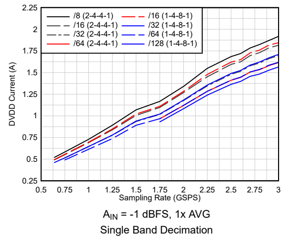
图 6-105. Current vs Sampling Rate vs Complex Decimation
