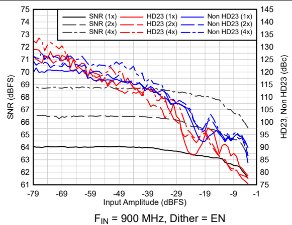
图 6-87. AC Performance vs A_{IN}
