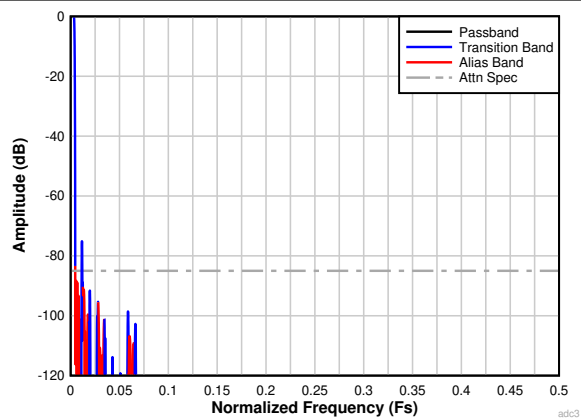
图 7-35. Complex Decimation by 128 Filter Response
