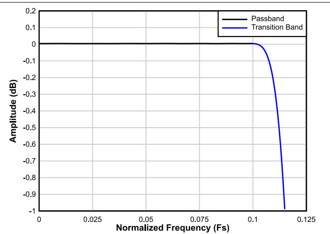
图 7-25. Decimation by 4 Passband Ripple Response
