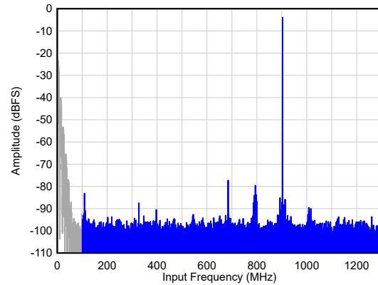
图 6-6. Single Tone FFT at F_{IN} = 900 MHz
