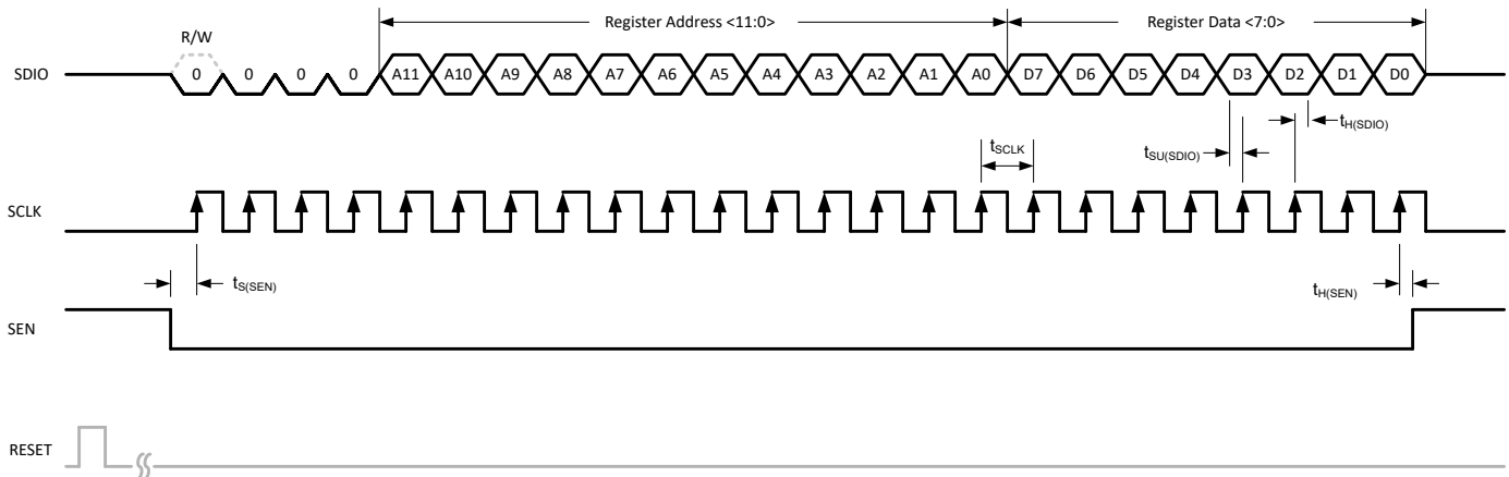
图 7-46. Serial Register Write Timing Diagram
