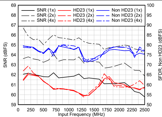
A_{IN} = -1 dBFS, Dither = DIS 图 6-82. AC Performance vs F_{IN}
