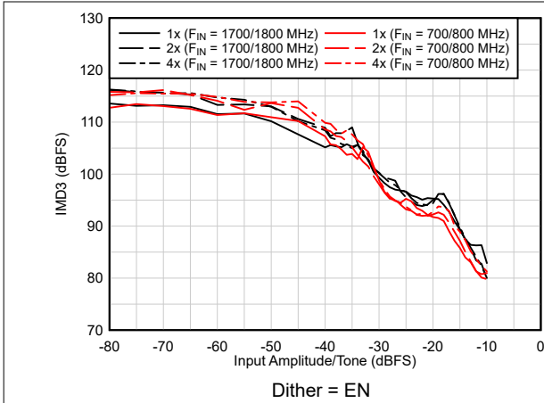
图 6-35. IMD3 Performance vs A_{IN}
