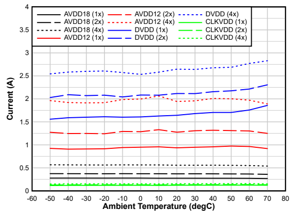
图 6-113. Current vs Temperature A_{IN} = -1 dBFS, DDC Bypass
