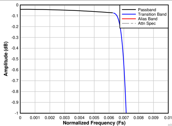
图 7-34. Decimation by 64 Passband Ripple Response
