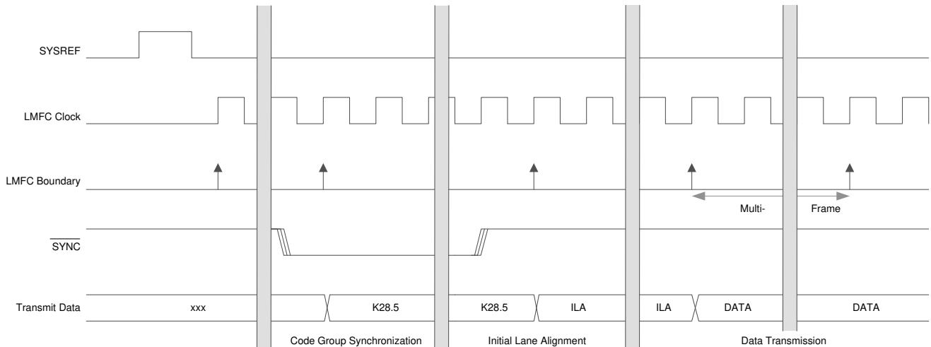
图 7-42. JESD204B Internal Timing Diagram
