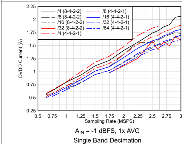
图 6-104. Current vs Sampling Rate vs Complex Decimation
