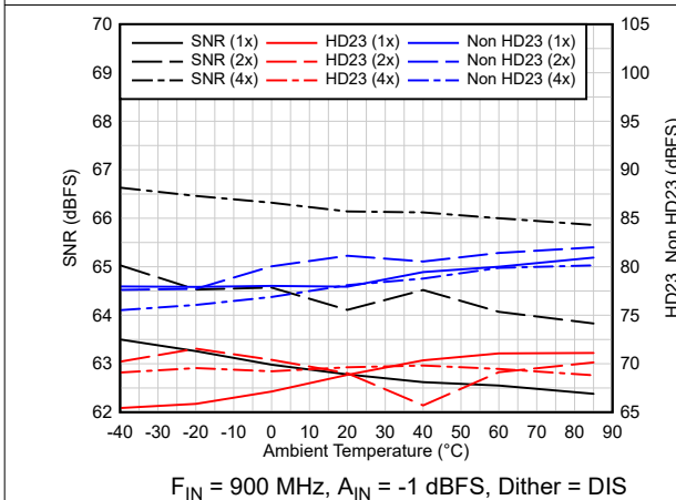
图 6-39. AC Performance vs Temperature
