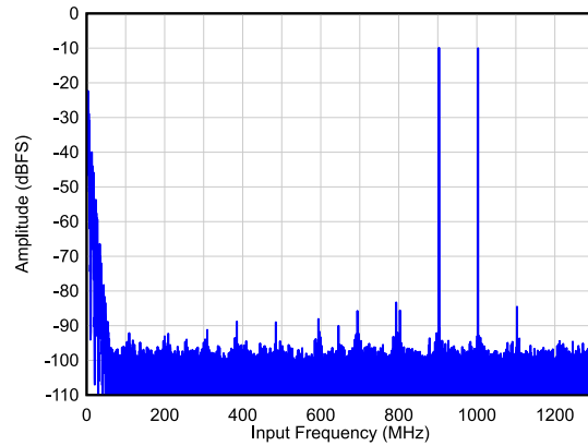
IMD3 = 74 dBc A_{IN} = -10 dBFS/tone, 1x AVG, Dither = EN
