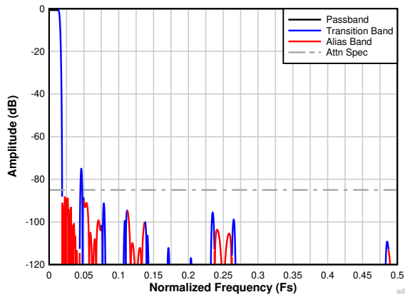
图 7-30. Complex Decimation by 32 Filter Response
