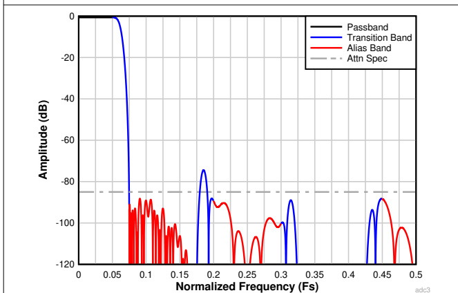
图 7-26. Complex Decimation by 8 Filter Response
