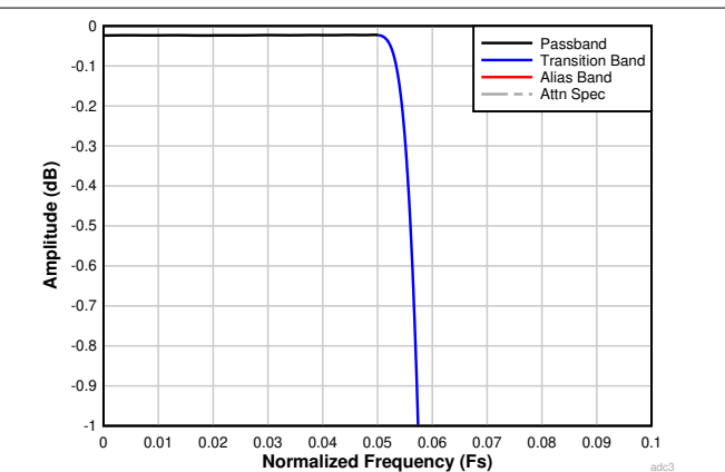
图 7-27. Decimation by 8 Passband Ripple Response
