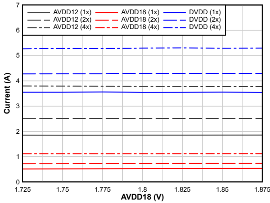
图 6-110. I_{AVDD18} vs Supply A_{IN} = -1 dBFS, DDC Bypass
