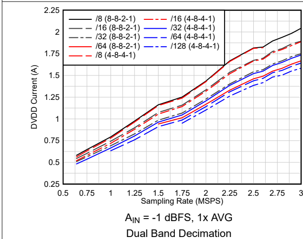
图 6-106. Current vs Sampling Rate vs Complex Decimation
