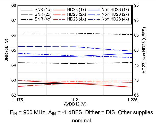
图 6-38. AC Performance vs AVDD12
