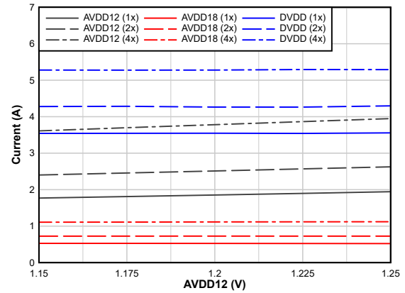
图 6-111. I_{AVDD12} vs Supply A_{IN} = -1 dBFS, DDC Bypass
