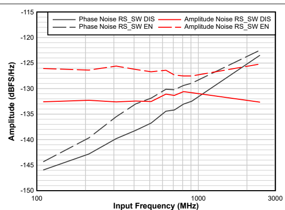
图 7-11. Amplitude and Phase noise at 10 kHz offset vs Input Frequency
