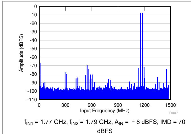
图 6-19. FFT for Two-Tone Input Signal (-8 dBFS)
