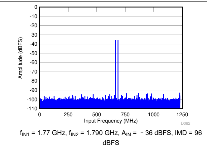
图 6-22. FFT for Two-Tone Input Signal (-36 dBFS, f_s = 2457.6 \text{ MSPS} )
