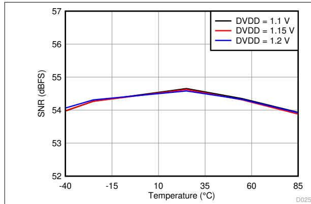
图 6-49. Signal-to-Noise Ratio vs. DVDD Supply and Temperature
