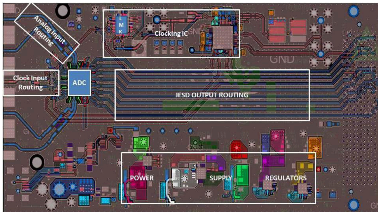
Figure 11-1. ADC32RF8x EVM Layout
