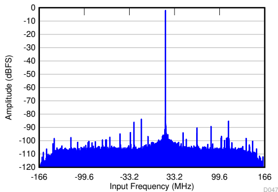
图 6-69. FFT in 6x Decimation (Complex Output)
