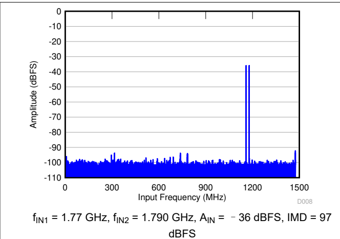
图 6-20. FFT for Two-Tone Input Signal (-36 dBFS)
