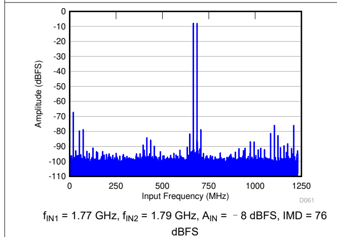
图 6-21. FFT for Two-Tone Input Signal (-8 dBFS, f_s = 2457.6 \text{ MSPS} )
