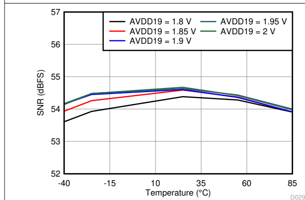
图 6-51. Signal-to-Noise Ratio vs. AVDD19 Supply and Temperature
