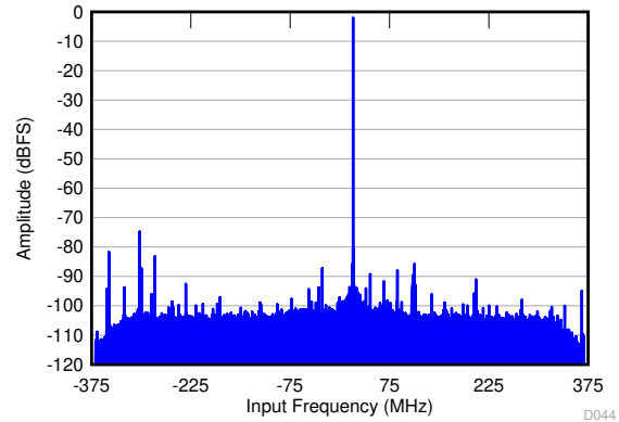
图 6-68. FFT in 4x Decimation (Complex Output)
