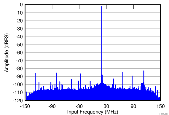
图 6-70. FFT in 8x Decimation (Complex Output)
