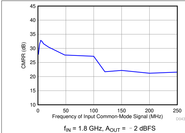
图 6-67. Common-Mode Rejection Ratio vs. Tone Frequency
