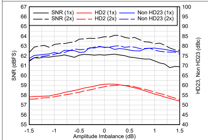
图 6-5. Amplitude Imbalance - 3.0 GSPS
