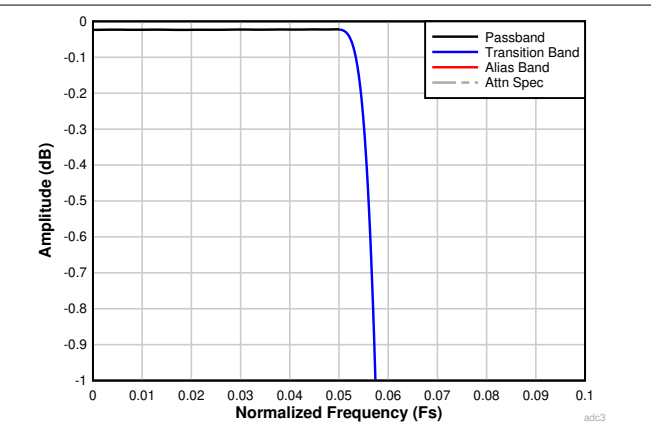
图 6-27. Decimation by 8 Passband Ripple Response
