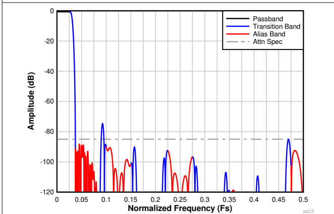
图 6-28. Complex Decimation by 16 Filter Response
