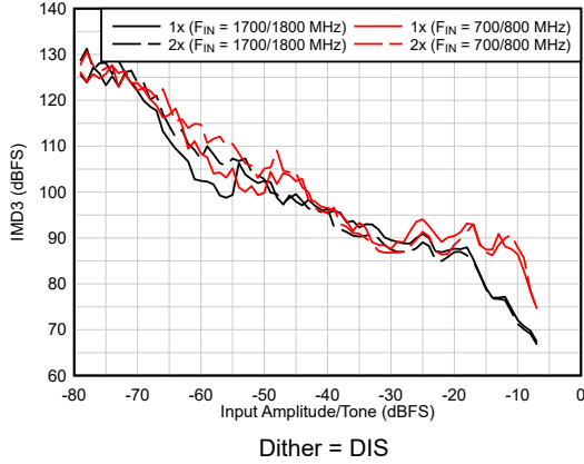
图 5-29. IMD3 Performance vs A_{IN}
