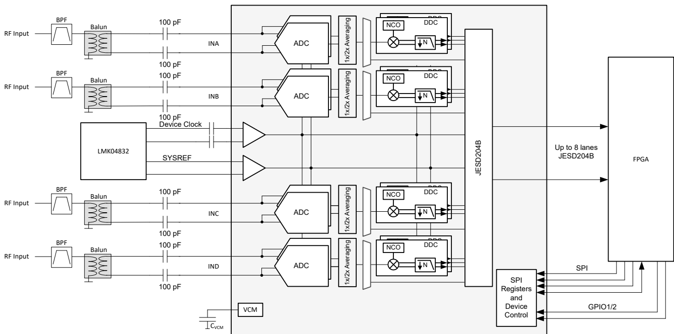
图 7-1. Typical Configuration for Wideband RF Sampling
