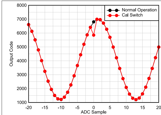
图 6-18. Output Code vs ADC Sample
