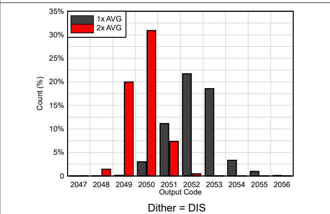
图 5-40. DC Offset Histogram
