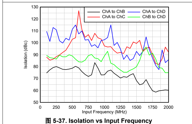
图 5-37. Isolation vs Input Frequency
