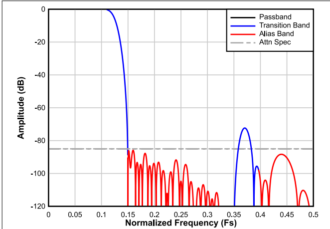
图 6-24. Complex Decimation by 4 Filter Response
