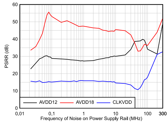
图 7-5. Power supply rejection ratio (PSRR) vs frequency
