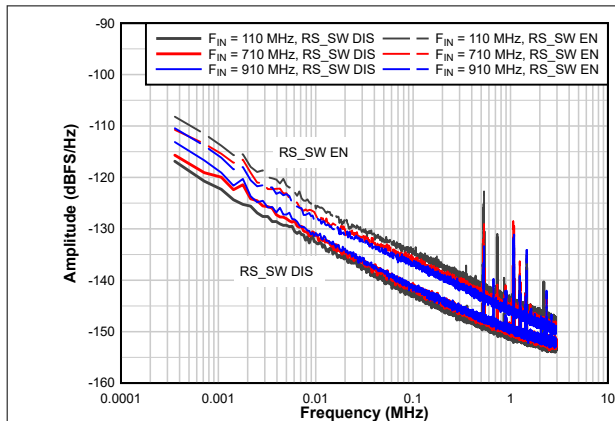
图 6-10. Amplitude Noise vs Input Frequency
