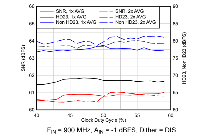
图 5-36. AC Performance vs Clock Duty Cycle
