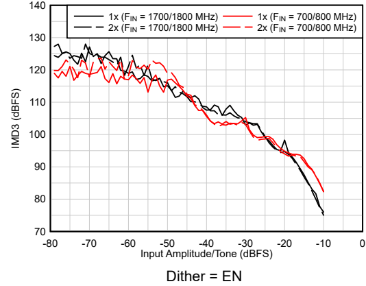
图 5-30. IMD3 Performance vs A_{IN}
