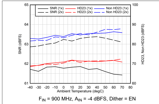
图 5-35. AC Performance vs Temperature
