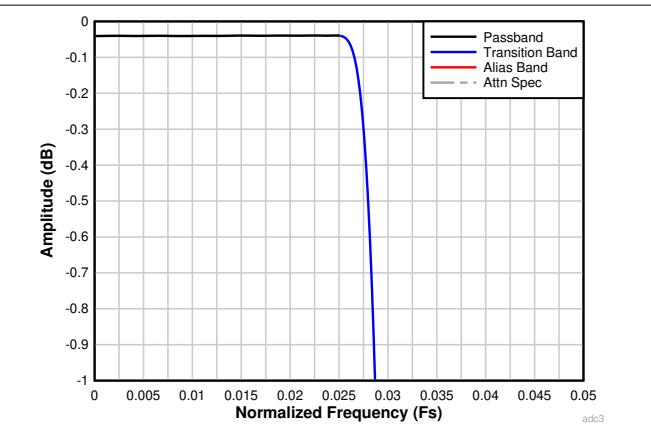
图 6-29. Decimation by 16 Passband Ripple Response
