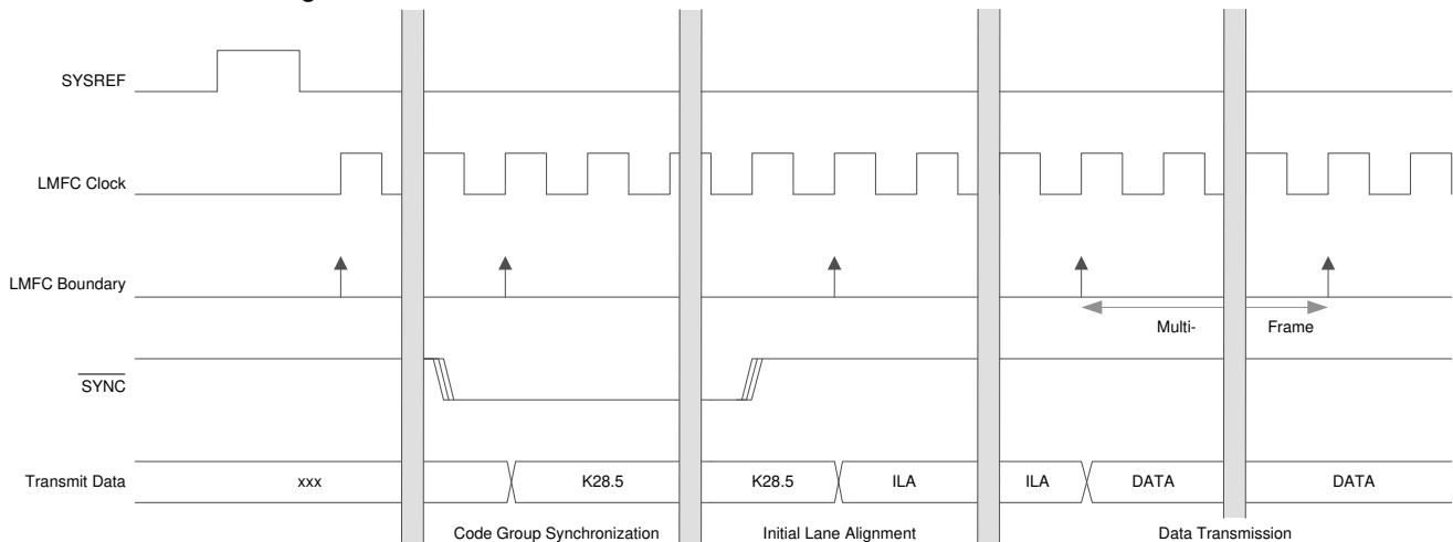
图 6-42. JESD204B Internal Timing Diagram
