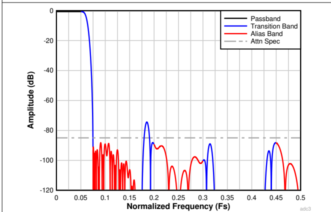
图 6-26. Complex Decimation by 8 Filter Response
