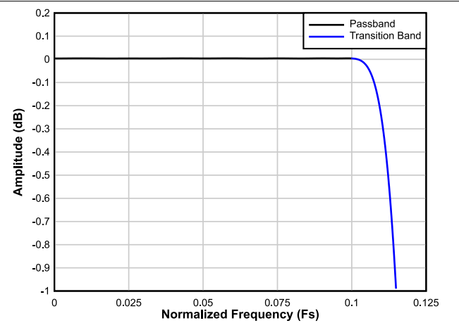
图 6-25. Decimation by 4 Passband Ripple Response
