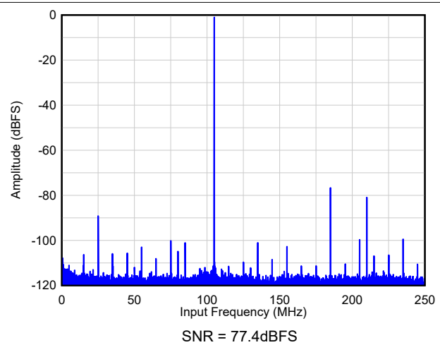
图 8-73. FFT - 2x AVG ( F_{IN} = 105\text{MHz} , A_{IN} = -1\text{dBFS} )
