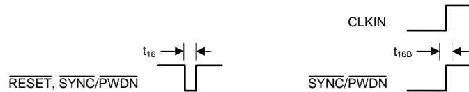
Figure 2. \overline{\text{RESET}} and \overline{\text{SYNC/PWDN}} Timing
