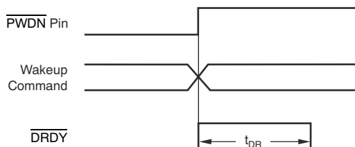
Figure 49. \overline{\text{PWN}} Pin and Wake-Up Command Timing ( Pulse-Sync Timing Requirements Shows t_{DR} )
