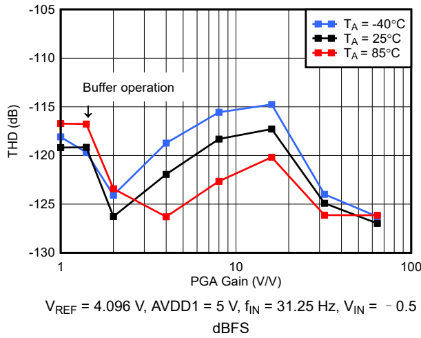
图 6-49. High-Power Mode THD vs PGA Gain
