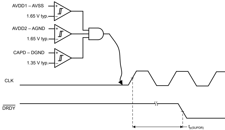
图 6-8. Power-Up Switching Characteristics
