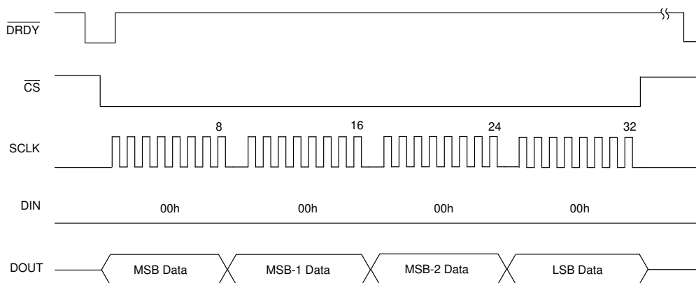
图 8-24. Read Data Direct
