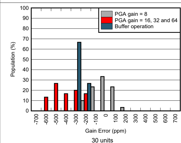
图 6-42. Gain Error Distribution
