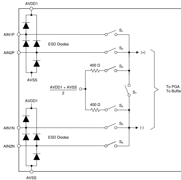
图 8-1. Analog Input and Multiplexer
