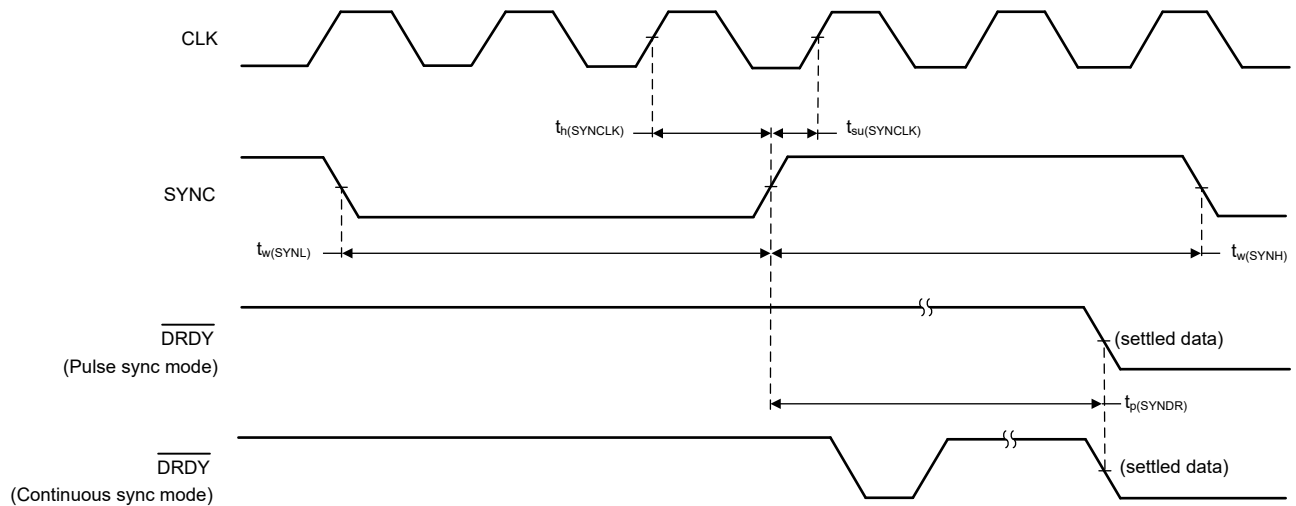
图 6-4. SYNC Timing Requirements and Switching Characteristics
