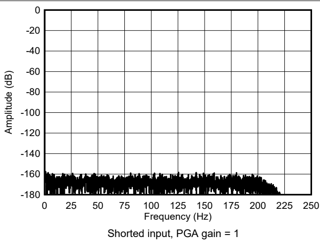
图 6-19. Mid-Power Mode FFT Spectrum
