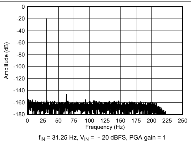
图 6-14. High-Power Mode FFT Spectrum
