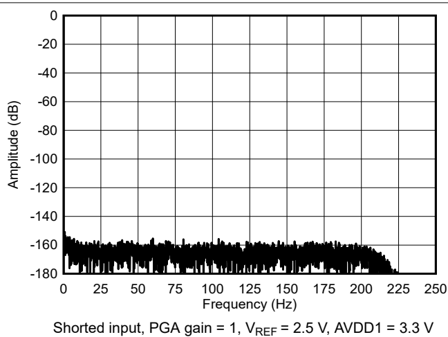
图 6-11. High-Power Mode FFT Spectrum
