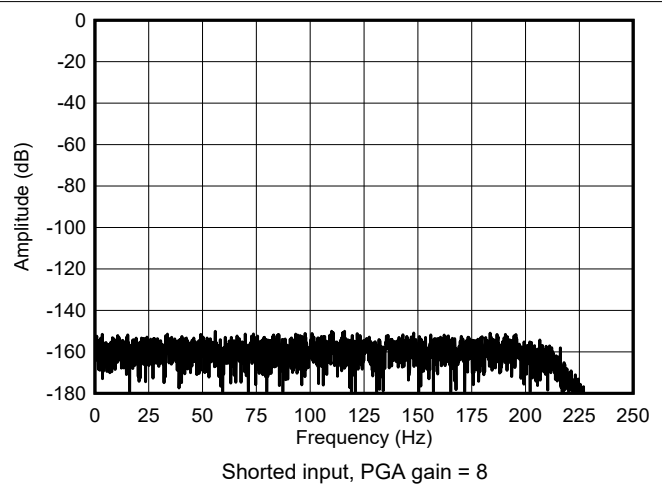
图 6-20. Mid-Power Mode FFT Spectrum
