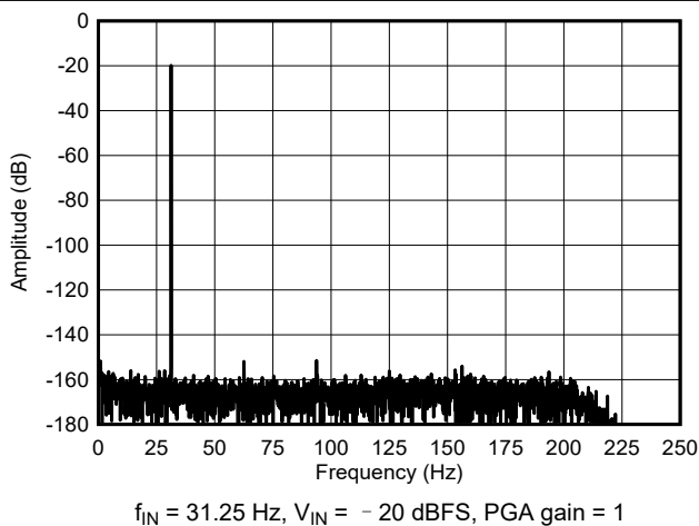
图 6-21. Mid-Power Mode FFT Spectrum
