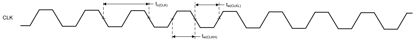
图 6-1. Clock Timing Requirements
