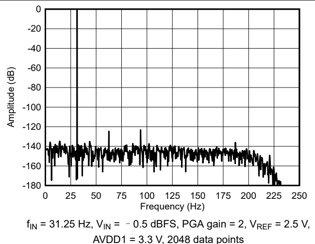
图 6-24. Mid-Power Mode FFT Spectrum
