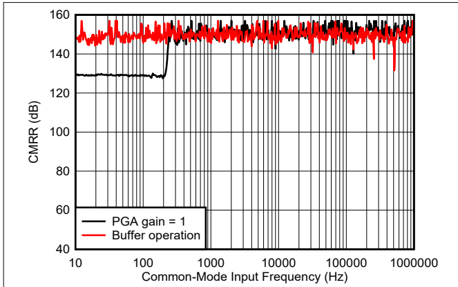
图 6-59. CMRR vs Common-Mode Input Frequency
