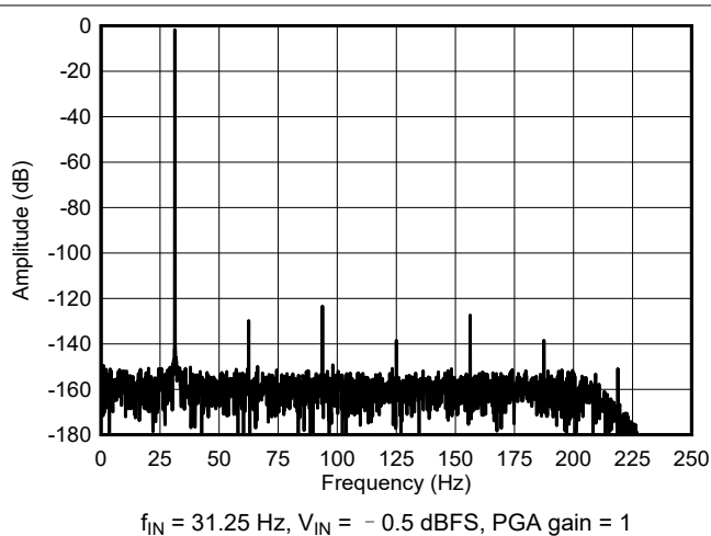
图 6-13. High-Power Mode FFT Spectrum
