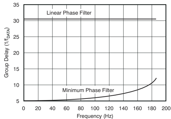
图 8-18. FIR Group Delay ( f_{DATA} = 500 SPS)
