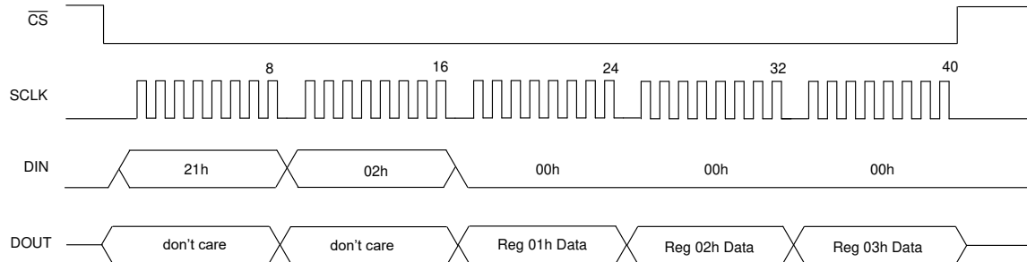
图 8-26. Read Register Data
