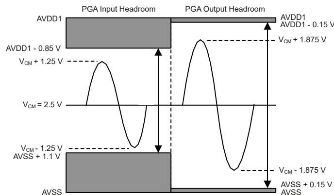
图 8-5. PGA Headroom (AVDD1 = 5 V, PGA Gain = 1)
