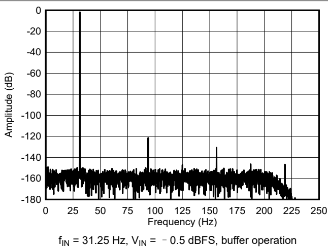
图 6-15. High-Power Mode FFT Spectrum
