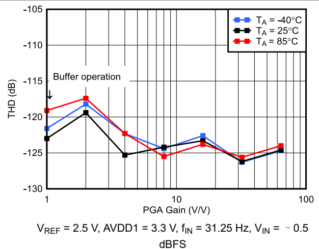
图 6-46. High-Power Mode THD vs PGA Gain
