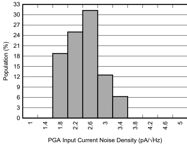
图 6-55. PGA Input Current Noise Distribution
