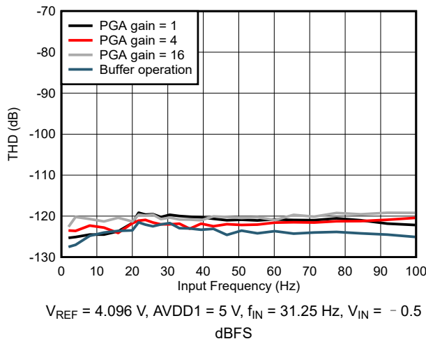
图 6-53. Low-Power Mode THD vs Input Frequency
