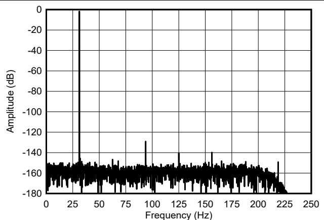
图 6-28. Low-Power Mode FFT Spectrum
