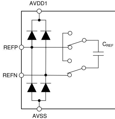
图 8-8. Simplified Voltage Reference Input Circuit
