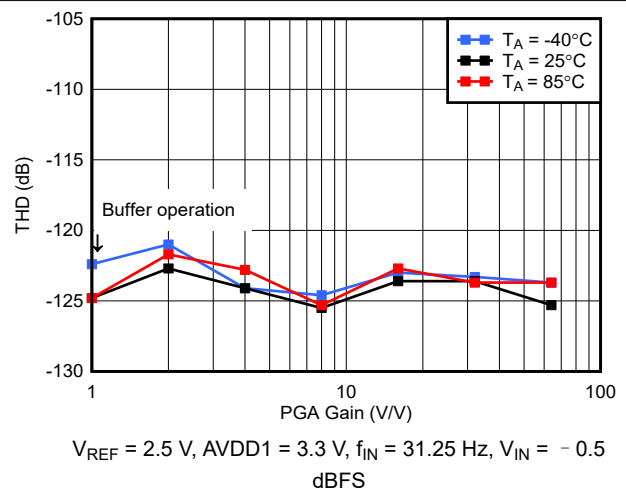
图 6-48. Low-Power Mode THD vs PGA Gain
