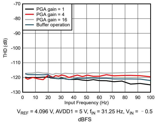
图 6-52. High- and Mid-Power Mode THD vs Input Frequency
