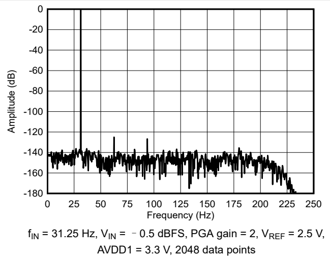
图 6-32. Low-Power Mode FFT Spectrum
