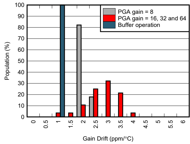
图 6-44. Gain Drift Distribution
