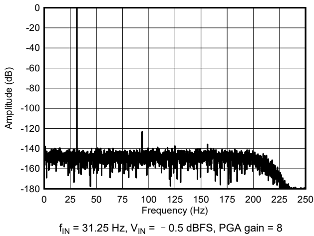
图 6-33. Low-Power Mode FFT Spectrum
