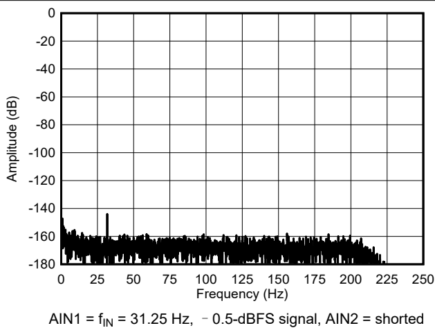
图 6-35. Channel-to-Channel Crosstalk
