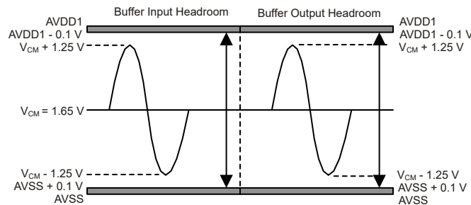
图 8-7. Buffer Headroom (3.3-V Operation Shown)
