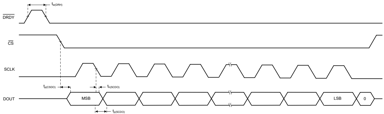
图 6-3. Serial Interface Switching Characteristics
