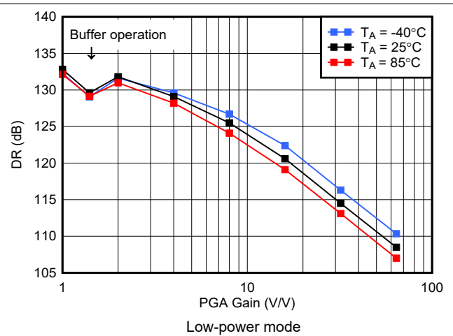
图 6-38. Dynamic Range vs PGA Gain
