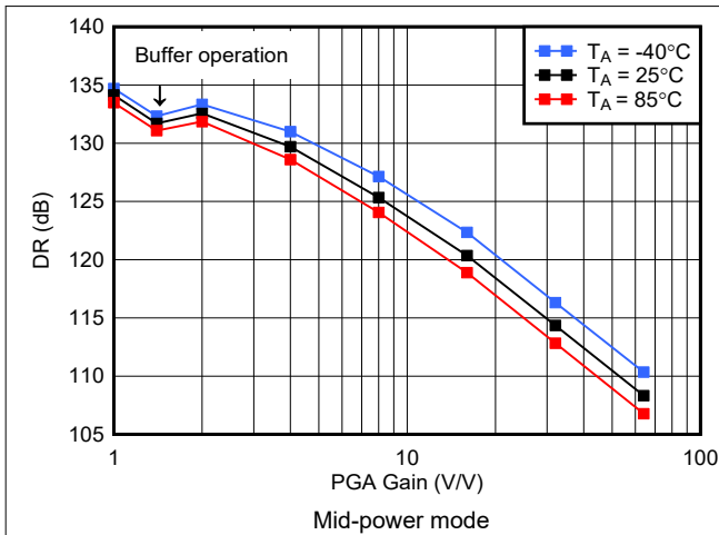
图 6-37. Dynamic Range vs PGA Gain
