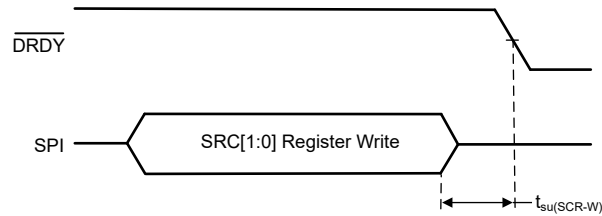
图 6-7. Sample Rate Converter Register-Write Timing Requirements
