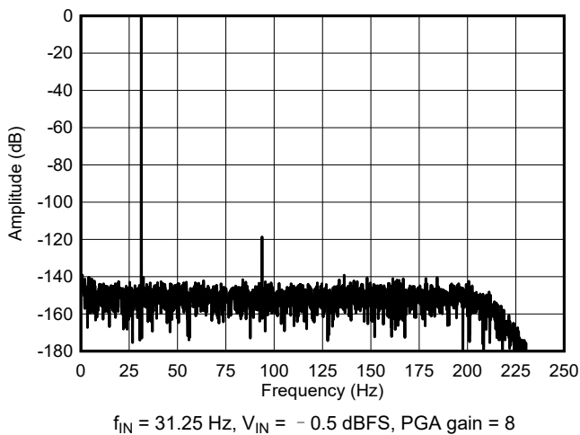
图 6-17. High-Power Mode FFT Spectrum
