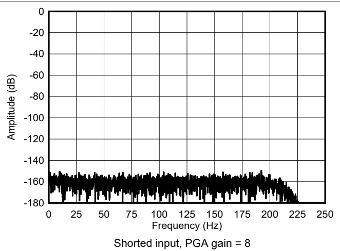
图 6-10. High-Power Mode FFT Spectrum
