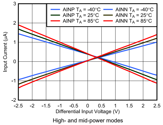
图 6-56. Buffer Input Current vs Input Voltage
