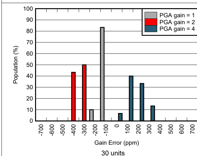
图 6-41. Gain Error Distribution
