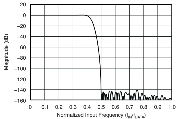
图 8-16. FIR Filter Transition Band Response
