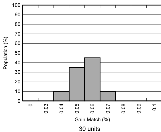
图 6-45. Gain Match Distribution
