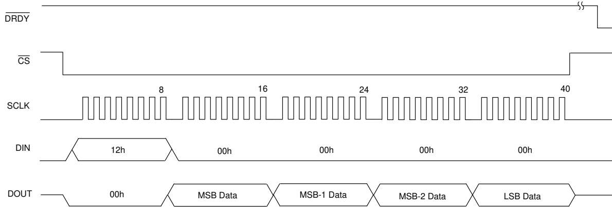
图 8-25. Read Conversion Data by Command
