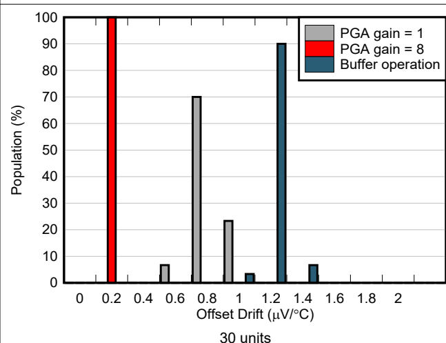
图 6-40. Offset Drift Distribution
