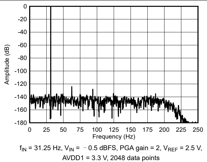
图 6-16. High-Power Mode FFT Spectrum
