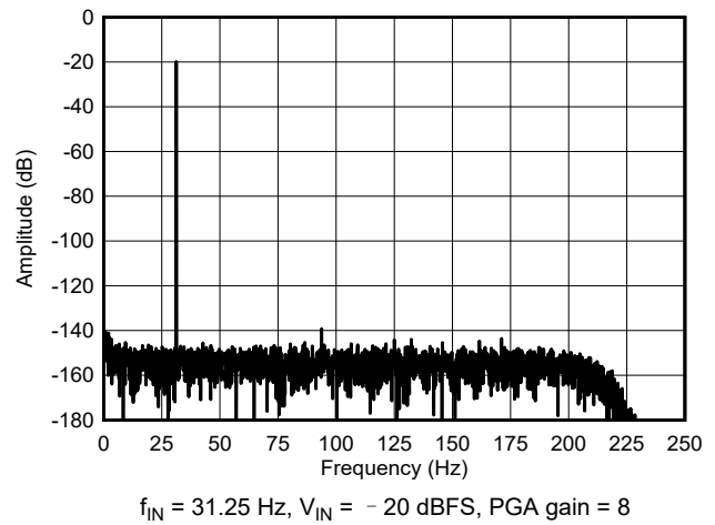
图 6-34. Low-Power Mode FFT Spectrum
