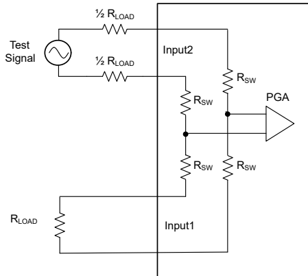
图 8-2. THD versus R_{LOAD} Test Circuit
