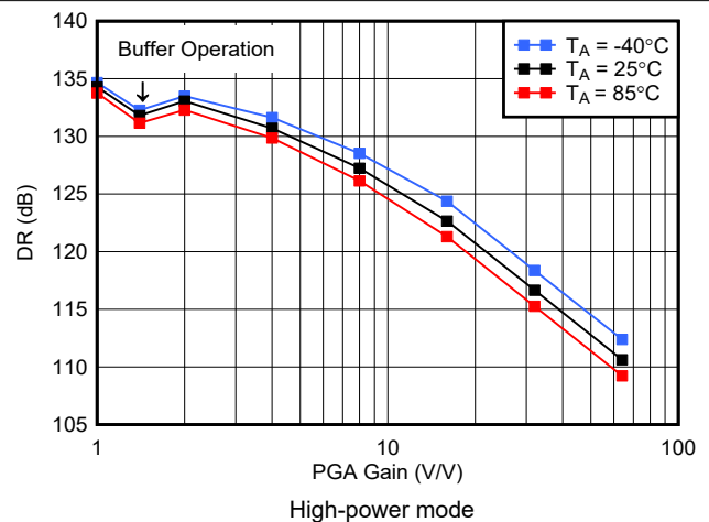
图 6-36. Dynamic Range vs PGA Gain
