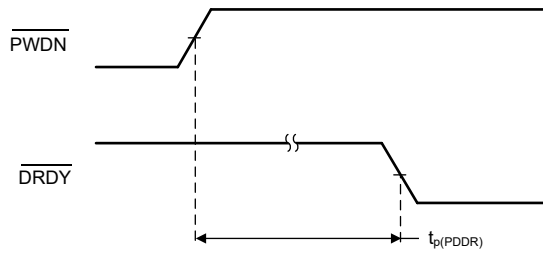
图 6-6. PWDN Switching Characteristics
