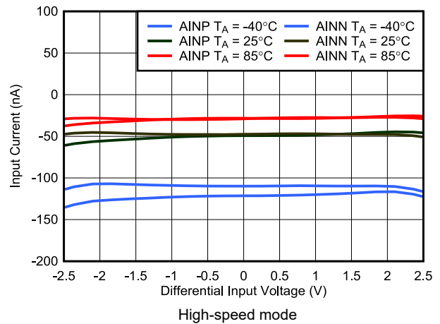
图 6-54. PGA Input Current vs Input Voltage
