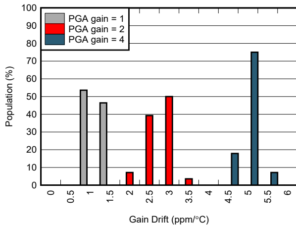
图 6-43. Gain Drift Distribution
