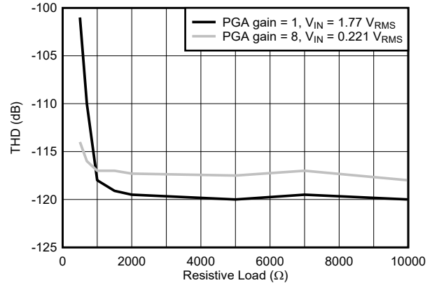
图 8-3. THD Performance vs R_{LOAD}
