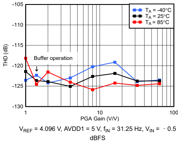
图 6-51. Low-Power Mode THD vs PGA Gain
