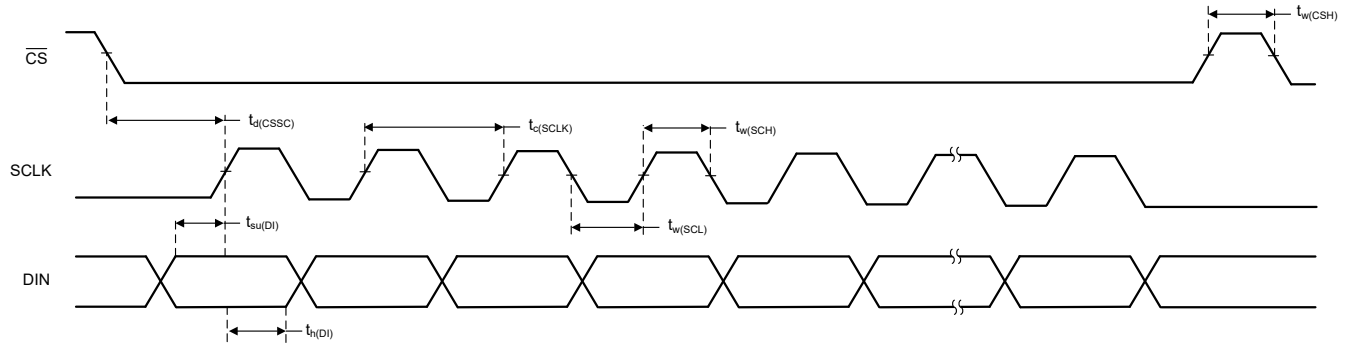
图 6-2. Serial Interface Timing Requirements
