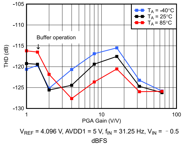
图 6-50. Mid-Power Mode THD vs PGA Gain
