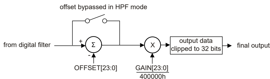
图 8-20. Calibration Block Diagram
