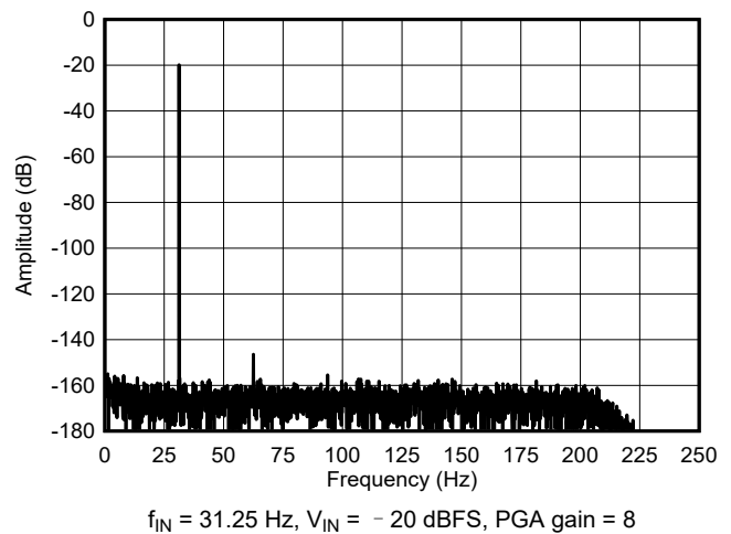
图 6-18. High-Power Mode FFT Spectrum
