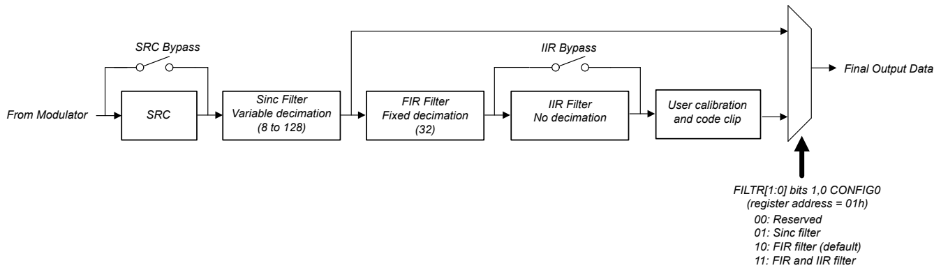
图 8-10. Digital Filter Block Diagram
