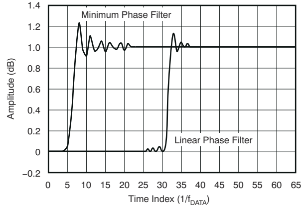
图 8-17. FIR Step Response
