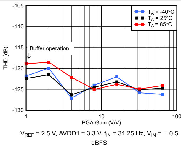
图 6-47. Mid-Power Mode THD vs PGA Gain
