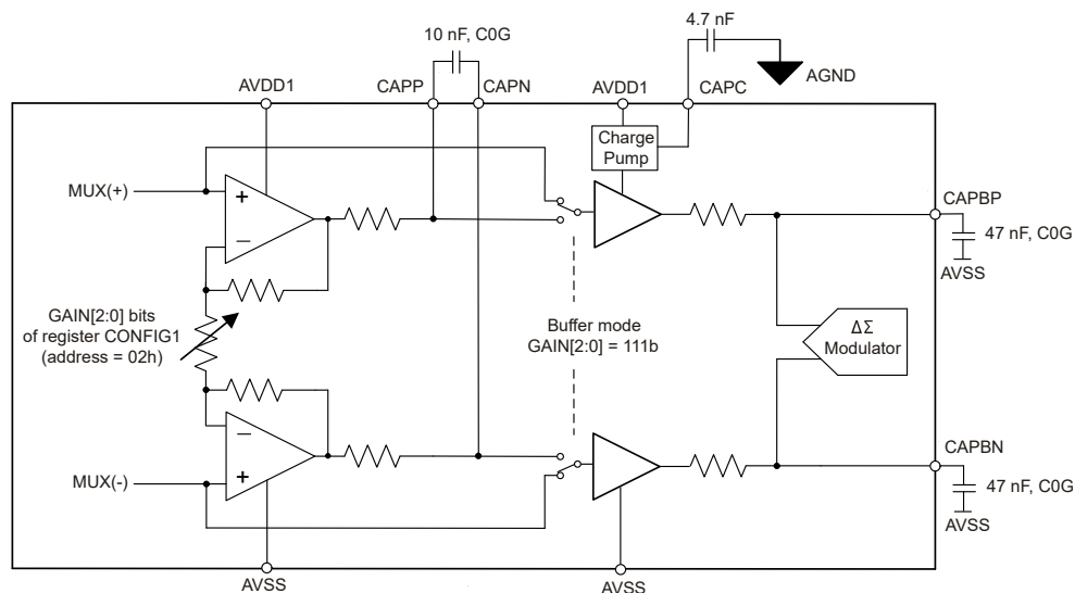
图 8-4. PGA and Buffer Block Diagram
