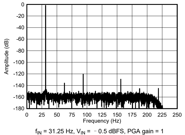
图 6-22. Mid-Power Mode FFT Spectrum
