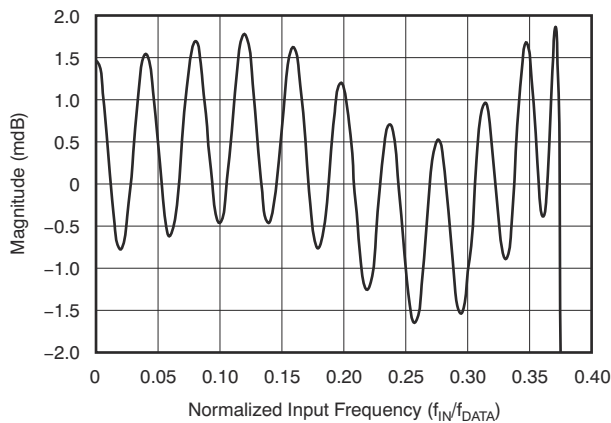
图 8-15. FIR Filter Pass-Band Response
