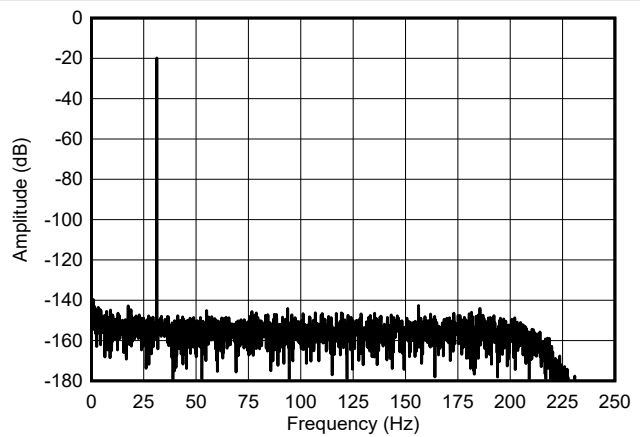
图 6-26. Mid-Power Mode FFT Spectrum
