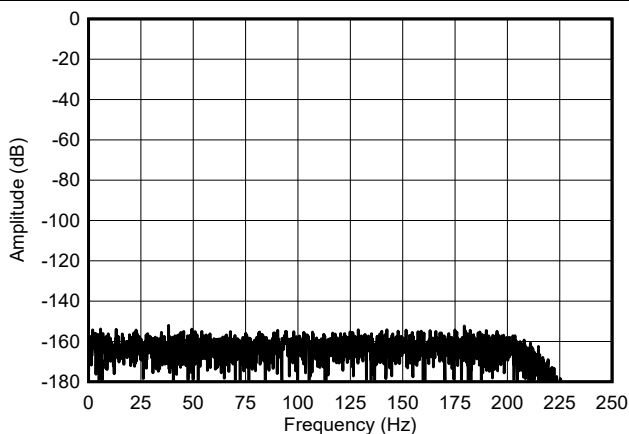
图 6-27. Low-Power Mode FFT Spectrum
