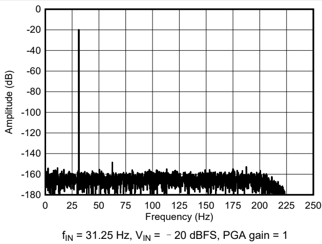
图 6-31. Low-Power Mode FFT Spectrum
