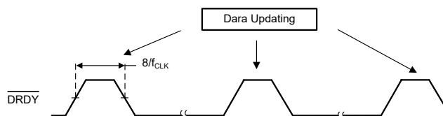
图 8-22. \overline{DRDY} With No Data Retrieval
