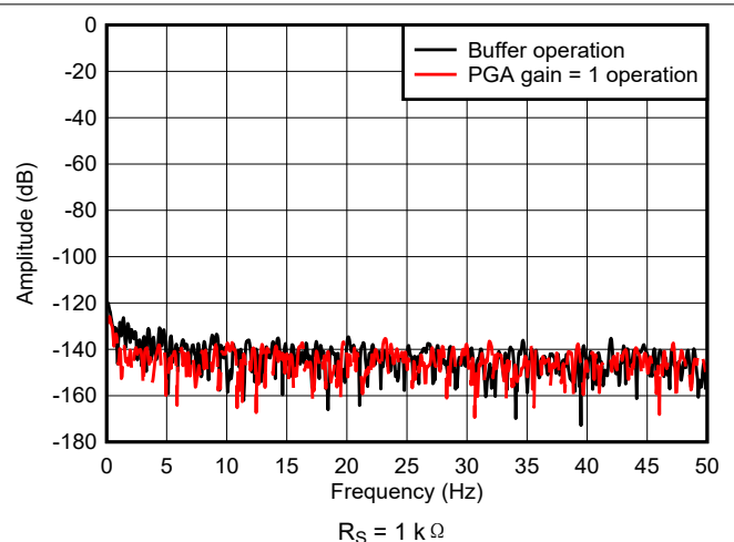
图 6-12. High-Power Mode FFT Spectrum
