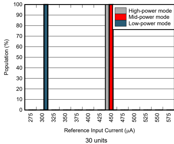
图 6-58. Reference Input Current Distribution
