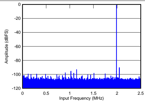
f_S = 5 MSPS, f_{IN} = 3 MHz, SNR = 70.9 dBFS, SFDR = 89 dBc, SINAD = 70.8 dBFS, THD = 87 dBc
