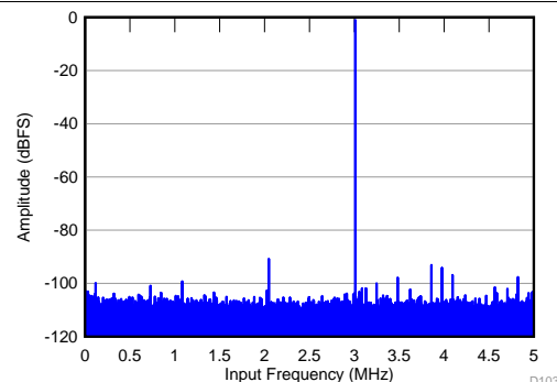
f_S = 10 MSPS, f_{IN} = 3 MHz, SNR = 71.1 dBFS, SFDR = 89 dBc, SINAD = 71 dBFS, THD = 86 dBc
