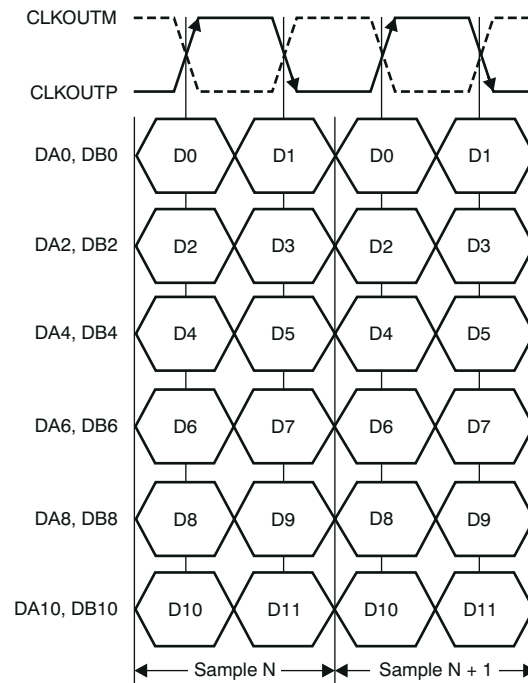
图 7-4. ADS4226/25/22 LVDS Interface Timing Diagram
