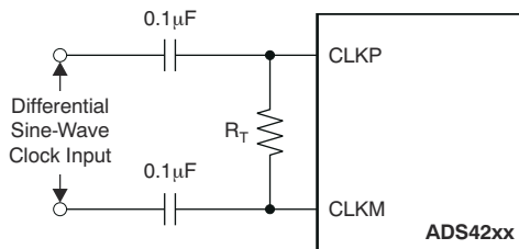
图 8-10. Differential Sine-Wave Clock Driving Circuit
