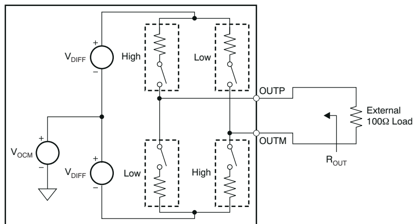
图 8-22. LVDS Buffer Equivalent Circuit
