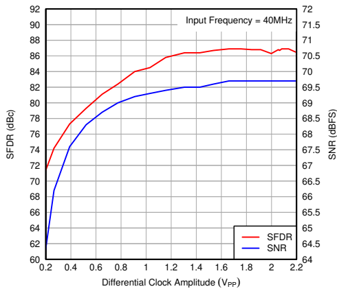
图 7-102. Performance vs Input Clock Amplitude
