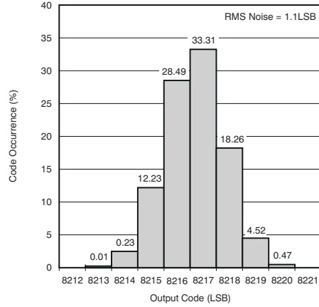
图 7-69. Output Noise Histogram (With Inputs Shorted to VCM)
