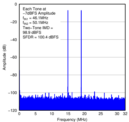
图 7-108. FFT for Two-Tone Input Signal
