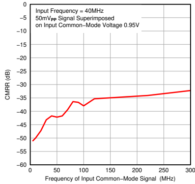
图 7-124. CMRR vs Test Signal Frequency
