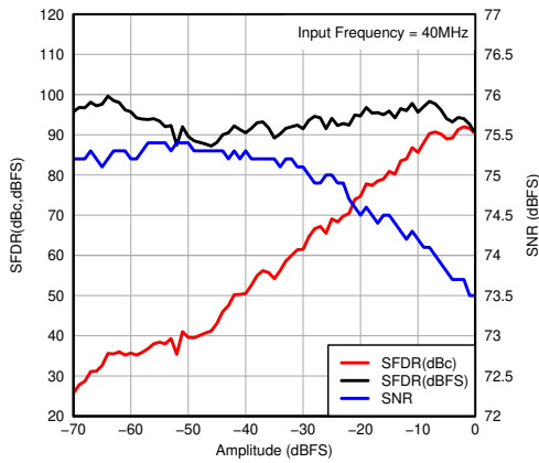
图 7-58. Performance vs Input Amplitude
