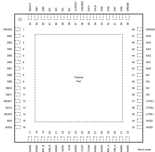
图 6-4. ADS4226, ADS4225, and ADS4222 RGC Package 64-Pin VQFN With Exposed Thermal Pad CMOS Mode (Top View)
