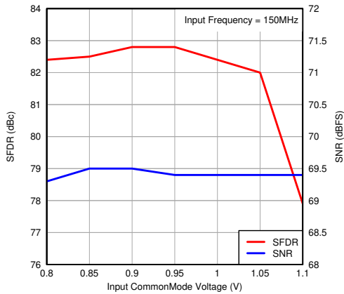
图 7-82. Performance vs Input Common-Mode Voltage
