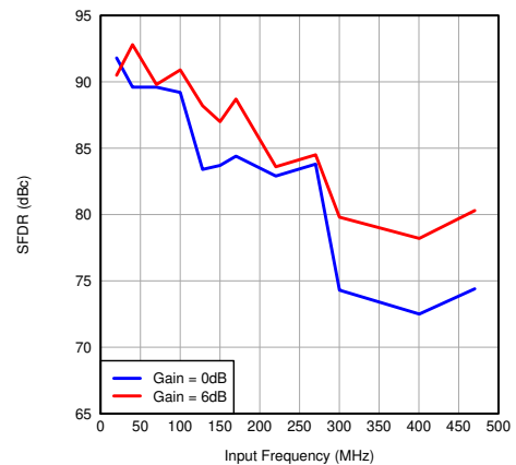
图 7-109. SFDR vs Input Frequency
