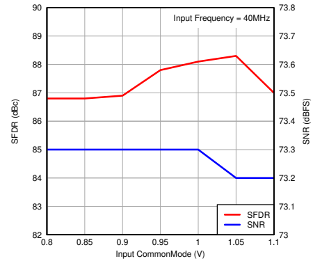
图 7-39. Performance vs Input Common-Mode Voltage
