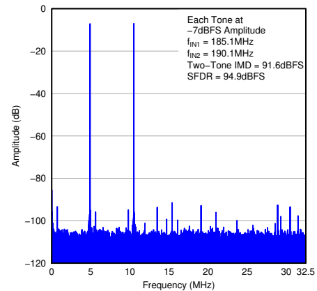
图 7-107. FFT for Two-Tone Input Signal
