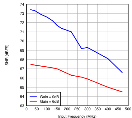
图 7-33. SNR vs Input Frequency
