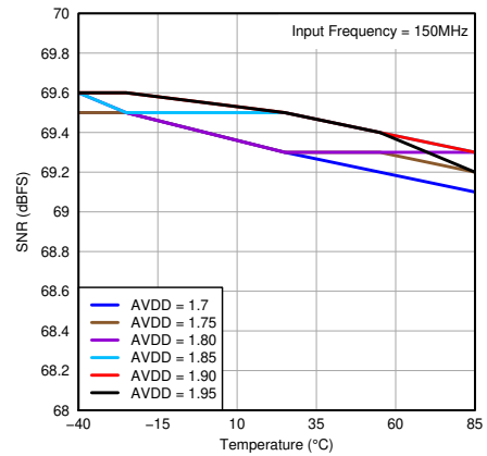
图 7-83. SNR vs Temperature and AVDD Supply
