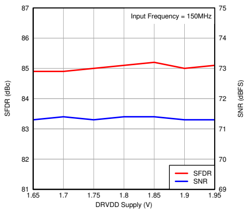
图 7-64. Performance vs DRVDD Supply Voltage
