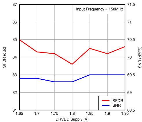
图 7-84. Performance vs DRVDD Supply Voltage
