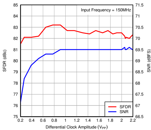
图 7-86. Performance vs Input Clock Amplitude
