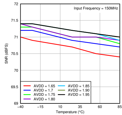
图 7-21. SNR vs Temperature and AVDD Supply
