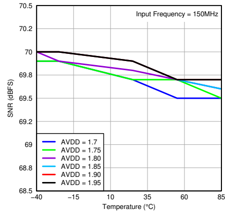
图 7-99. SNR vs Temperature and AVDD Supply
