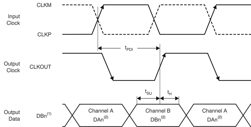
图 8-25. Multiplexed Mode Timing Diagram
