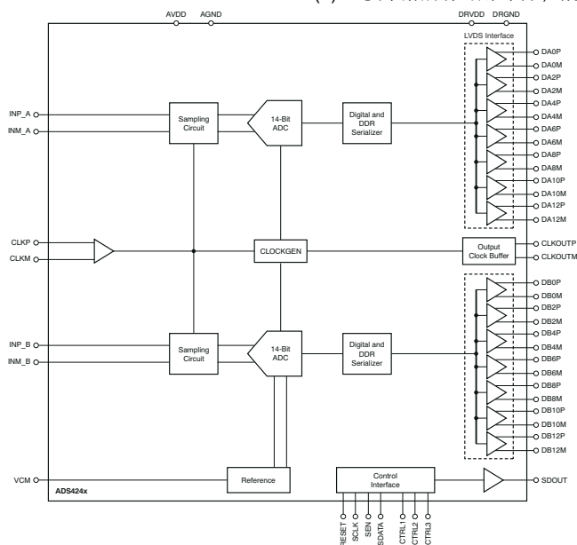
ADS4222/25/26/42/45/46 方框图
