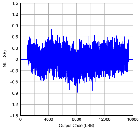
图 7-68. Integrated Nonlinearity
