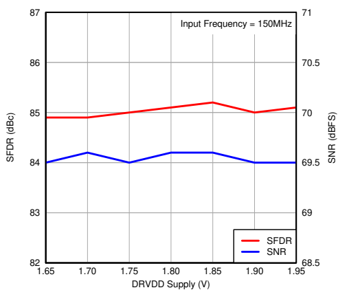
图 7-120. Performance vs DRVDD Supply Voltage
