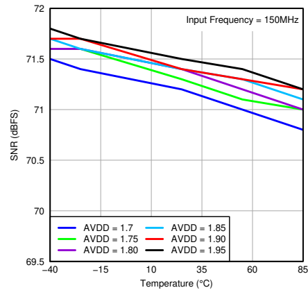
图 7-63. SNR vs Temperature and AVDD Supply
