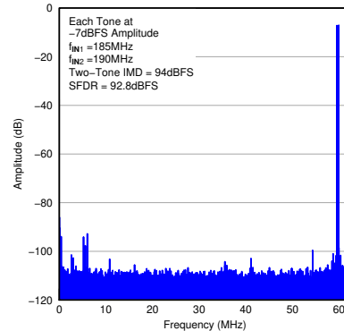
图 7-31. FFT for Two-Tone Input Signal
