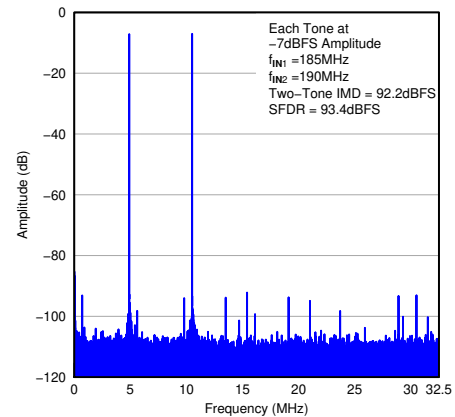
图 7-51. FFT for Two-Tone Input Signal
