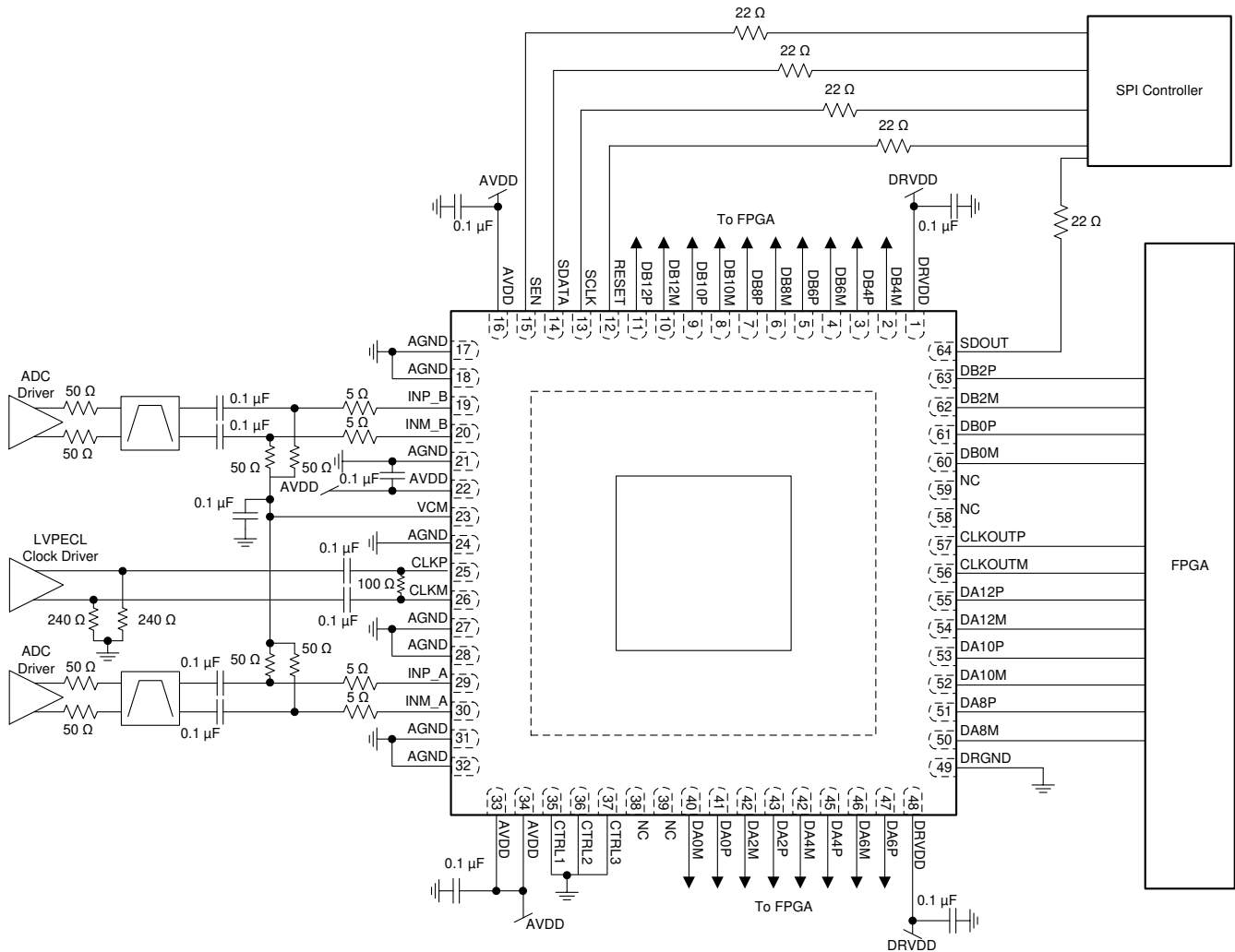
图 9-1. Example Schematic for ADS4246
