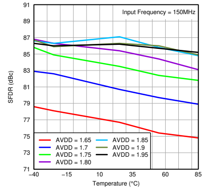
图 7-41. SFDR vs Temperature and AVDD Supply
