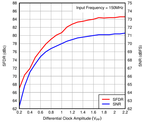
图 7-66. Performance vs Input Clock Amplitude
