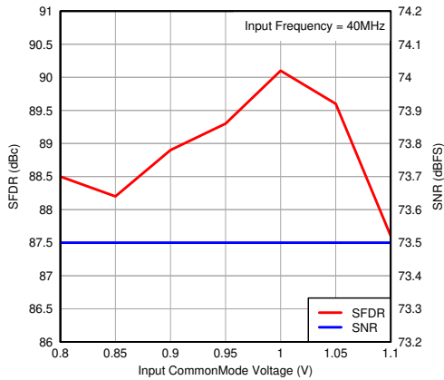
图 7-60. Performance vs Input Common-Mode Voltage
