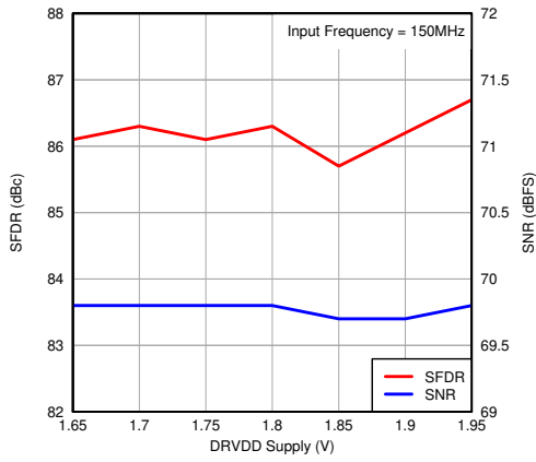
图 7-100. Performance vs DRVDD Supply Voltage
