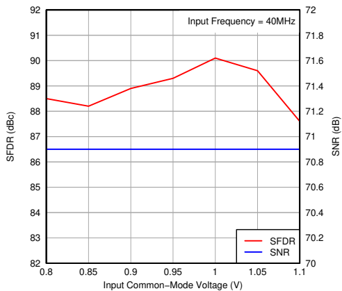
图 7-116. Performance vs Input Common-Mode Voltage
