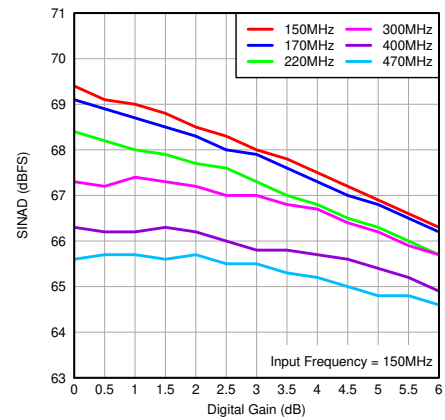
图 7-113. SINAD vs Gain and Input Frequency
