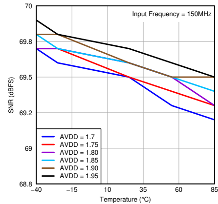
图 7-119. SNR vs Temperature and AVDD Supply
