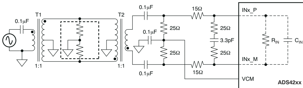
图 8-6. Drive Circuit with Low Bandwidth (for Low Input Frequencies Less Than 150 MHz)
