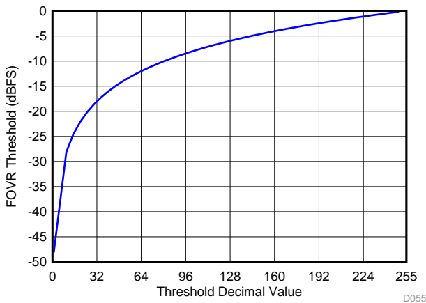
Figure 67. Programming Fast OVR Thresholds
