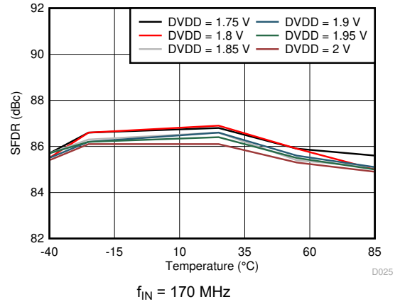
图 7-28. Spurious-Free Dynamic Range vs DVDD Supply and Temperature
