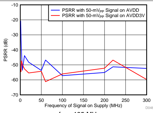
Figure 48. Power-Supply Rejection Ratio vs Noise Signal Frequency f_{\text{IN}} = 185 \text{ MHz}
