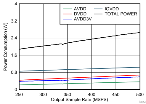
Figure 52. Power Consumption vs Sampling Speed
