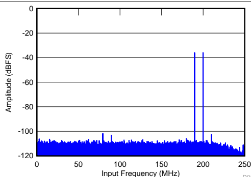
Figure 11. FFT for Two-Tone Input Signal ( -36\text{ dBFS} )
