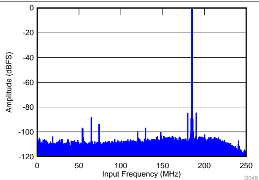
Figure 47. Power-Supply Rejection Ratio FFT for AVDD Supply A_{\text{IN}} = -1 \text{ dBFS} , SFDR = 84 dBc, SINAD = 70 dBFS, f_{\text{PSRR}} = 5 \text{ MHz} , A_{\text{PSRR}} = 50 \text{ mV}_{\text{PP}} , f_{\text{IN}} = 185 \text{ MHz} , amplitude: f_{\text{IN}} - f_{\text{PSRR}} = 85 \text{ dBc} , f_{\text{IN}} + f_{\text{PSRR}} = 84 \text{ dBc}
