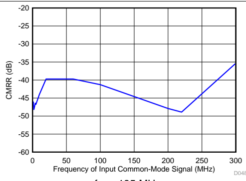
Figure 50. Common-Mode Rejection Ratio vs Common-Mode Signal Frequency f_{\text{IN}} = 185 \text{ MHz}
