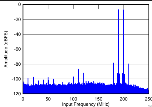
Figure 10. FFT for Two-Tone Input Signal ( -7\text{ dBFS} )
