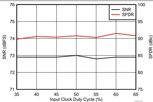
Figure 45. Performance vs Input Clock Duty Cycle f_{\text{IN}} = 185 \text{ MHz}
