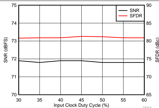
Figure 46. Performance vs Input Clock Duty Cycle f_{\text{IN}} = 300 \text{ MHz}
