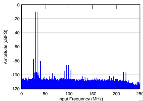
Figure 12. FFT for Two-Tone Input Signal ( -7\text{ dBFS} )
