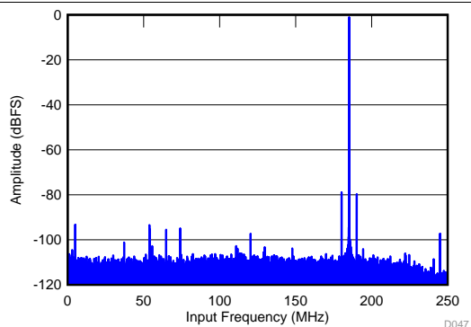
Figure 49. Common-Mode Rejection Ratio FFT A_{\text{IN}} = -1 \text{ dBFS} , SFDR = 78 dBc, SINAD = 71 dBFS, f_{\text{CMRR}} = 5 \text{ MHz} , A_{\text{CMRR}} = 50 \text{ mV}_{\text{PP}} , f_{\text{IN}} = 185 \text{ MHz} , amplitude: f_{\text{IN}} - f_{\text{CMRR}} = 79 \text{ dBc} , f_{\text{IN}} + f_{\text{CMRR}} = 80 \text{ dBc}
