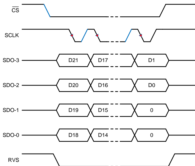
Figure 68. SPI-10-Q Protocol
