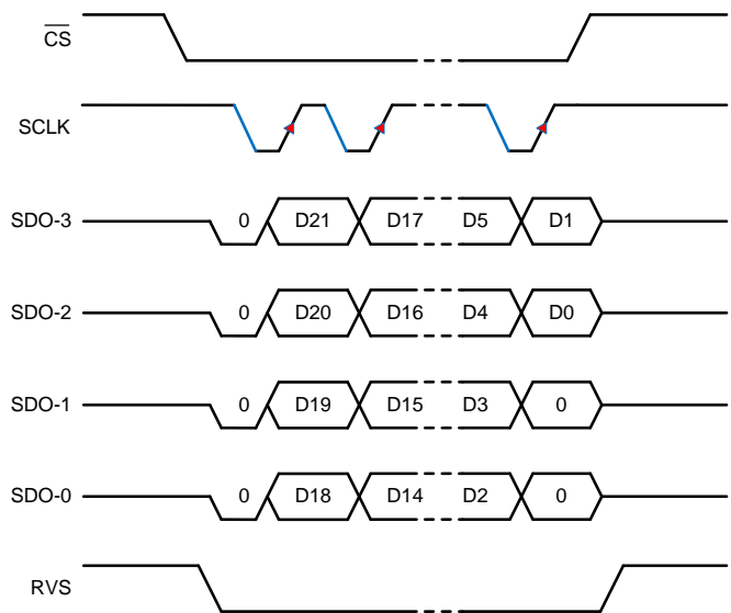
Figure 69. SPI-11-Q Protocol
