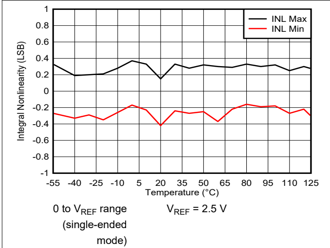
图 6-32. Integral Linearity Error vs Temperature
