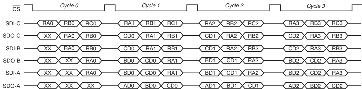
图 7-29. Three devices in a Daisy-Chain Configuration
