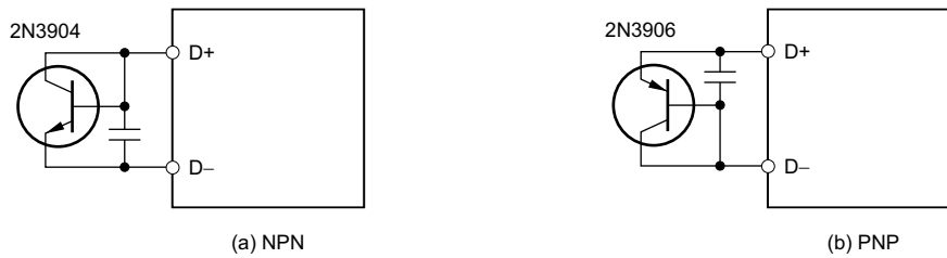
图 7-6. Remote Temperature Sensor Using Transistor
