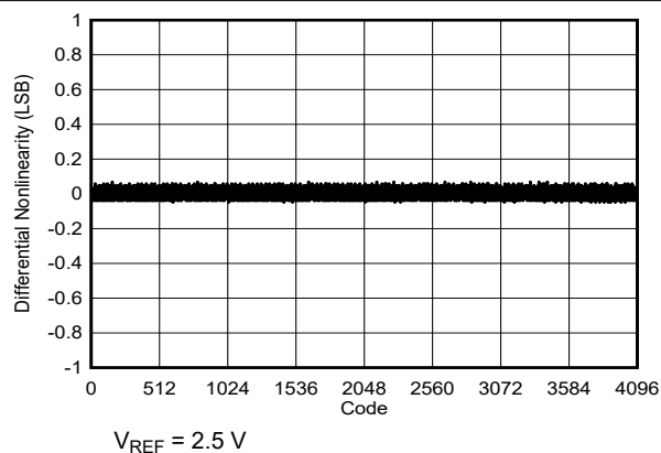
图 6-6. Differential Linearity Error vs Code
