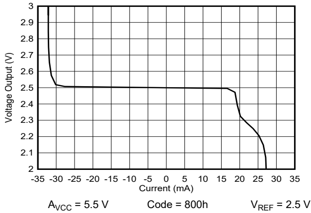
图 6-12. Output Voltage vs Output Current
