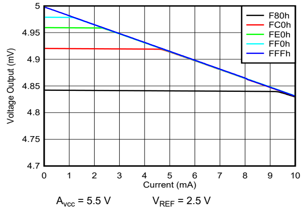
图 6-13. Output Voltage vs Source Current Capability
