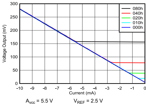
图 6-14. Output Voltage vs Sink Current Capability
