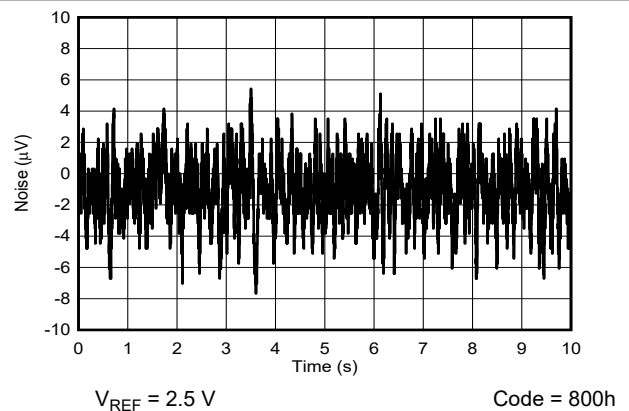
图 6-17. DAC Noise (0.1 Hz to 10 Hz)
