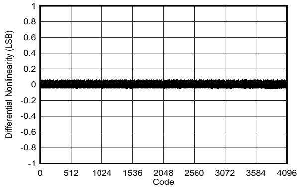
图 6-6. Differential Linearity Error vs Code
