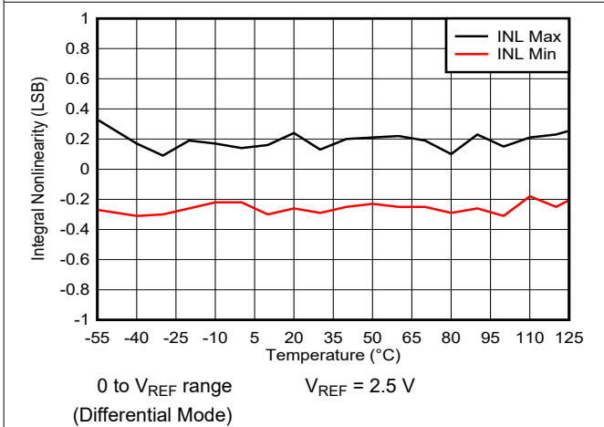
图 6-34. Integral Linearity Error vs Temperature
