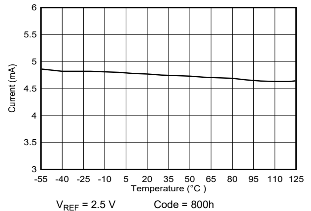
图 6-15. Supply Current vs Temperature
