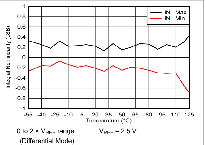
图 6-35. Integral Linearity Error vs Temperature
