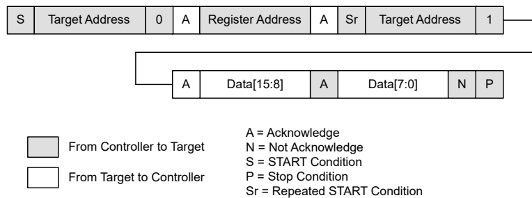
图 7-23. Read A Single Register
