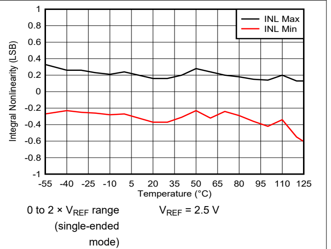
图 6-33. Integral Linearity Error vs Temperature
