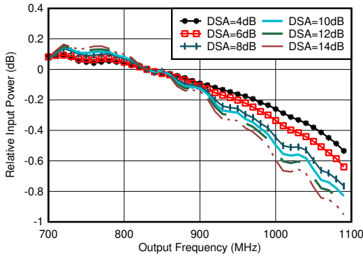
图 6-50. RX In-Band Gain Flatness for Channel 1RX, f_{IN} = 830 MHz
