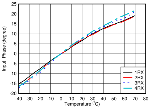
图 6-83. RX Input Phase vs Temperature and DSA at f_{IN} = 1.75 \text{ GHz}
