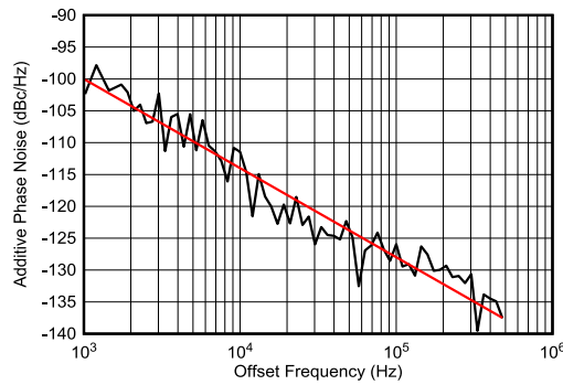
图 6-228. RX Additive Phase Noise at 6.85GHz
