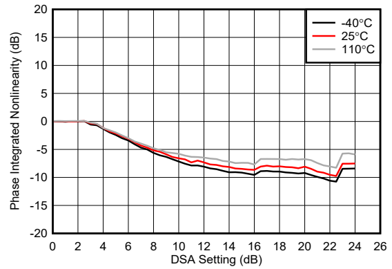
图 6-209. RX Uncalibrated Integrated Phase Error at 6.851GHz
