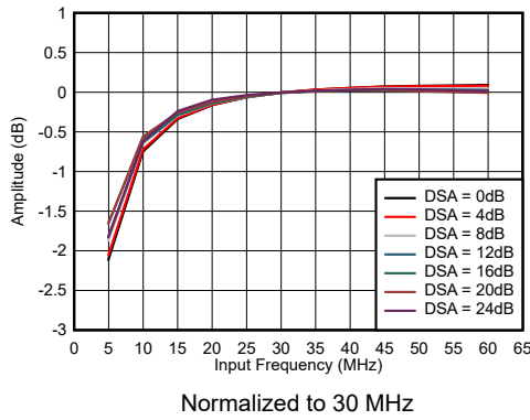
图 6-1. RX In-Band Gain Flatness, f_{IN} = 30 MHz
