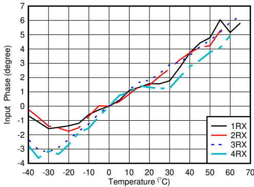
图 6-52. RX Input Phase vs Temperature and DSA at f_{OUT} = 0.8 GHz
