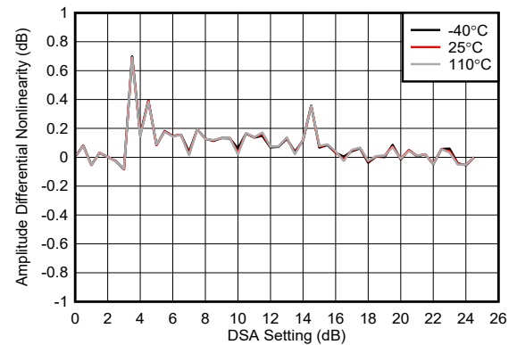
图 6-203. RX Uncalibrated Differential Amplitude Error at 6.851GHz
