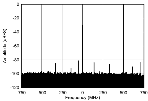
F_{NCO} = 6.851\text{GHz} , F_{IN} offset -130kHz
