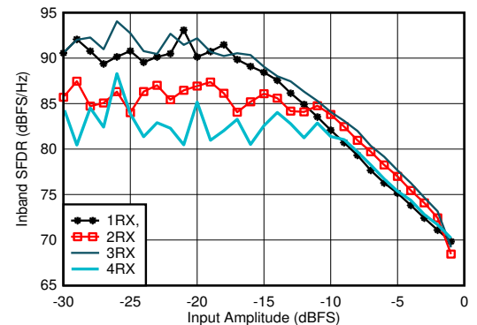
With 1.8 GHz matching, decimated by 3
