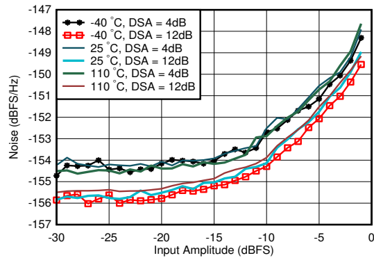
图 6-63. RX Noise Spectral Density vs Input Amplitude and Temperature at 0.8 GHz
