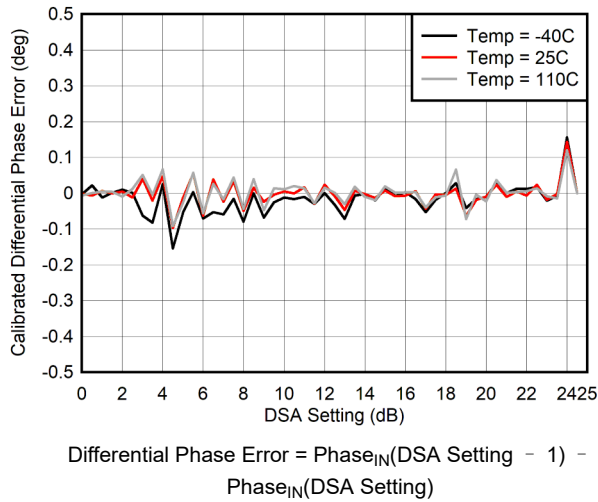
图 6-35. RX Calibrated Differential Phase Error vs DSA Setting at 400 MHz
