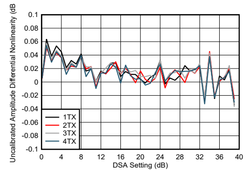
图 4-187. TX DSA Uncalibrated Amplitude Differential Nonlinearity at 8.11GHz
