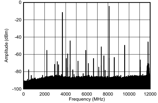
-1dBFS 图 4-203. TX Single Tone Output Spectrum at 8.1GHz
