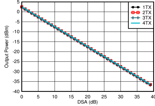
f_{\text{DAC}} = 8847.36\text{MSPS} , A_{\text{out}} = -0.5\text{dBFS} , matching 2.6GHz
