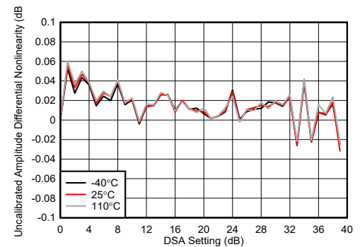
图 4-189. TX DSA Uncalibrated Amplitude Differential Nonlinearity at 8.11GHz
