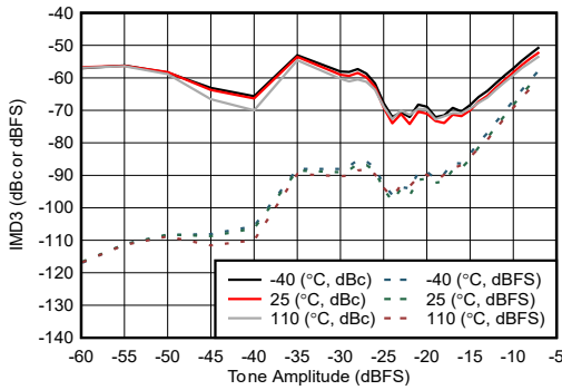
50MHz tone spacing 图 4-253. TX IMD3 vs Digital Amplitude at 9.61GHz
