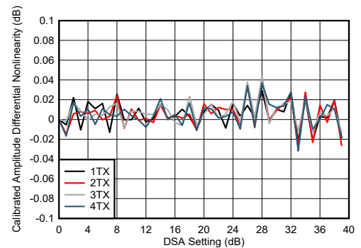
图 4-188. TX DSA Calibrated Amplitude Differential Nonlinearity at 8.11GHz
