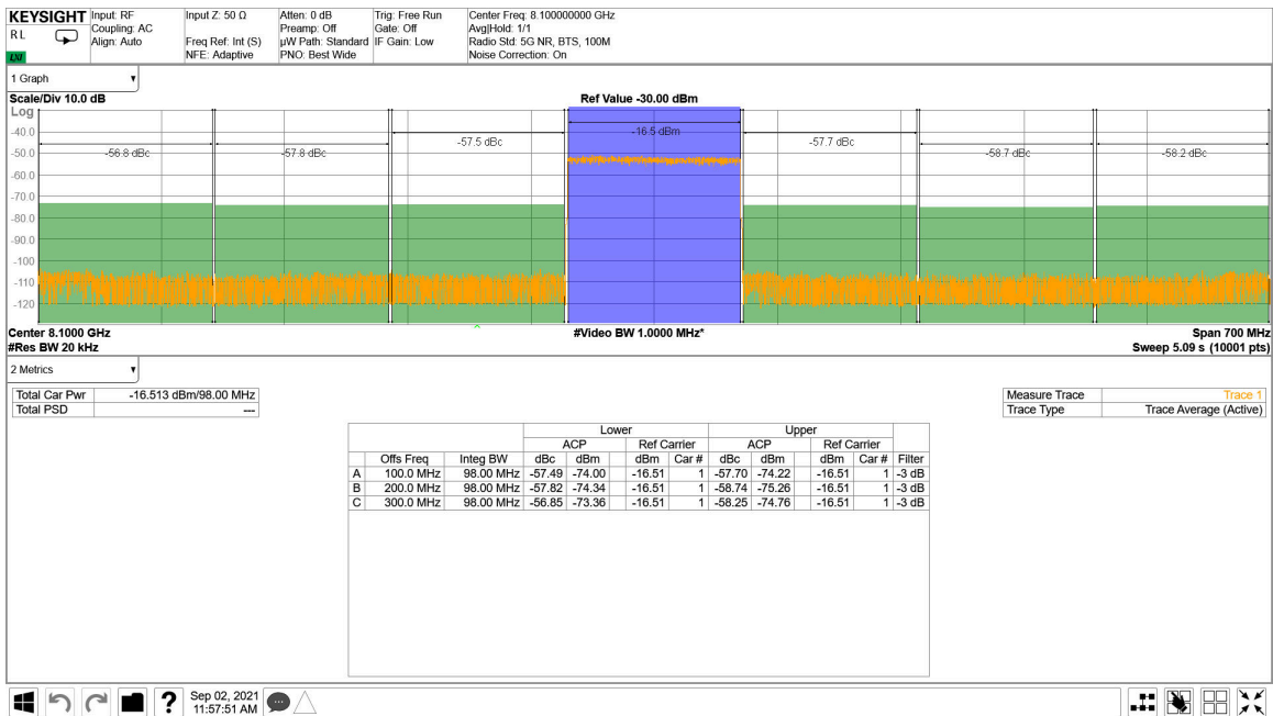
图 4-229. TX 100MHz NR Output Spectrum at 8.11GHz
