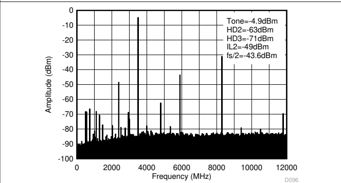
Matching at 3.5GHz, f_{DAC} = 11.79648\text{GSPS} , interleave mode.
