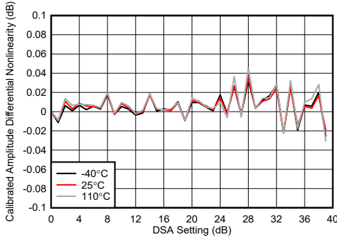
图 4-190. TX DSA Calibrated Amplitude Differential Nonlinearity at 8.11GHz
