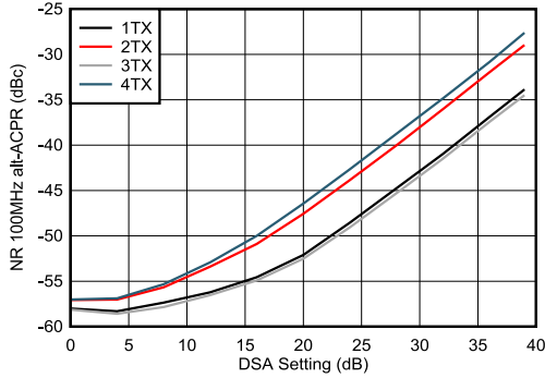
图 4-281. TX NR100MHz ACPR vs DSA Setting at 9.6GHz NR100MHz alt-ACPR vs DSA Setting at 9.6GHz
