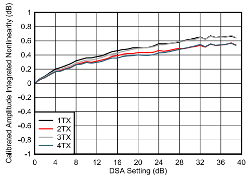
图 4-192. TX DSA Calibrated Amplitude Integrated Nonlinearity at 8.11GHz
