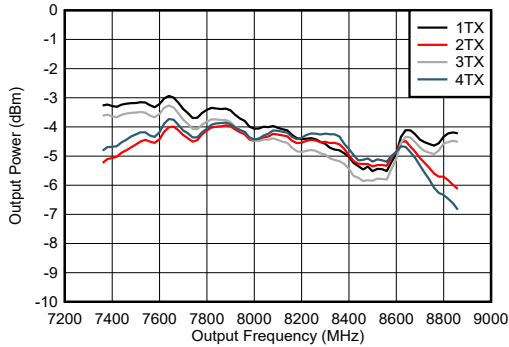
图 4-184. TX Output Power vs Frequency at 8.11GHz
