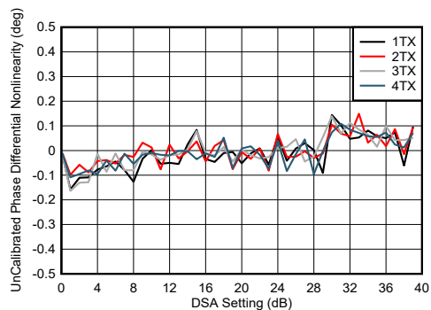
图 4-195. TX DSA Uncalibrated Phase Differential Nonlinearity at 8.11GHz
