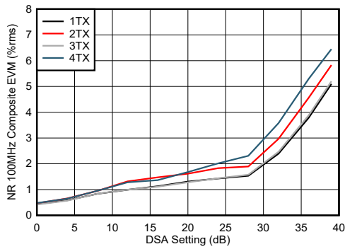
图 4-228. TX NR100MHz EVM vs DSA Setting 8.11GHz
