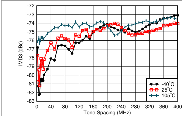
图 4-27. TX IMD3 vs Tone Spacing and Temperature at 0.85GHz
