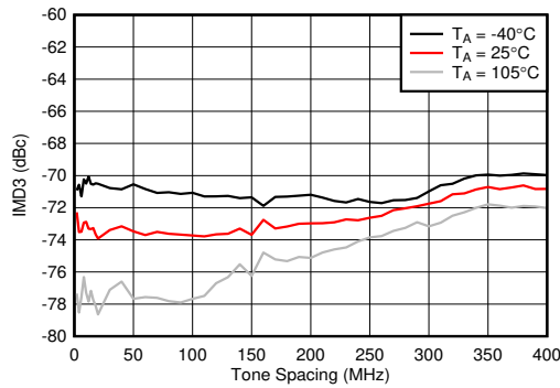
f_{DAC} = 8847.36\text{MSPS} , straight mode, f_{CENTER} = 2.6\text{GHz} , matching at 2.6GHz, -13\text{dBFS} each tone, worst channel.
