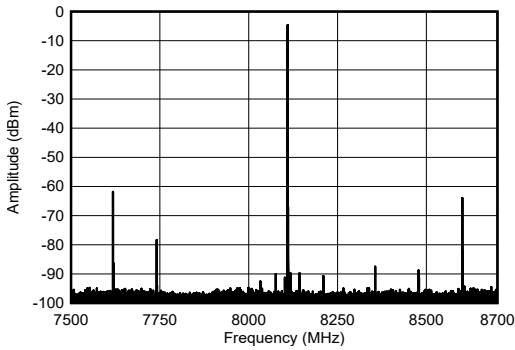
-1dBFS 图 4-204. TX Single Tone Output Spectrum at 8.1GHz
