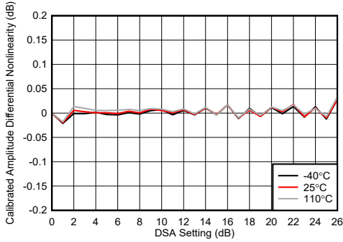
图 4-239. TX DSA Calibrated Amplitude Differential Nonlinearity
