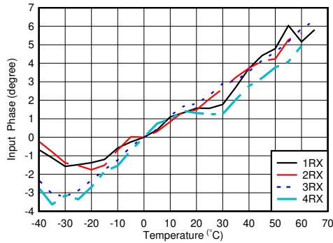
图 4-287. RX Input Phase vs Temperature and DSA at f_{OUT} = 0.8\text{GHz}
