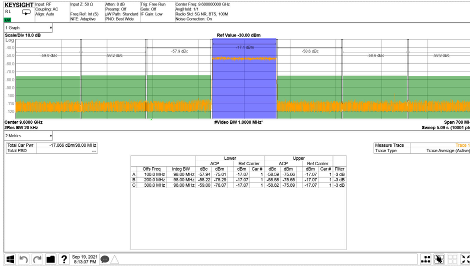
图 4-281. TX NR100MHz ACPR vs DSA Setting at 9.6GHz NR100MHz alt-ACPR vs DSA Setting at 9.6GHz
