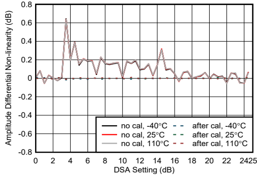
图 4-451. RX Amplitude Differential Non-linearity at 9.6GHz
