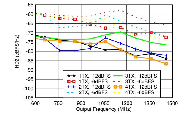
Matching at 0.8GHz, f_{DAC} = 8847.36\text{GSPS} , straight mode
