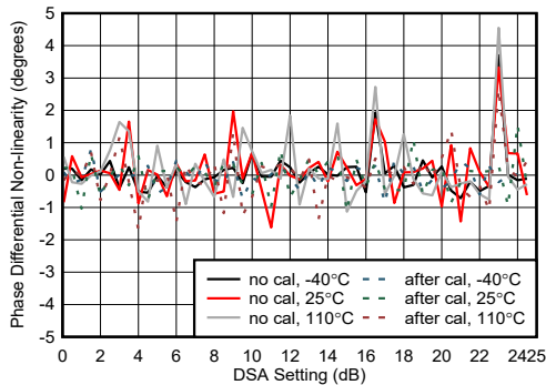
图 4-453. RX Phase Differential Non-linearity at 9.6GHz
