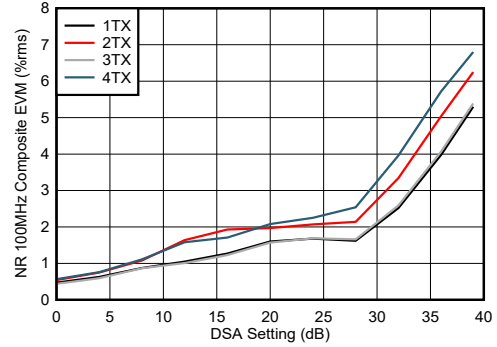
图 4-282. TX NR100MHz EVM vs DSA Setting at 9.6GHz
