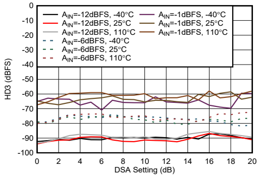
图 4-465. RX HD3 vs DSA Setting at 9.6GHz
