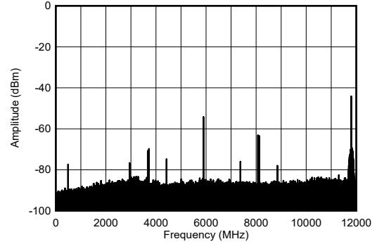
50MHz tone spacing, -60dBFS each tone
