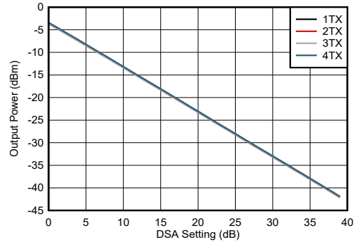
图 4-185. TX Output Power vs DSA Setting at 8.11GHz
