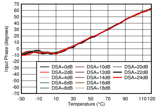
With 3.6GHz matching, normalized to phase at 25°C
