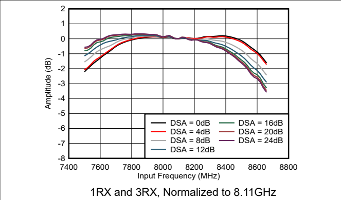
图 4-423. RX Amplitude vs Frequency and DSA Setting
