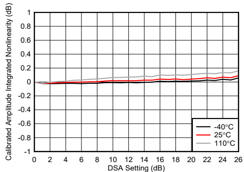
图 4-243. TX DSA Calibrated Amplitude Integrated Nonlinearity
