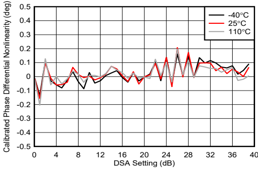
图 4-198. TX DSA Calibrated Phase Differential Nonlinearity at 8.1GHz
