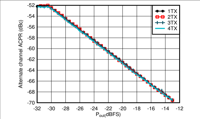
Matching at 0.8GHz, single carrier 20MHz BW TM1.1 LTE
