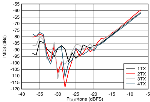
f_{DAC} = 8847.36\text{MSPS} , straight mode, f_{CENTER} = 2.6\text{GHz} , f_{SPACING} = 20\text{MHz} , matching at 2.6GHz
