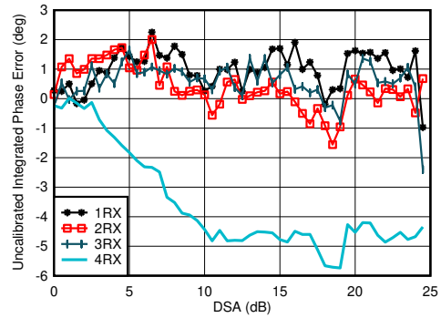
图 4-400. RX Uncalibrated Differential Phase Error vs DSA Setting at 4.9GHz
