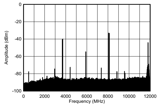
图 4-211. TX Dual Tone Output Spectrum at 8.11GHz
