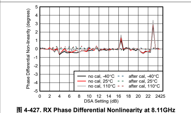
图 4-427. RX Phase Differential Nonlinearity at 8.11GHz
