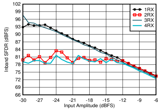
图 4-418. RX In-Band SFDR ( \pm 400 MHz) vs Input Amplitude and Channel at 4.9GHz
