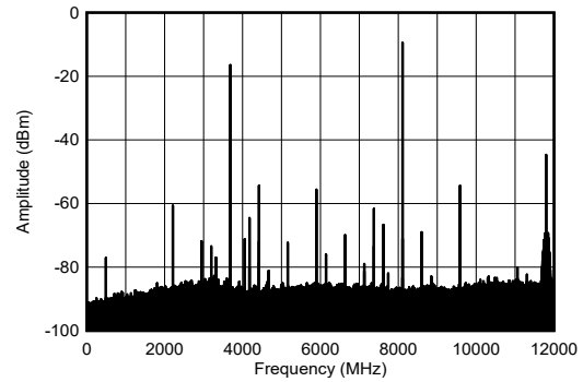
-6dBFS 图 4-205. TX Single Tone Output Spectrum at 8.1GHz
