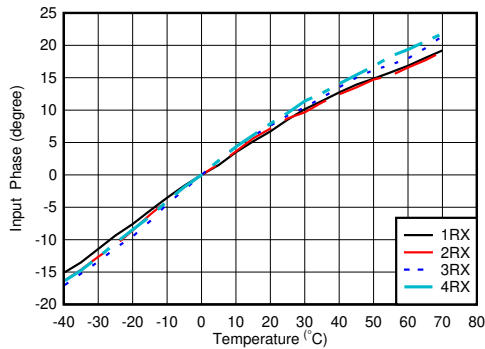
图 4-318. RX Input Phase vs Temperature and DSA at f_{IN} = 1.75\text{GHz}
