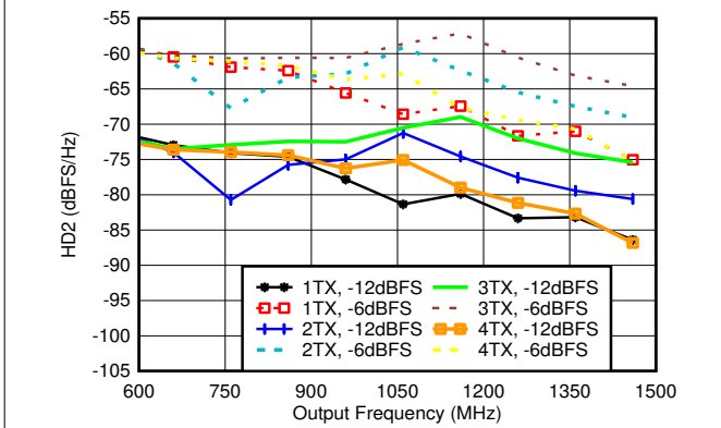
Matching at 0.8GHz, f_{DAC} = 5898.2\text{ GSPS} , straight mode
