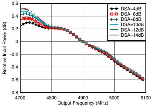
图 4-393. RX Inband Gain Flatness, f_{IN} = 4900\text{MHz}
