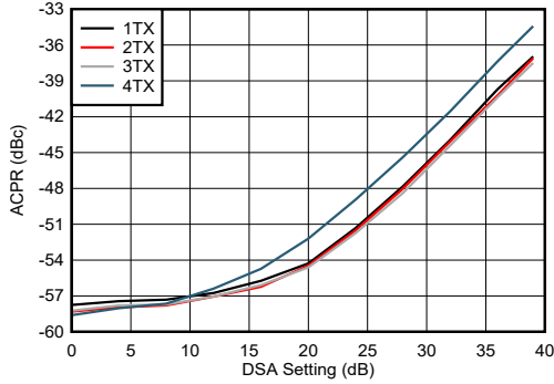
图 4-226. TX NR100MHz ACPR vs DSA Setting 8.11GHz
