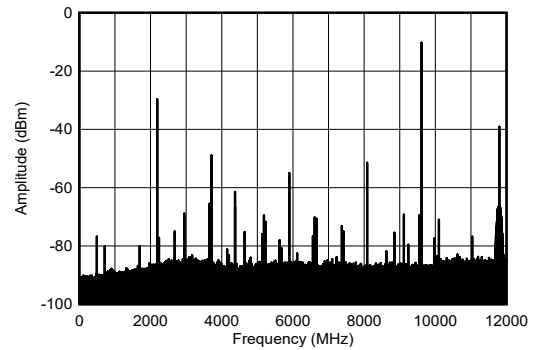
图 4-266. TX Single Tone Spectrum at 9.61GHz and -1dBFS (wideband)
