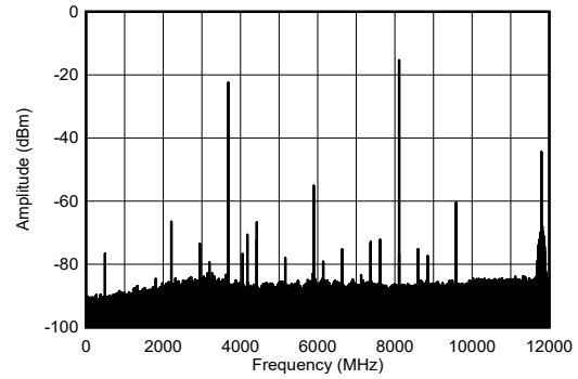
-12dBFS 图 4-207. TX Single Tone Output Spectrum at 8.1GHz
