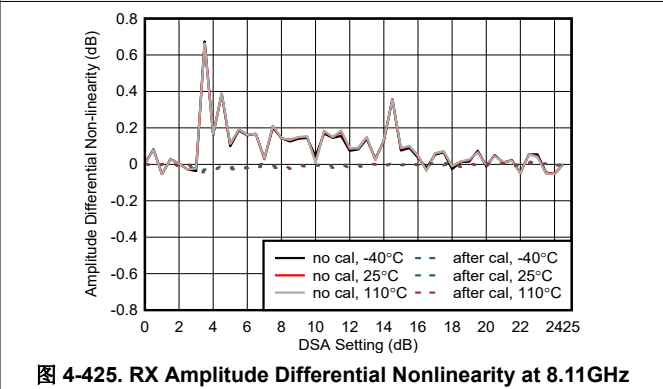
图 4-425. RX Amplitude Differential Nonlinearity at 8.11GHz
