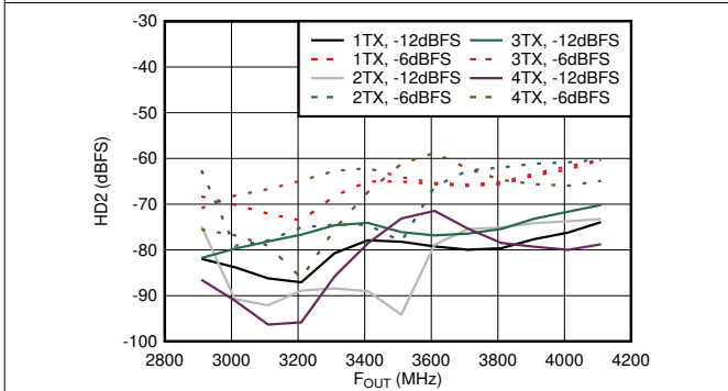
Matching at 3.5GHz, f_{DAC} = 11.79648\text{GSPS} , interleave mode, normalized to output power at harmonic frequency
