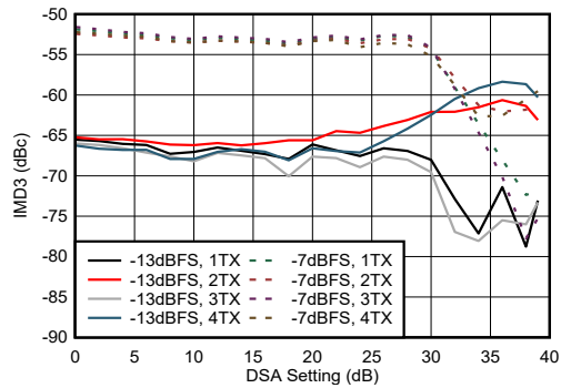
50MHz tone spacing 图 4-255. TX IMD3 vs DSA Setting at 9.61GHz
