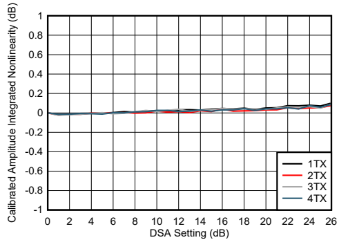
图 4-241. TX DSA Calibrated Amplitude Integrated Nonlinearity
