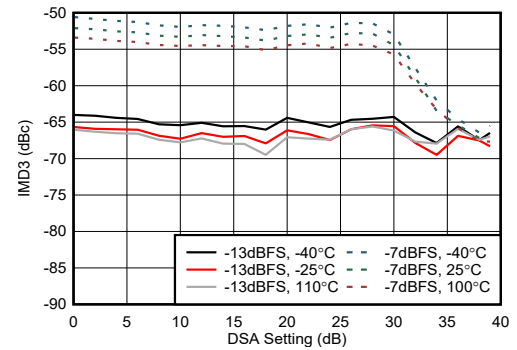
50MHz tone spacing 图 4-256. TX IMD3 vs DSA Setting at 9.61GHz
