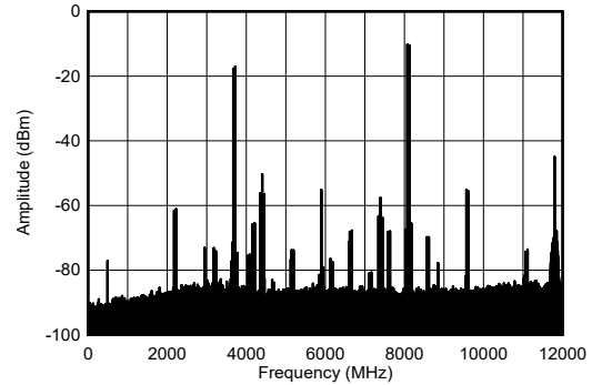
图 4-209. TX Dual Tone Output Spectrum at 8.11GHz
