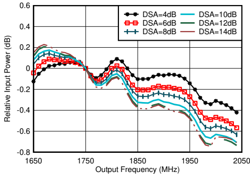
图 4-316. RX In-Band Gain Flatness, f_{IN} = 1750\text{MHz}
