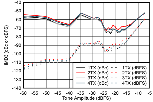
50MHz tone spacing 图 4-252. TX IMD3 vs Digital Amplitude at 9.61GHz
