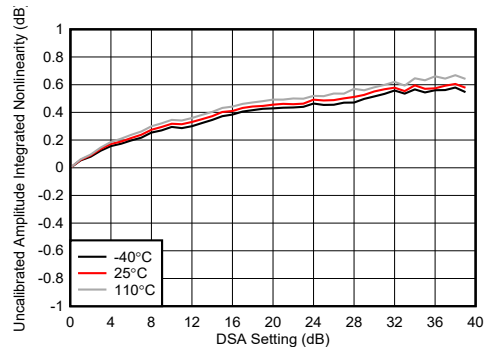
图 4-193. TX DSA Uncalibrated Amplitude Integrated Nonlinearity at 8.11GHz
