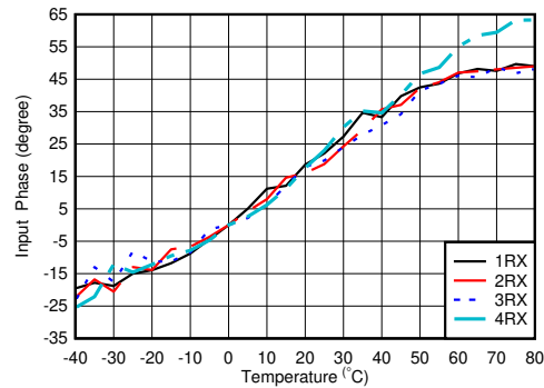
图 4-395. RX Input Phase vs Temperature and DSA at f_{OUT} = 4.9\text{GHz}
