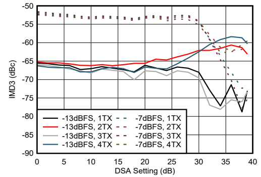
50MHz tone spacing 图 4-254. TX IMD3 vs DSA Setting at 9.61GHz
