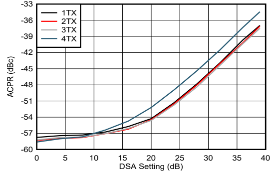
图 4-227. TX NR100MHz alt-ACPR vs DSA Setting 8.11GHz
