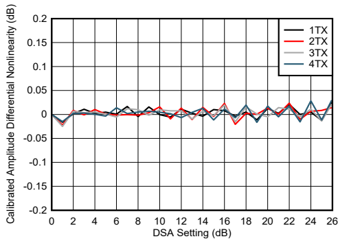
图 4-237. TX DSA Calibrated Amplitude Differential Nonlinearity
