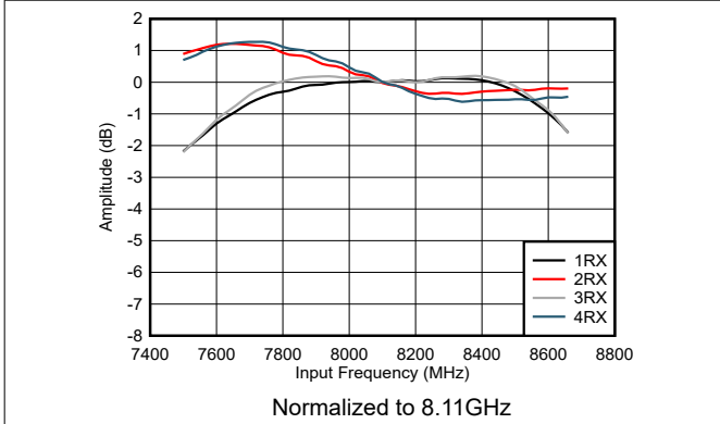
图 4-422. RX Amplitude vs Frequency and Channel
