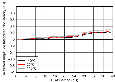
图 4-194. TX DSA Calibrated Amplitude Integrated Nonlinearity at 8.11GHz
