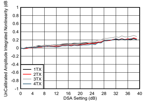
图 4-191. TX DSA Uncalibrated Amplitude Integrated Nonlinearity at 8.11GHz
