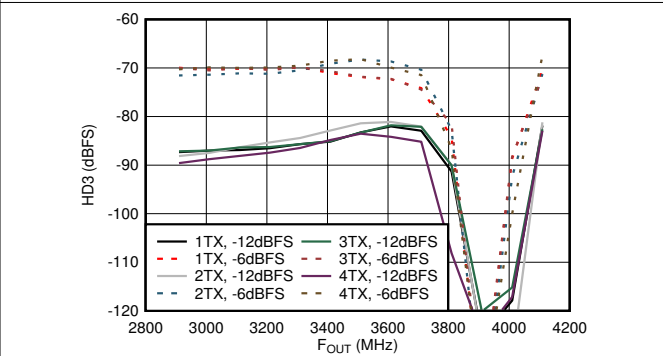
Matching at 3.5GHz, f_{DAC} = 11.79648\text{GSPS} , interleave mode, normalized to output power at harmonic frequency. Dip is due to HD3 falling near DC.
