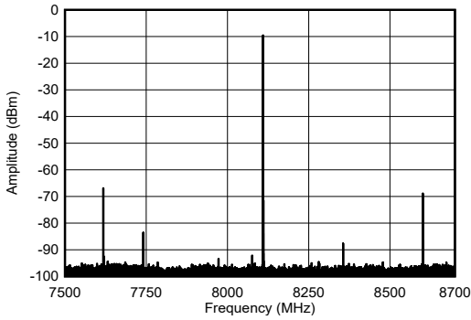
-6dBFS 图 4-206. TX Single Tone Output Spectrum at 8.1GHz
