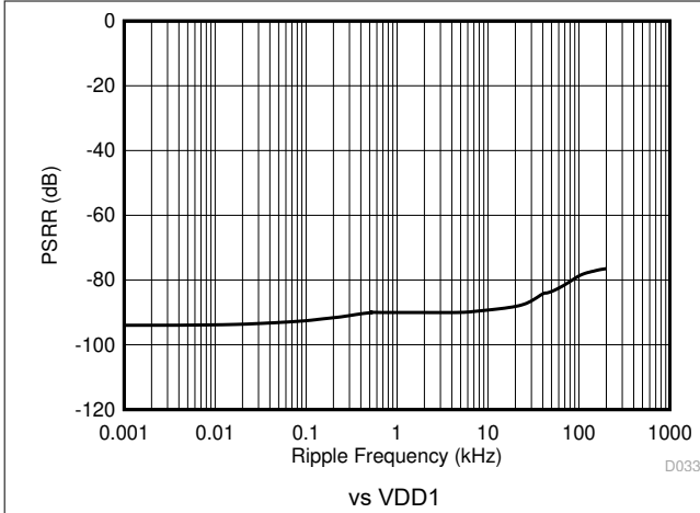
图 6-35. Power-Supply Rejection Ratio vs Ripple Frequency
