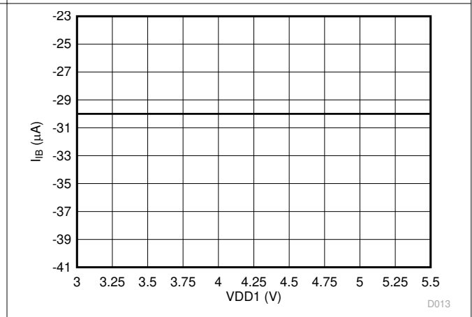
图 6-16. Input Bias Current vs High-Side Supply Voltage
