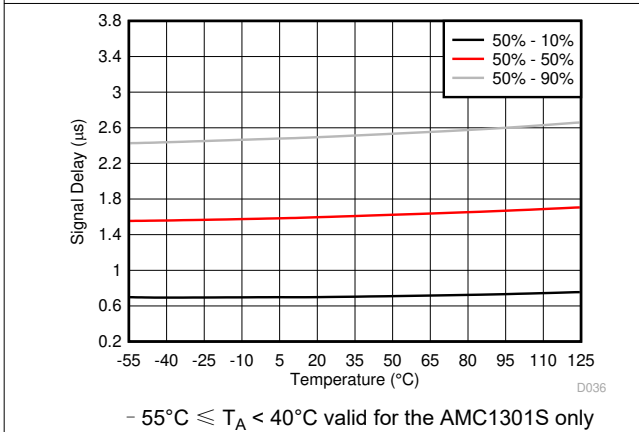
图 6-39. V IN to V OUT Signal Delay vs Temperature
