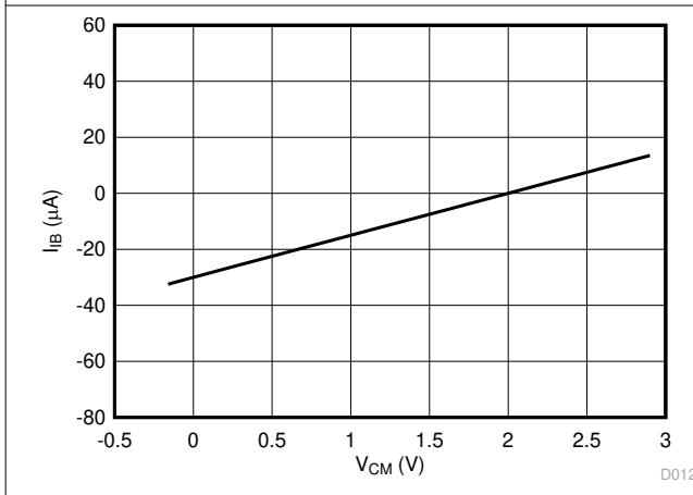
图 6-15. Input Bias Current vs Common-Mode Input Voltage
