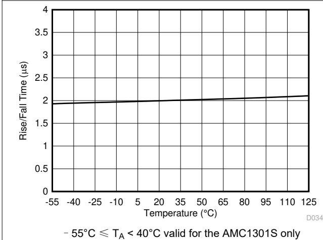
图 6-37. Output Rise and Fall Time vs Temperature
