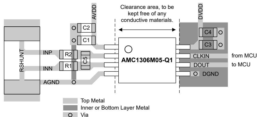
图 10-1. Recommended Layout of the AMC1306M05-Q1
