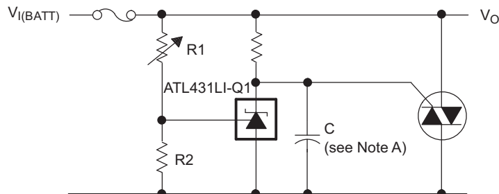
图 34. Crowbar Circuit
