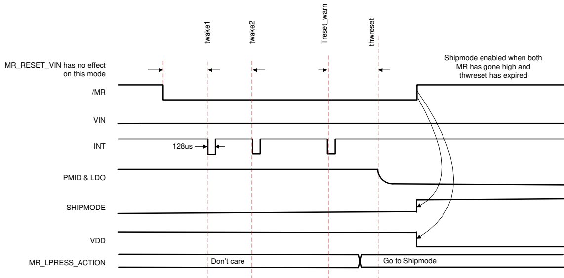
图 7-6. MR Wake and Reset Timing Active Mode When MR_LPRESS_ACTION = 1x (Ship Mode) and Only BAT is Present
