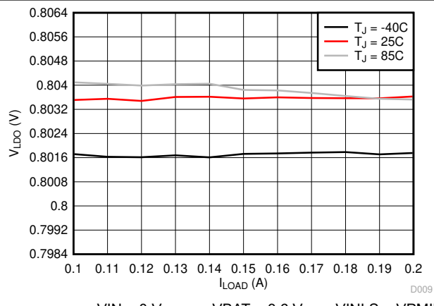
图 6-6. LDO Load Regulation (VLDO = 0.8 V)
