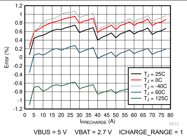
图 6-4. Pre-Charge Current Accuracy vs. IPRECHARGE Setting (ICHARGE_RANGE = 1)
