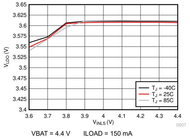
图 6-12. LDO Line Regulation (VLDO = 3.6 V)
