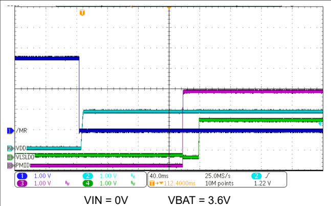
图 8-5. Power Up from Ship Mode with MR Press
