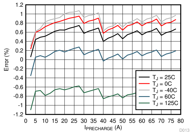
图 6-4. Pre-Charge Current Accuracy vs. IPRECHARGE Setting (ICHARGE_RANGE = 1)
