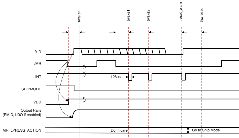
图 7-4. MR Wake from Ship Mode - VIN Dependencies
