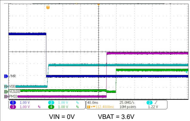
图 8-5. Power Up from Ship Mode with \overline{MR} Press
