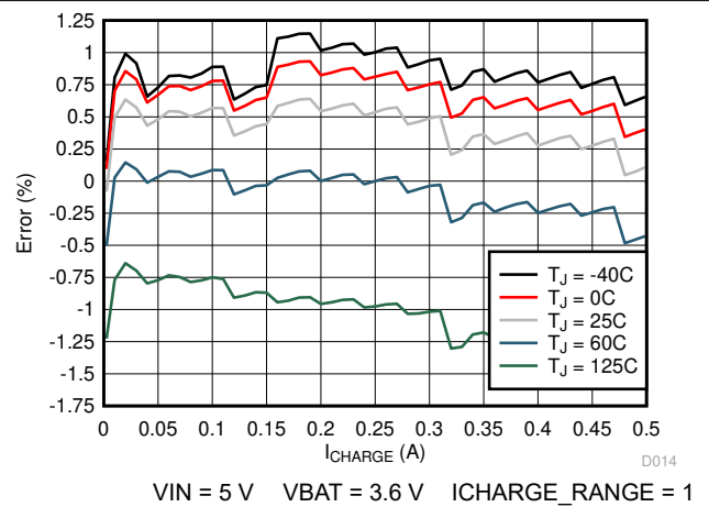
图 6-2. Charge Current Accuracy vs. ICHARGE Setting
