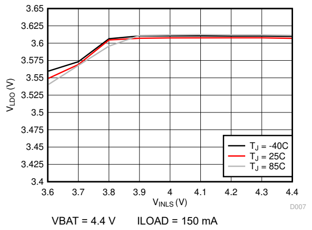
图 6-12. LDO Line Regulation (VLDO = 3.6 V)
