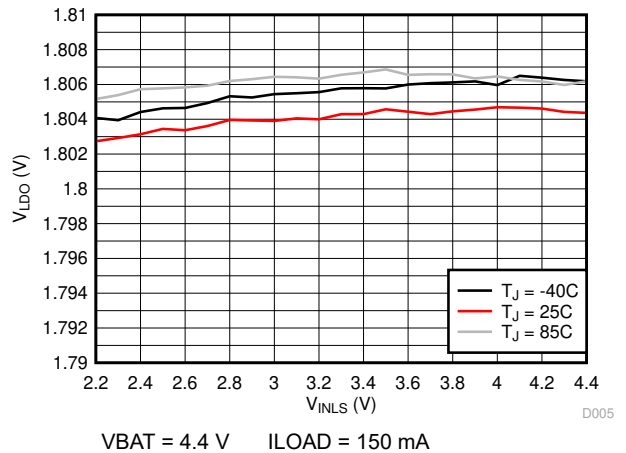
图 6-10. LDO Line Regulation (VLDO = 1.8 V)
