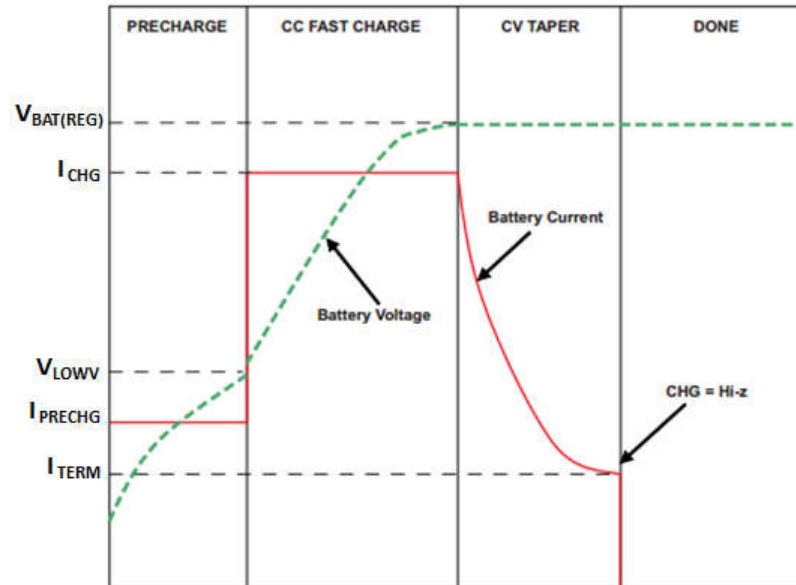
图 7-2. BQ21061 Typical Charge Cycle
