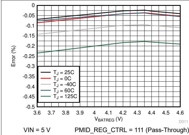
图 6-1. Battery Regulation Voltage Accuracy vs. VBATREG Setting
