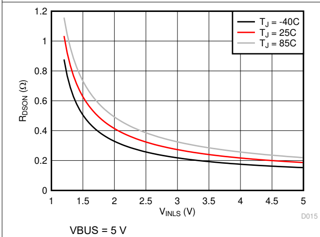
图 6-5. LS/LDO Switch On Resistance vs. VINLS
