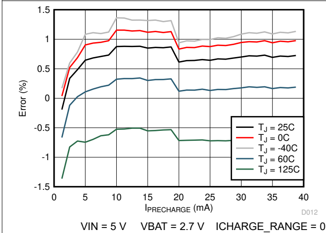
图 6-3. Pre-Charge Current Accuracy vs. IPRECHARGE setting (ICHARGE_RANGE = 0)
