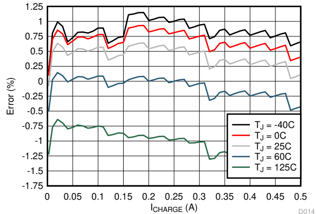
图 6-2. Charge Current Accuracy vs. ICHARGE Setting
