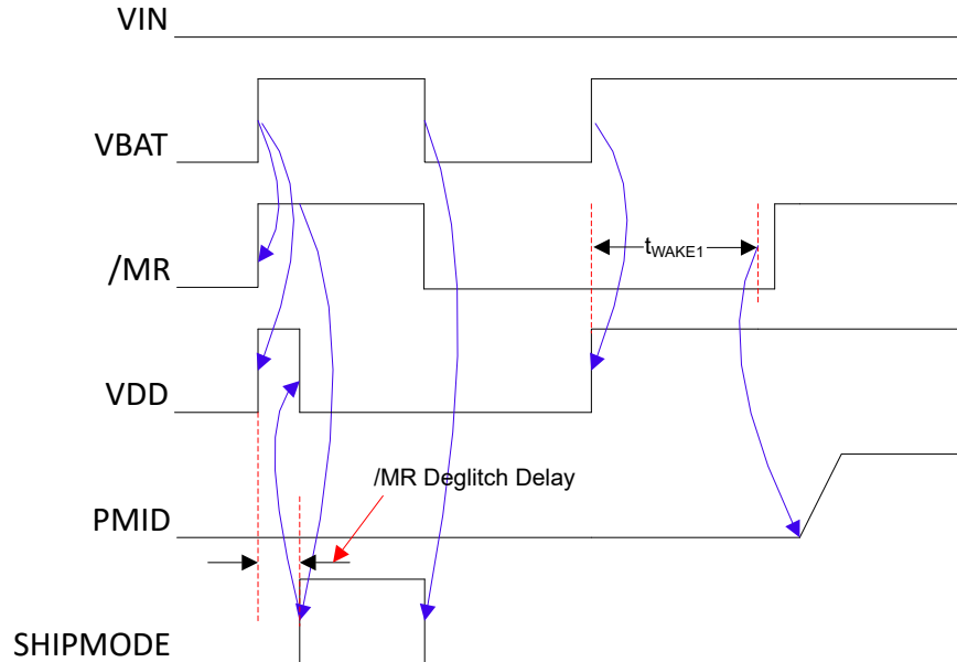
图 7-15. BQ21061 Wake-Up Upon Battery Insertion
