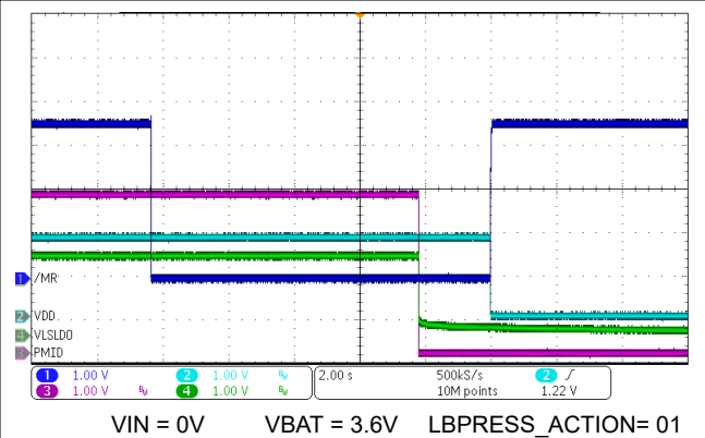
图 8-7. Ship Mode Entry with MR Long Button Press
