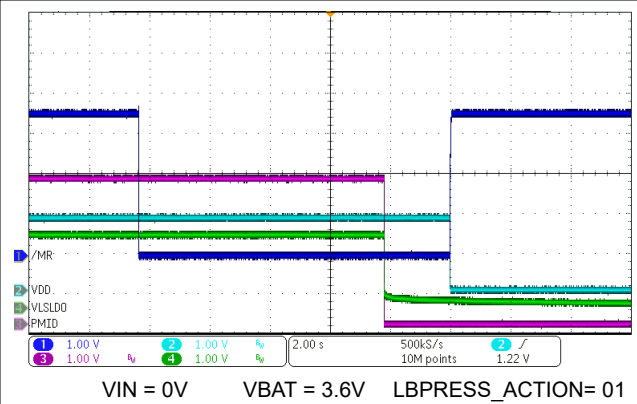
图 8-7. Ship Mode Entry with \overline{MR} Long Button Press
