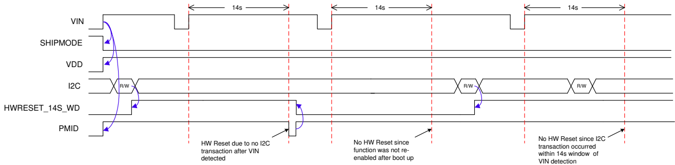
图 7-7. 14-Second Watchdog for HW Reset Behavior
