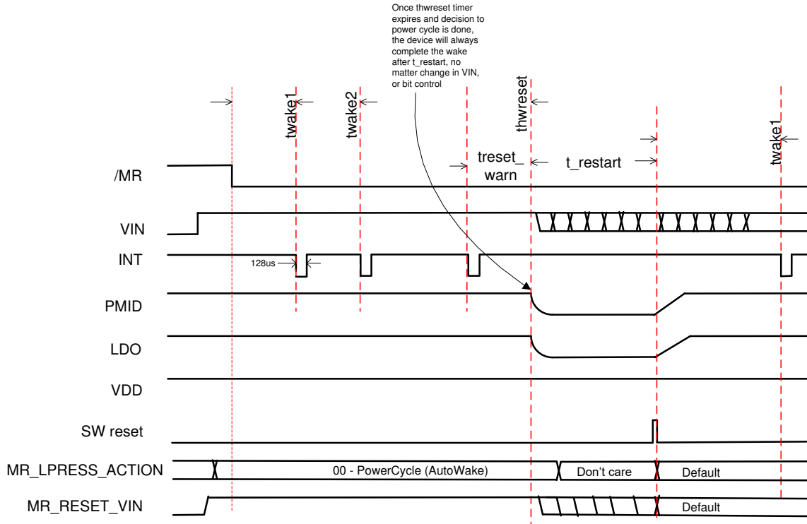
图 7-5. MR Wake and Reset Timing with VIN Present or BAT Active Mode When MR_LPRESS_ACTION = 00
