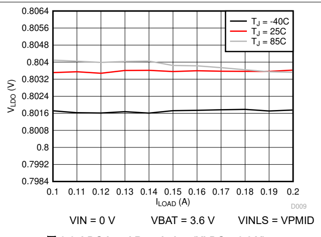
图 6-6. LDO Load Regulation (VLDO = 0.8 V)
