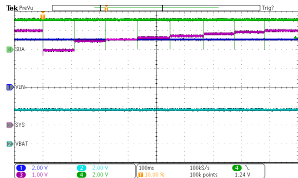
SYS_REG_CTRL = 000 → 111 (步进)
